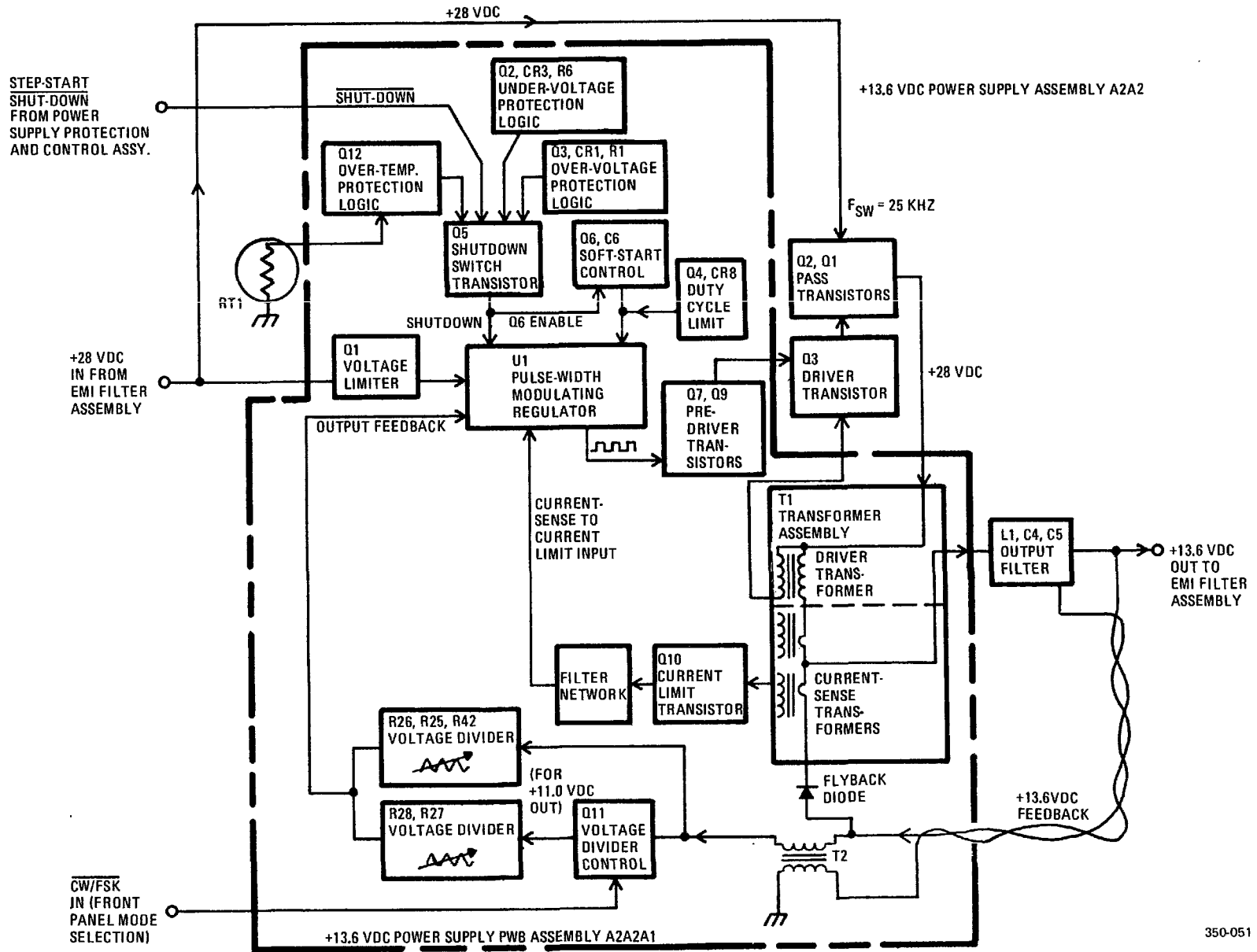
Figure 5-36. +13.6 Vdc Power Supply Functional Diagram
