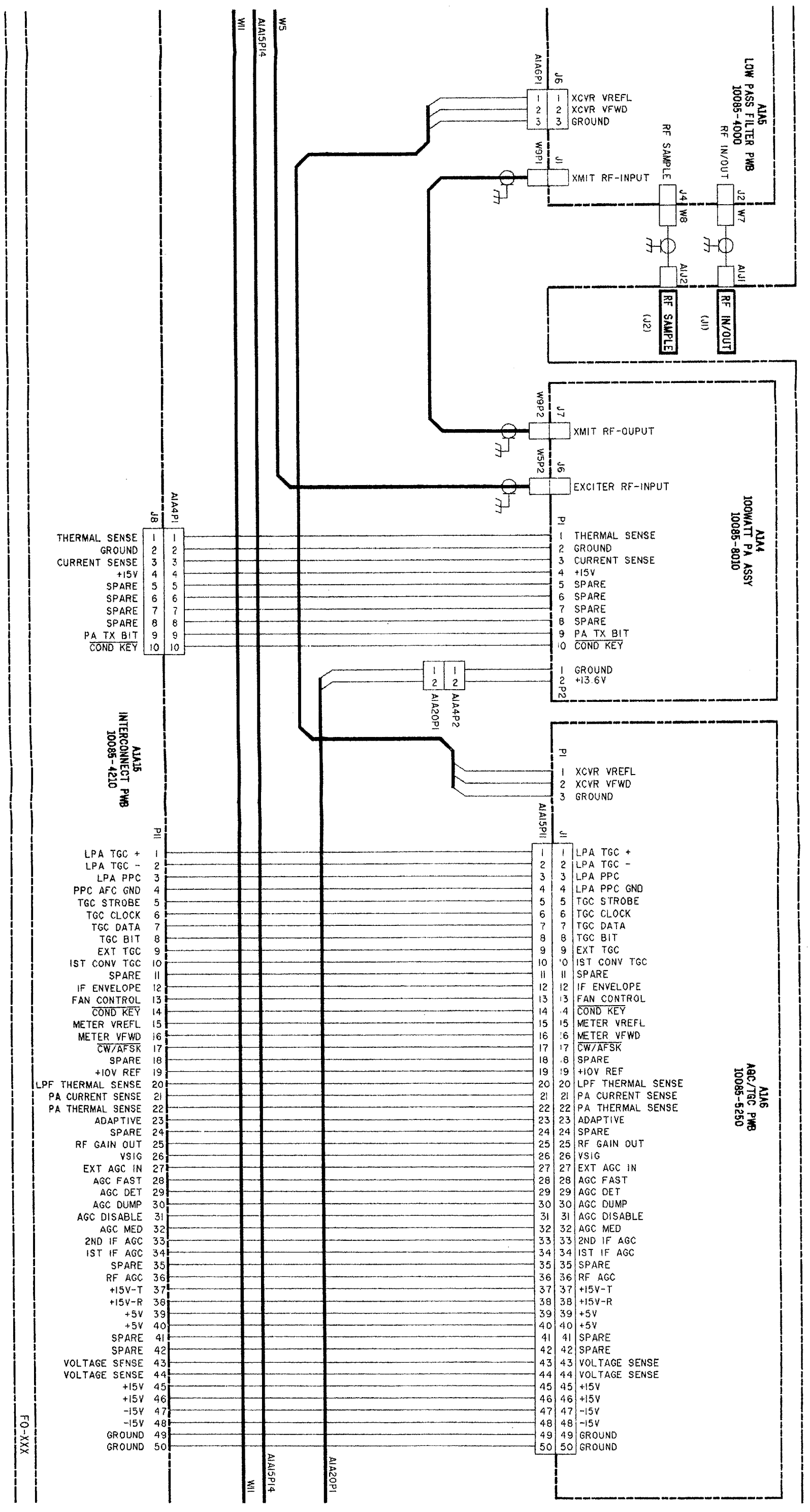
Figure FO-11. Interconnection Diagram. (Sheet 10 of 13)
