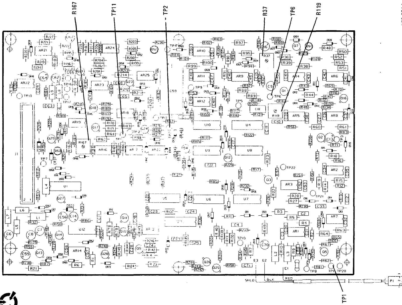
Figure 6-8. AGC/ITC PWB Assy.
