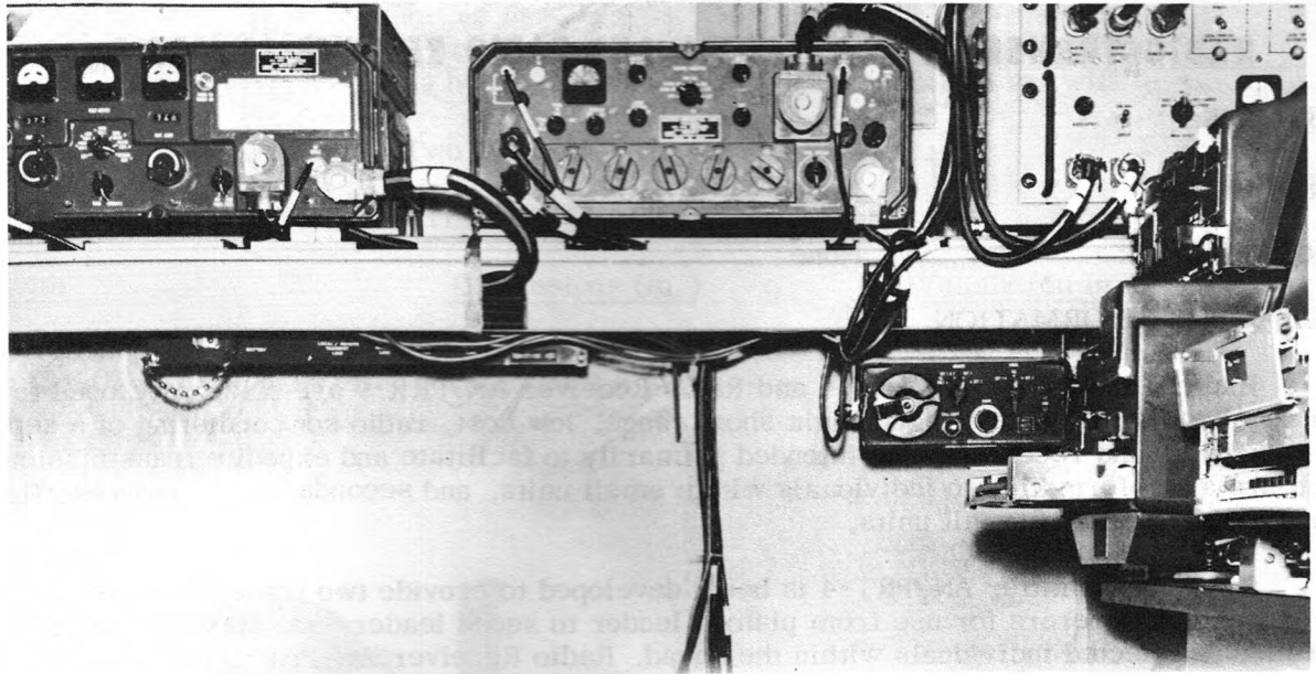
Figure 95. Radio Teletypewriter Set AN/GRC-142, forward view, upper half.
