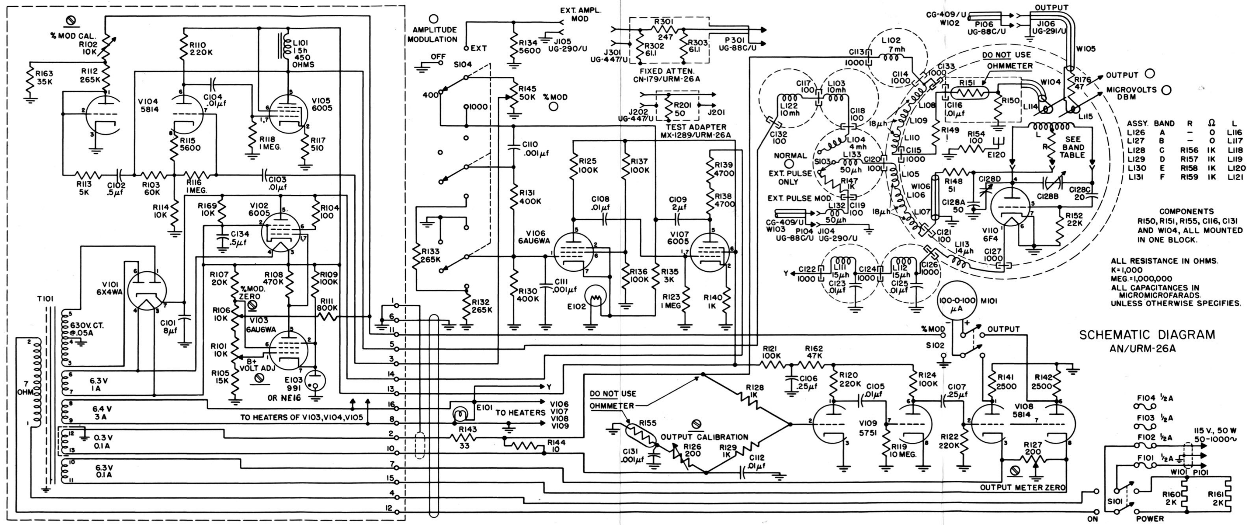
Figure 7-21. RF Signal Generator Set AN/URM-26A, Schematic Diagram
