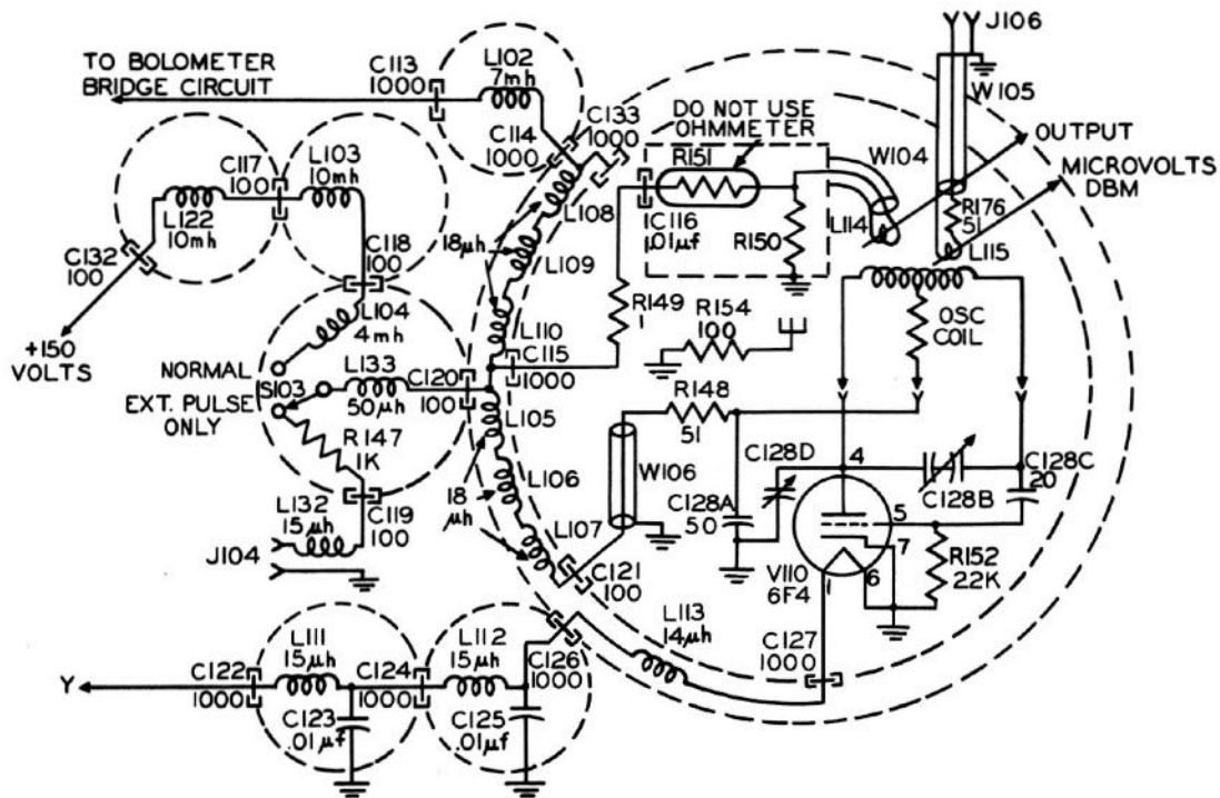
Figure 2-4. RF Signal Generator SG-45A/URM-26, Functional Schematic Diagram, RF Oscillator
