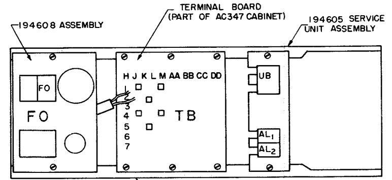
TOP VIEW OF CABINET MTG. LOCATION
