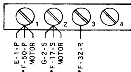
S 151415 MOTOR TERMINAL BLOCK
