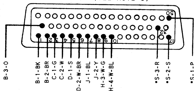
F 192013 KEYBOARD CONNECTOR (SEE NOTE 3)
