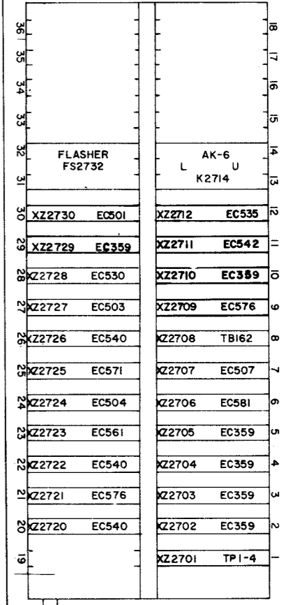
MODULE LAYOUT VIEW FROM WIRE SIDE 193240
