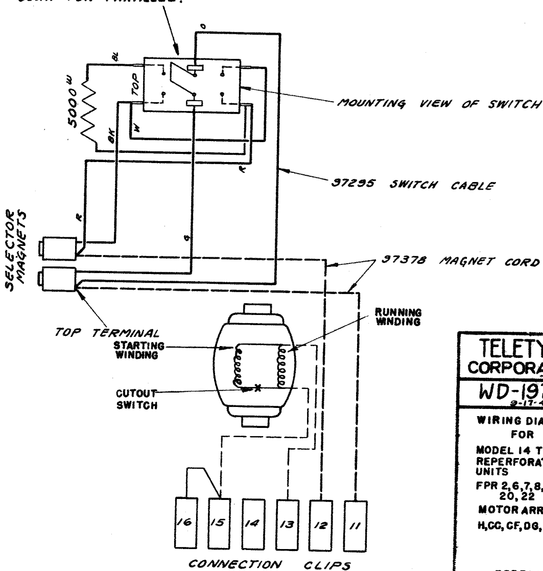
A.C. RECEIVING UNIT WITH SYNCHRONOUS MOTOR
