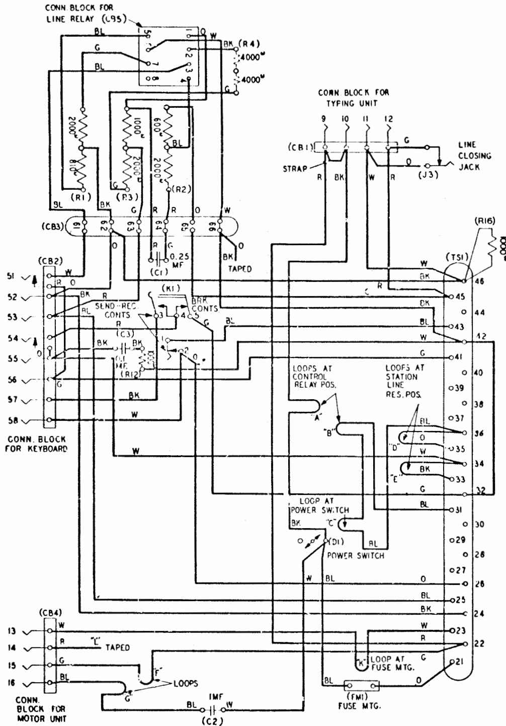
Figure 4 - 15D Teletypewriter Base
