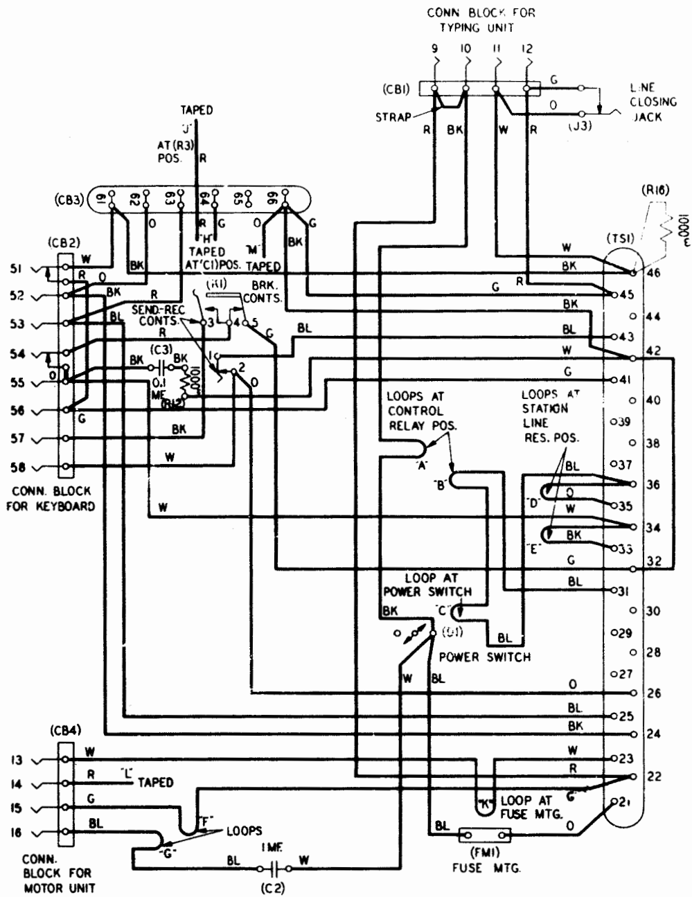
Figure 3 — 15C Teletypewriter Base
