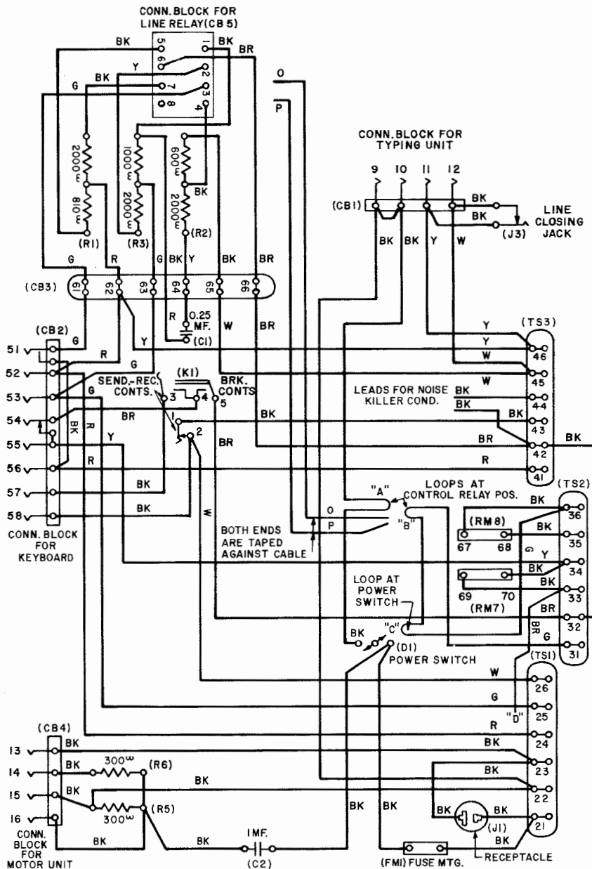
Figure 1 - 15A Teletypewriter Base
