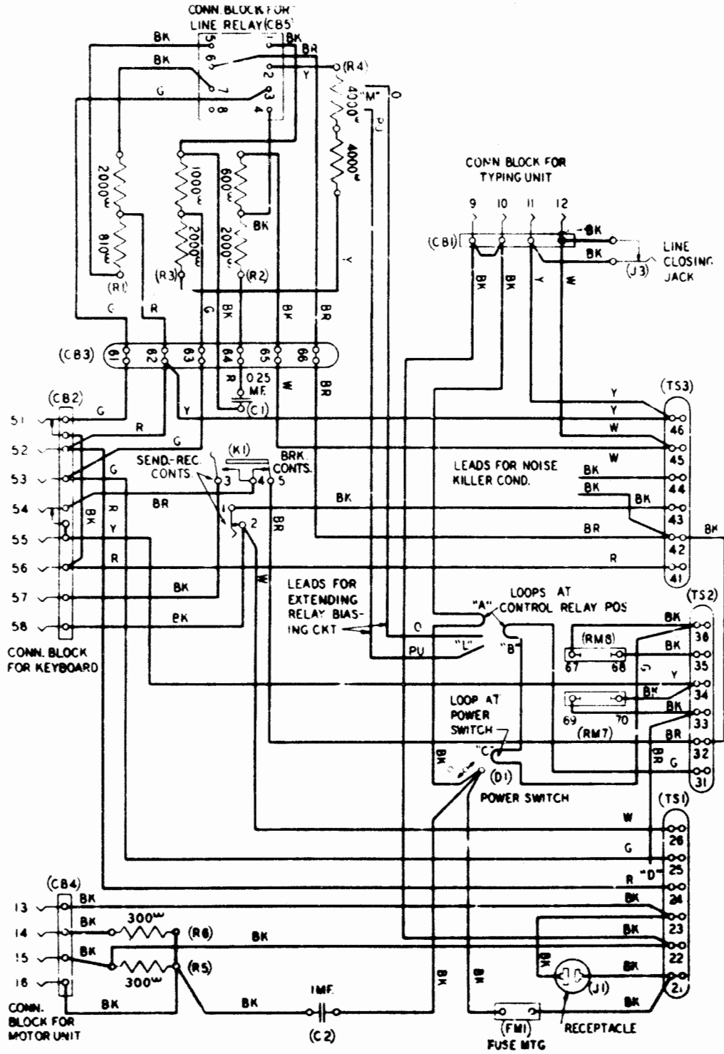
Figure 2 — 15B Teletypewriter Base
