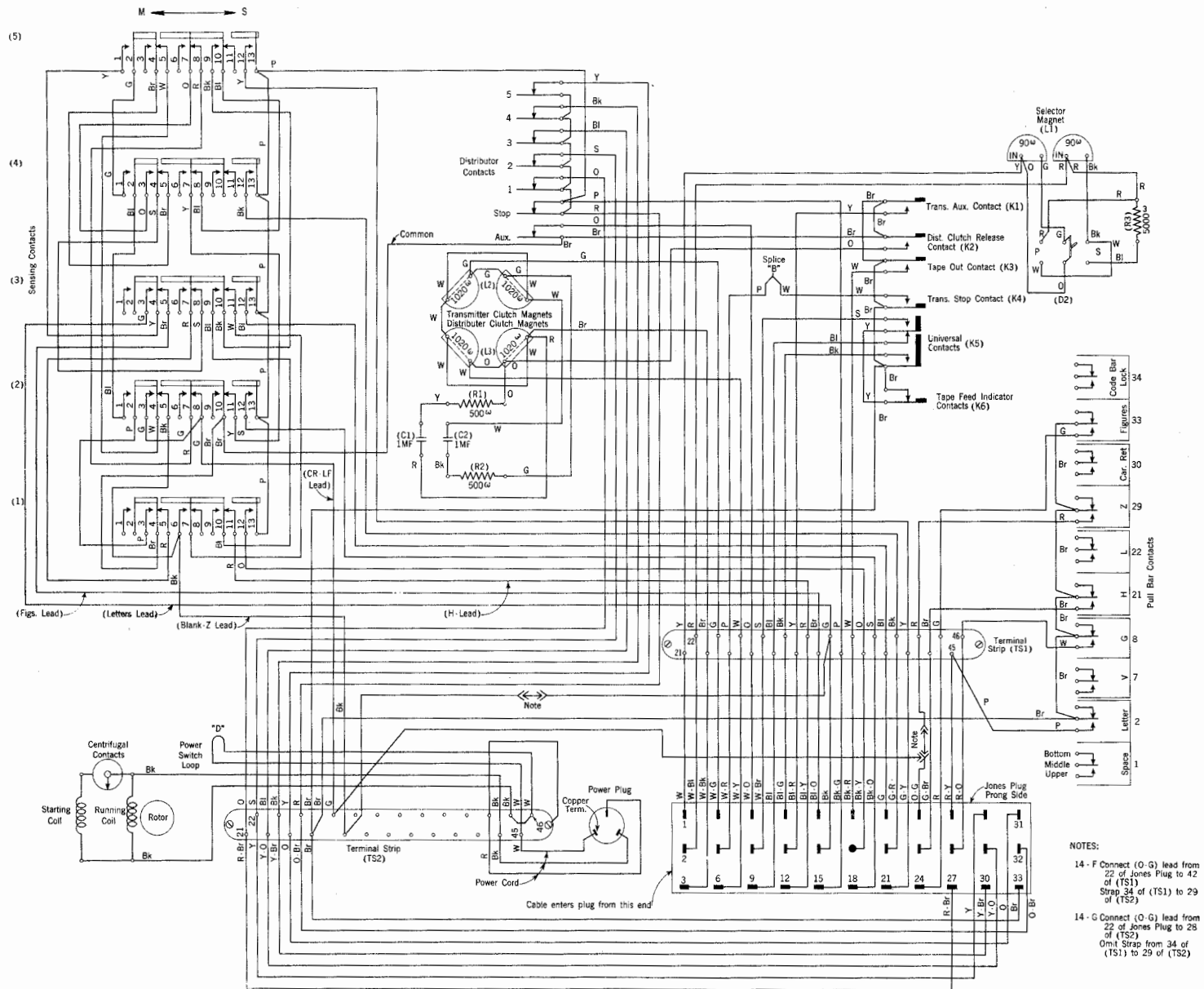
Figure 1 - 14F, 14F-1, 14F-2, 14F-3, 14G, 14G-1, 14G-2, and 14G-3 - Reperforator-Transmitter Units
