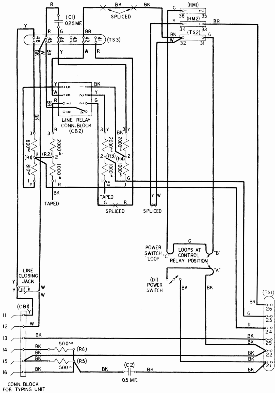
Figure 1 - 14A and 14S Teletypewriter Bases and 14N Typing Reperforator Base
