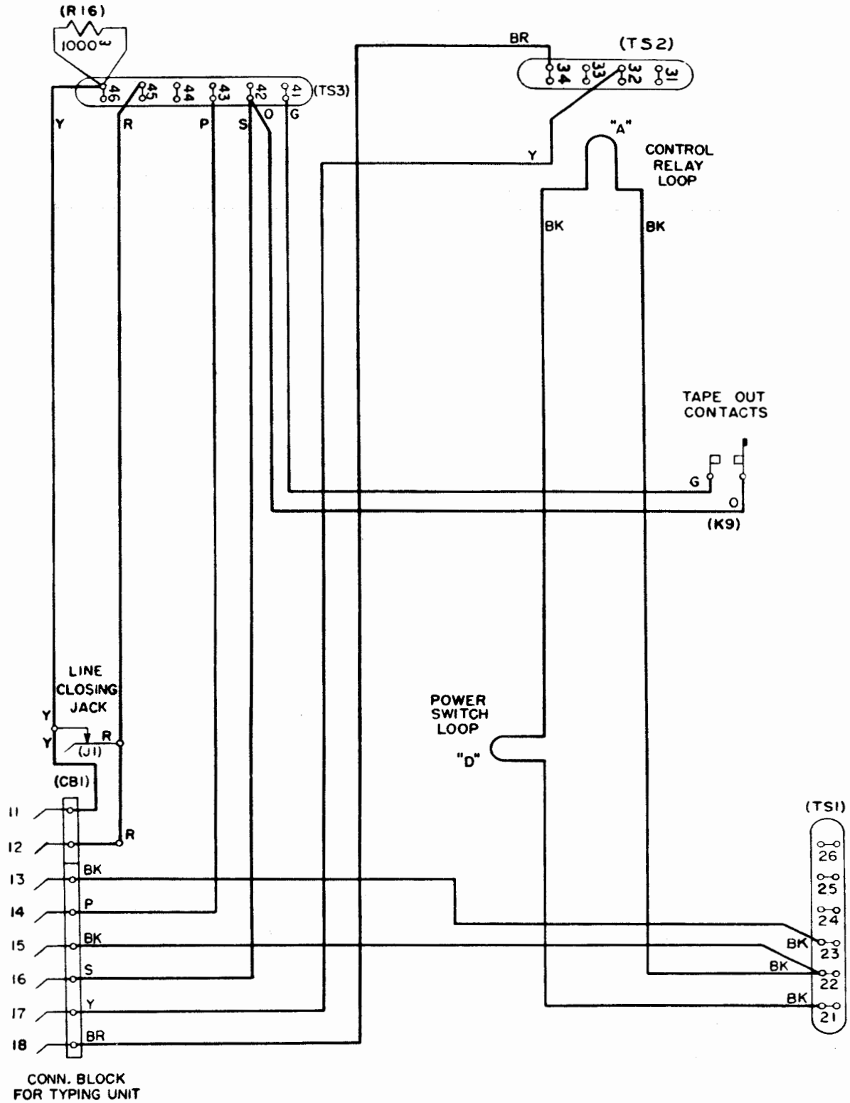
Figure 4 - 14AD and 14AE Typing Reperforator Bases
