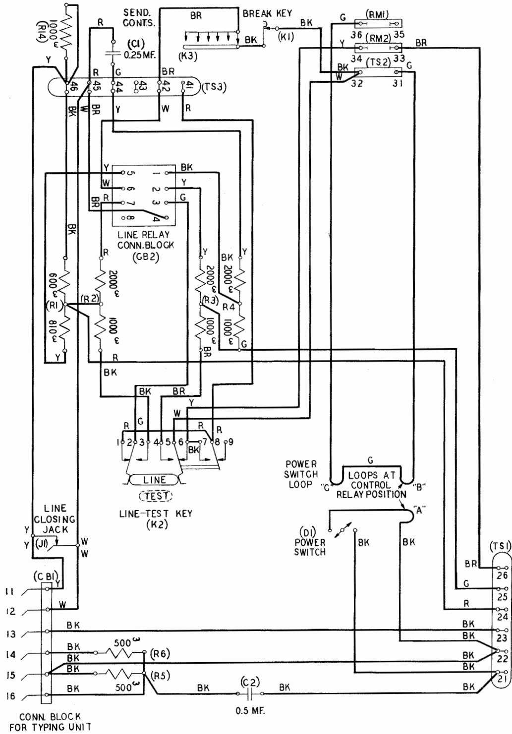
Figure 1 — 14M, 14U, 14W, 14Y, and 14AA Typing Reperforator Bases
