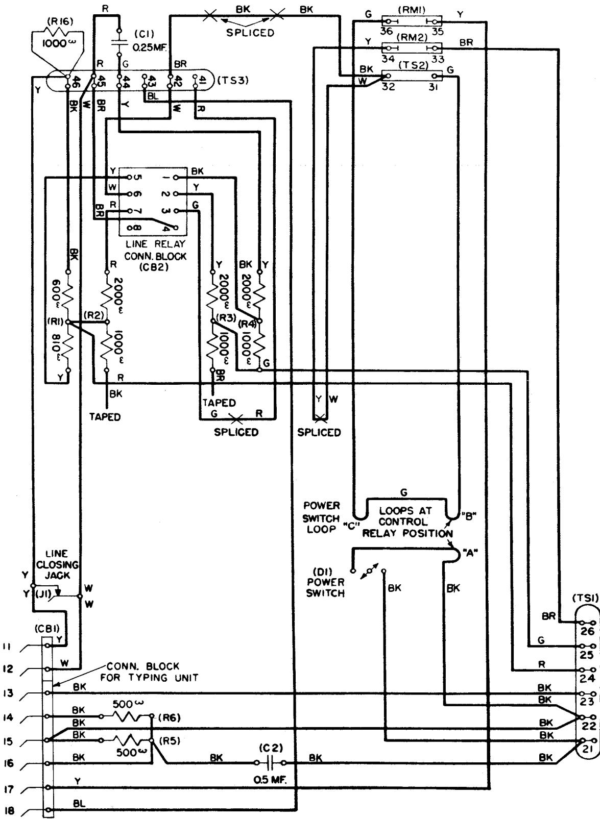
Figure 2 - 14P Typing Reperforator Base
