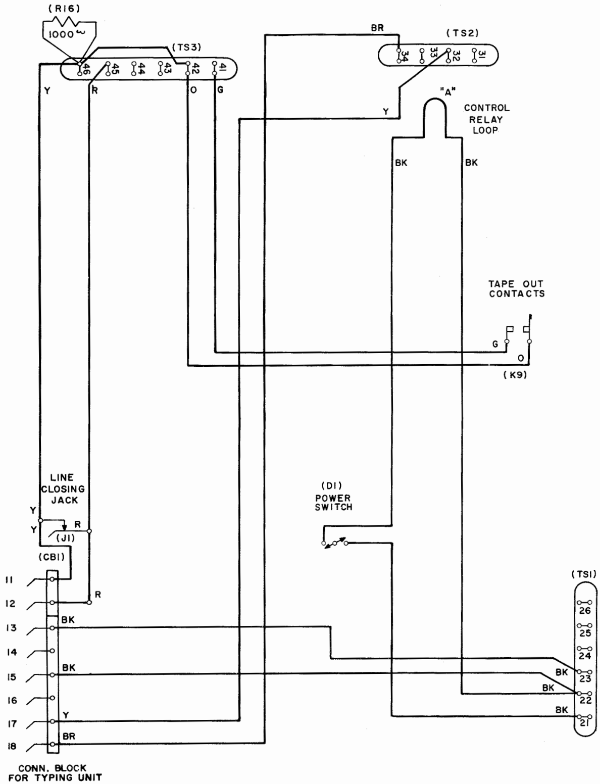
Figure 5 — 14AF Typing Reperforator Base
