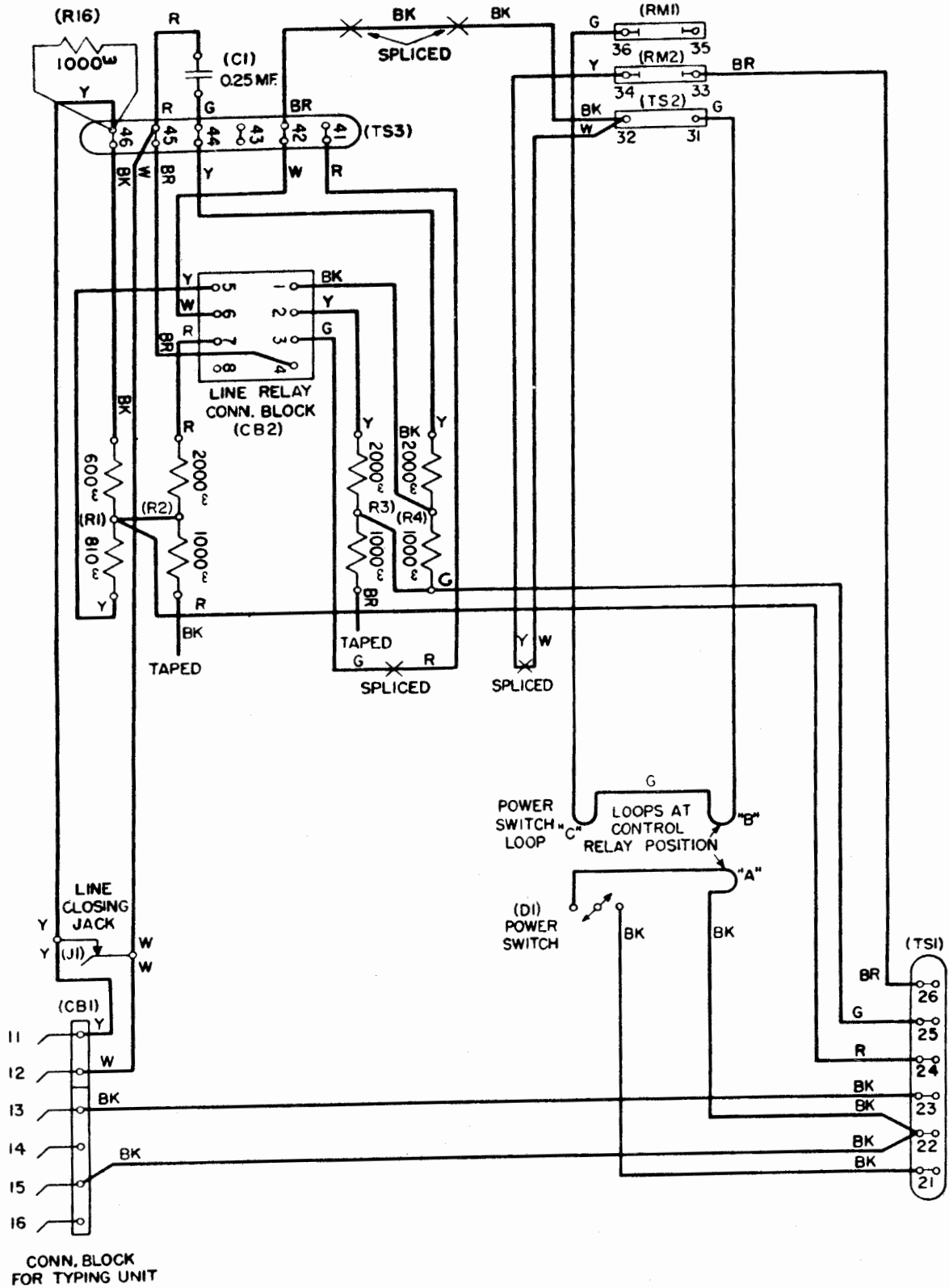
Figure 3 - 14AB Typing Reperforator Base
