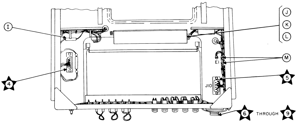
Figure 4-37. Electrical Chassis 1A1, Location of Test Points
