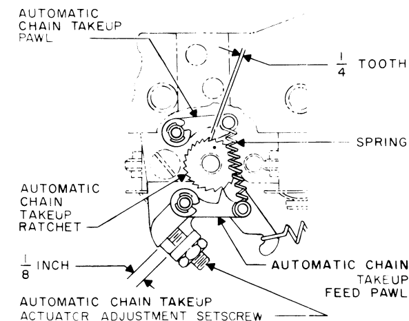
Figure 5-56. Automatic Lateral Chain Takeup Adjustment
