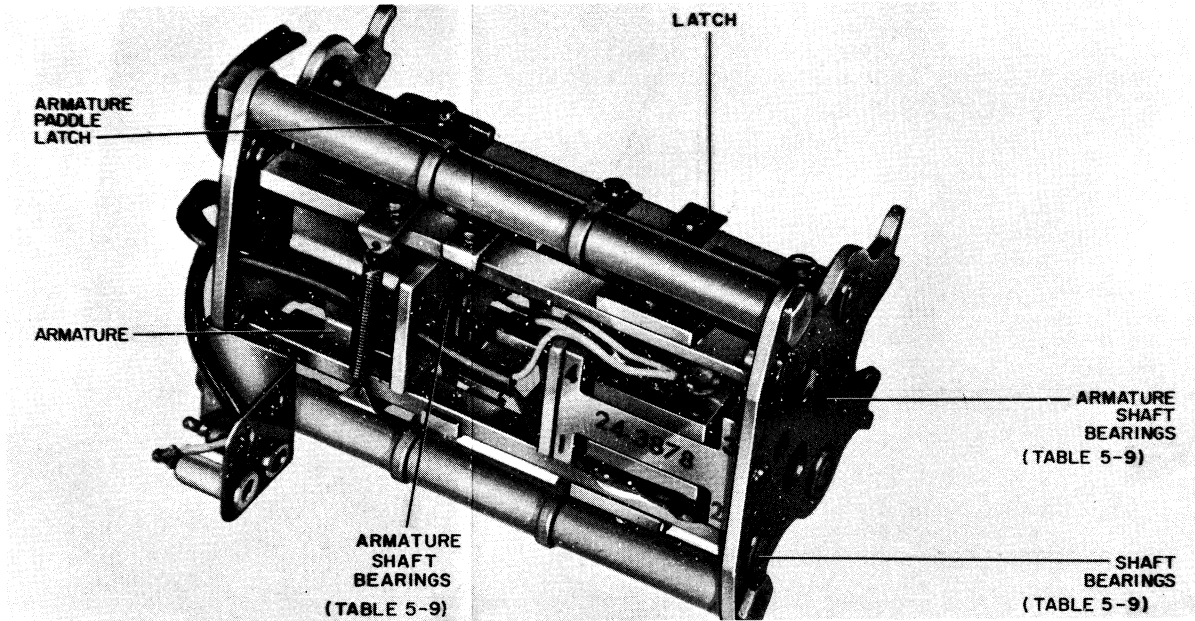
Figure 5-102. Selector Assembly, Lubrication Points
