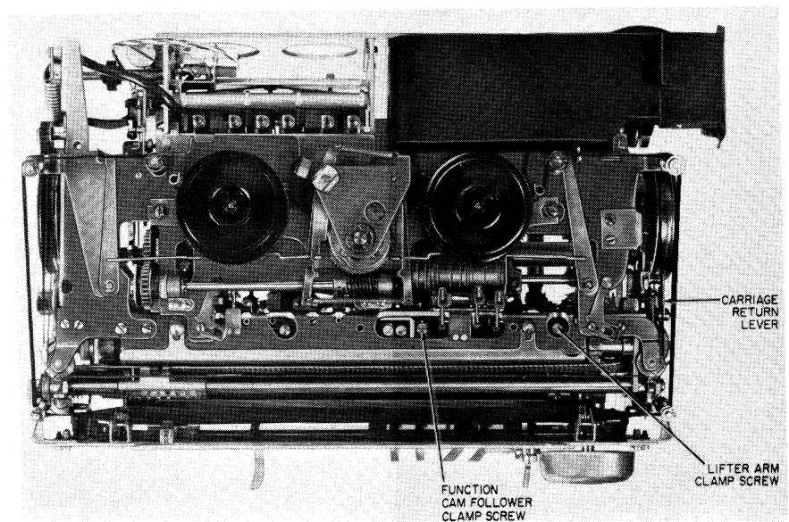
Figure 5-25. Function Selector, Start of Function Cycle
