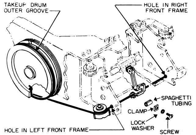
Figure 5-1. Hammer Clamp Location
