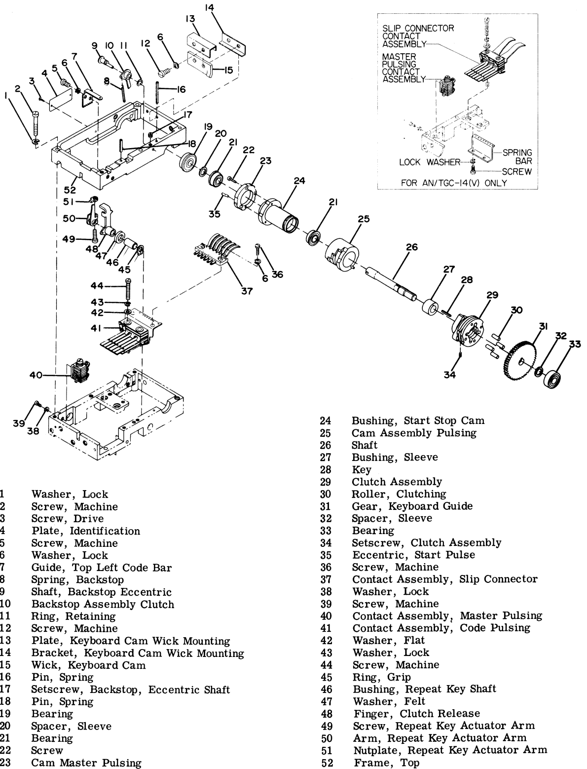
Figure 5-89. Keyboard Assembly (Sheet 3 of 3) SL-4-03315B Figure 6B
