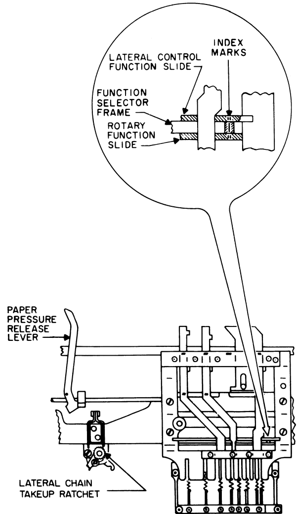
Figure 5-20. Lateral Function Slide Alignment
