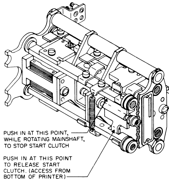
Figure 5-12. Release of Start Clutch
