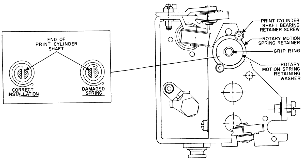
Figure 5-3. Rotary Cable Installation, Left-Side View
