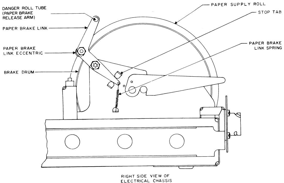
Figure 5-68. Paper Brake Adjustment, Parts Location
