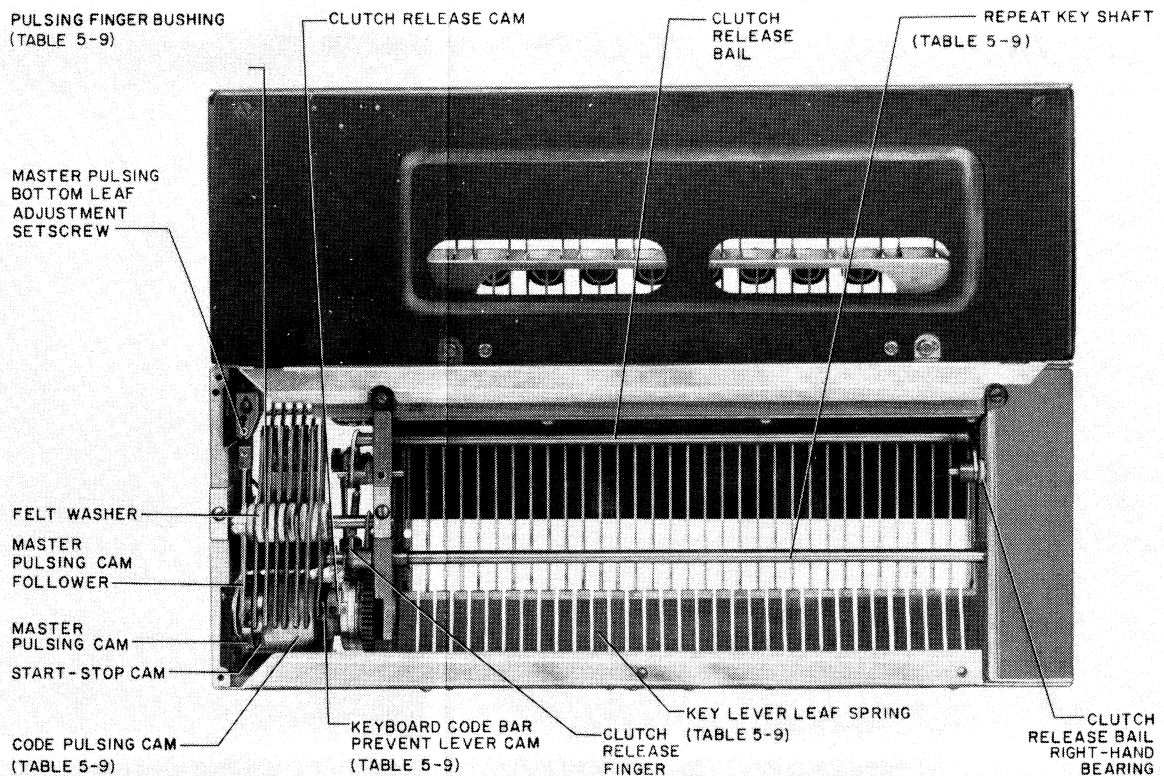
Figure 5-105. Keyboard Assembly, Bottom View (TT-318A/UG)
