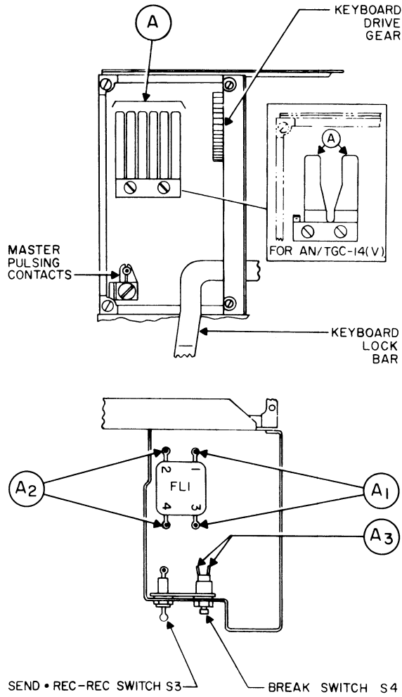
Figure 4-9. Keyboard 1A9, Location of Test Points
