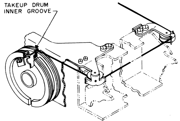
Figure 5-8. Return Cable Installation, Cable Threading Diagram
