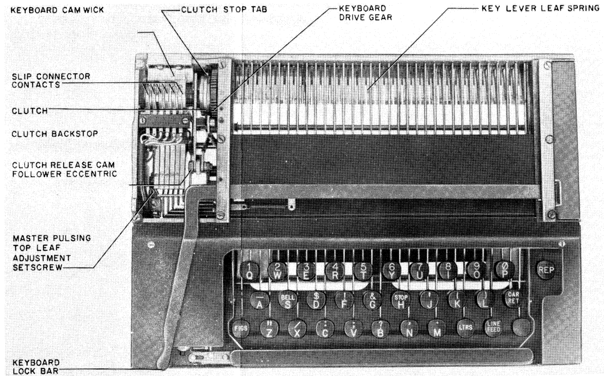
Figure 5-104. Keyboard Assembly, Top View (TT-318A/UG)
