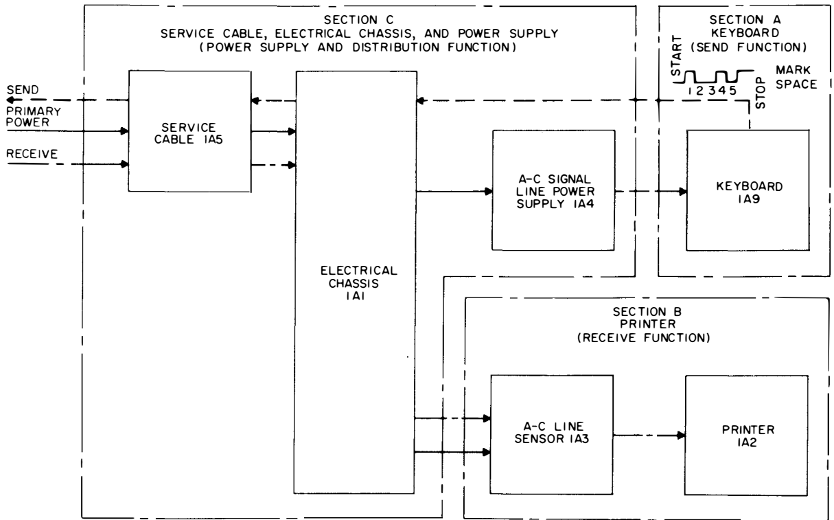
Figure 4-1. Functional Sections
