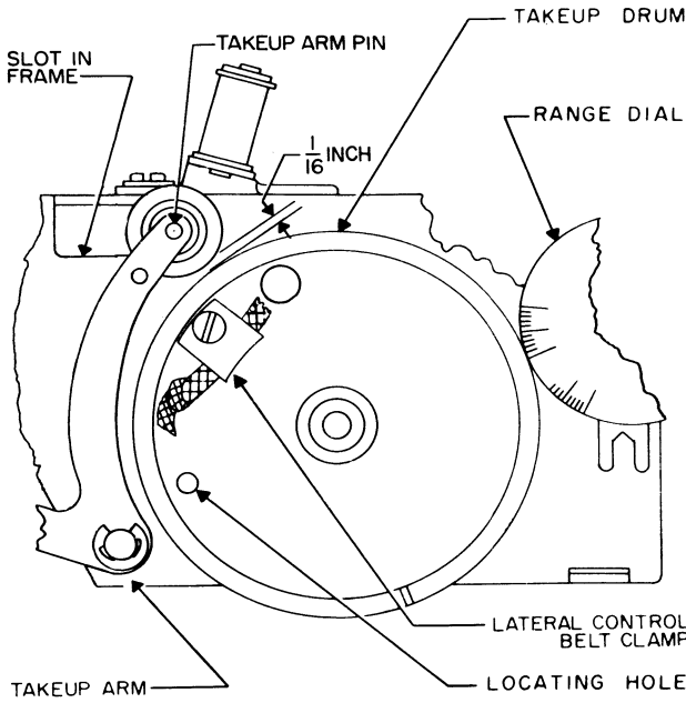
Figure 5-19. Lateral Belt Adjustment, Clearance Requirements
