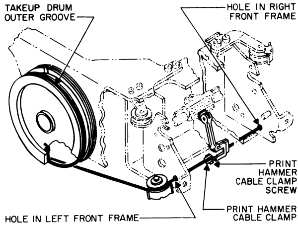
Figure 5-6. Print Hammer Cable Installation, Cable Threading Diagram
