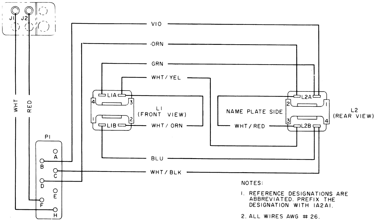
Figure 5-114. Selector, Wiring Diagram
