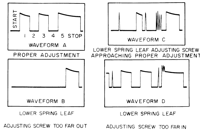
Figure 5-63. Waveforms for Transmitting Letters Y
