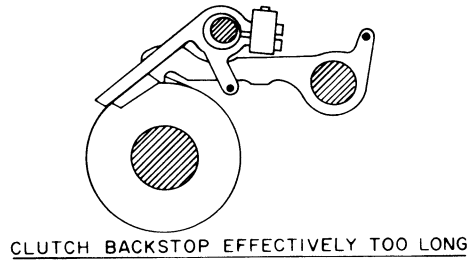
Figure 5-14. Clutch Back-Stop Adjustment
