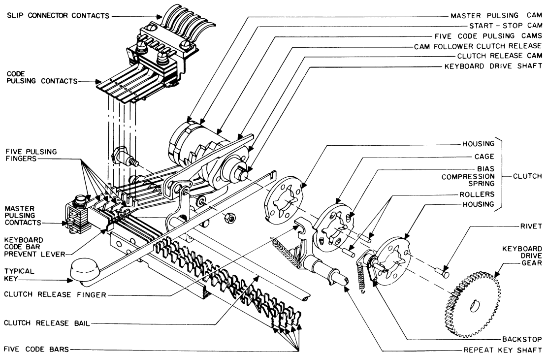
Figure 4-7. Keyboard 1A9, Mechanical Diagram
