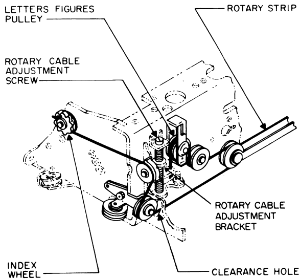
Figure 5-4. Rotary Cable Installation, Cable Threading Diagram
