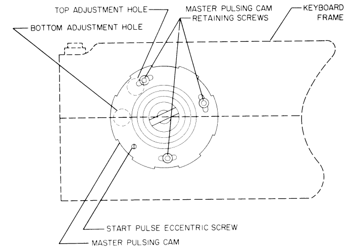
Figure 5-66. Keyboard Timing Adjustment
