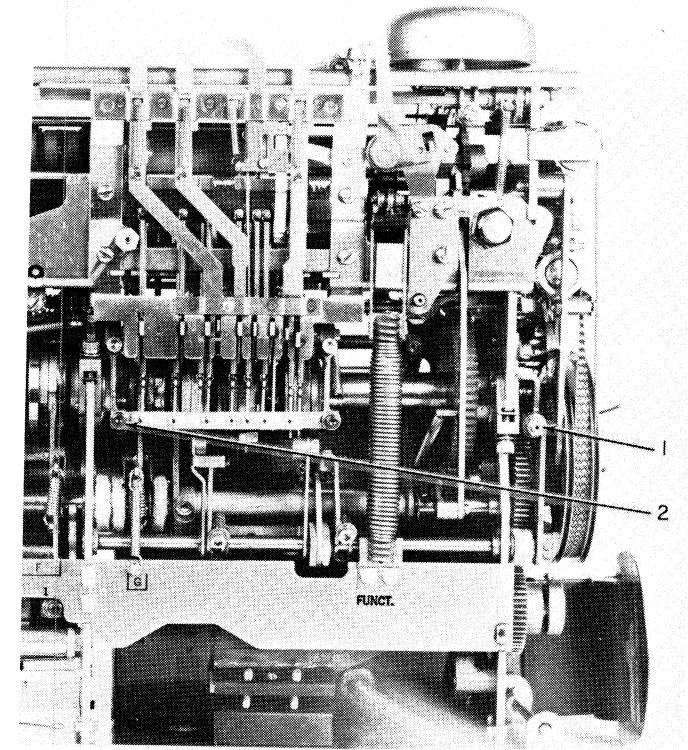
Figure 5-52. Spacing of the First Character
