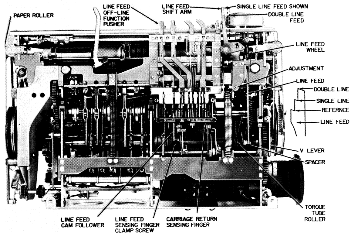
Figure 5-36. Line Feed Adjustment
