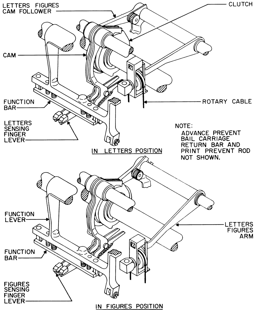
Figure 4-28. Function Selector, Letters Figures Linkage
