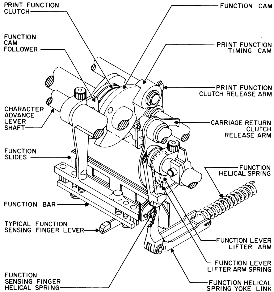
Figure 4-24. Function Selector, Start of Function Cycle
