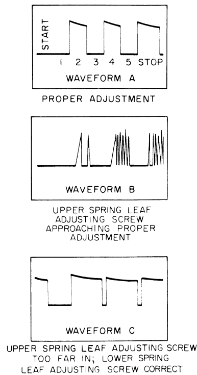
Figure 5-62. Waveforms for Transmitting Letters R
