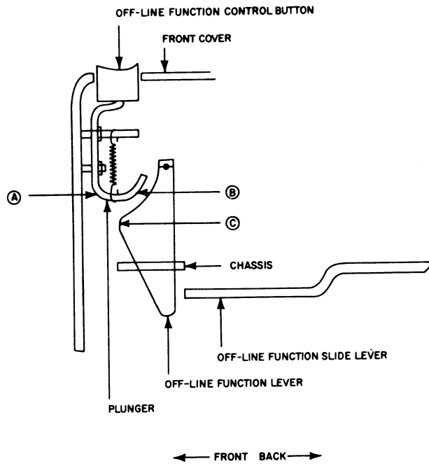
Figure 5-67. Off-Line Function Control Button Mechanism
