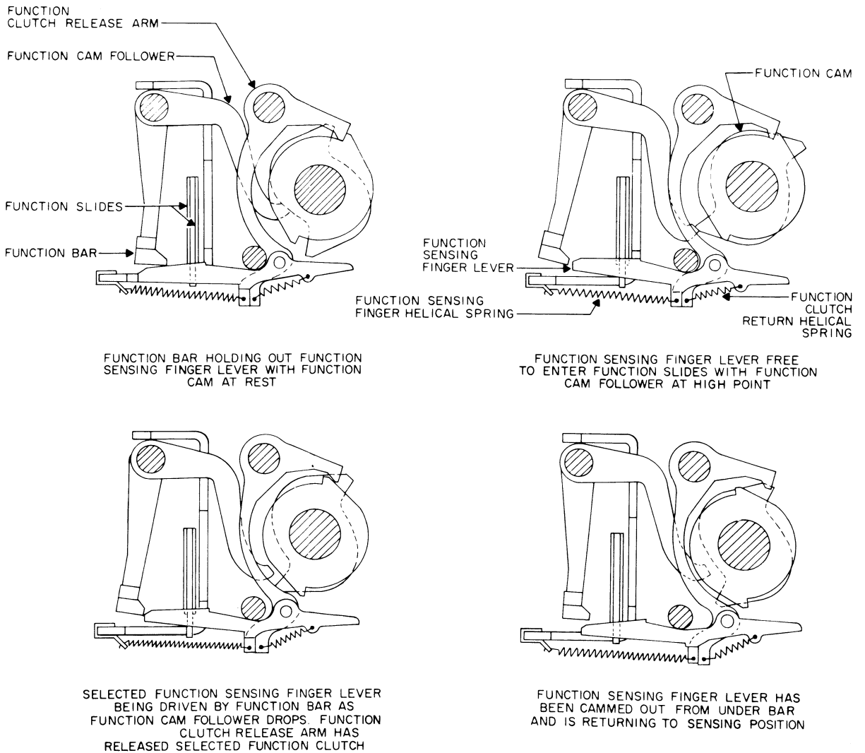
Figure 4-25. Function Selector, Operating Cycle
