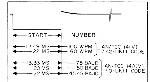
Figure 5-65. Waveform for Timing Adjustment
