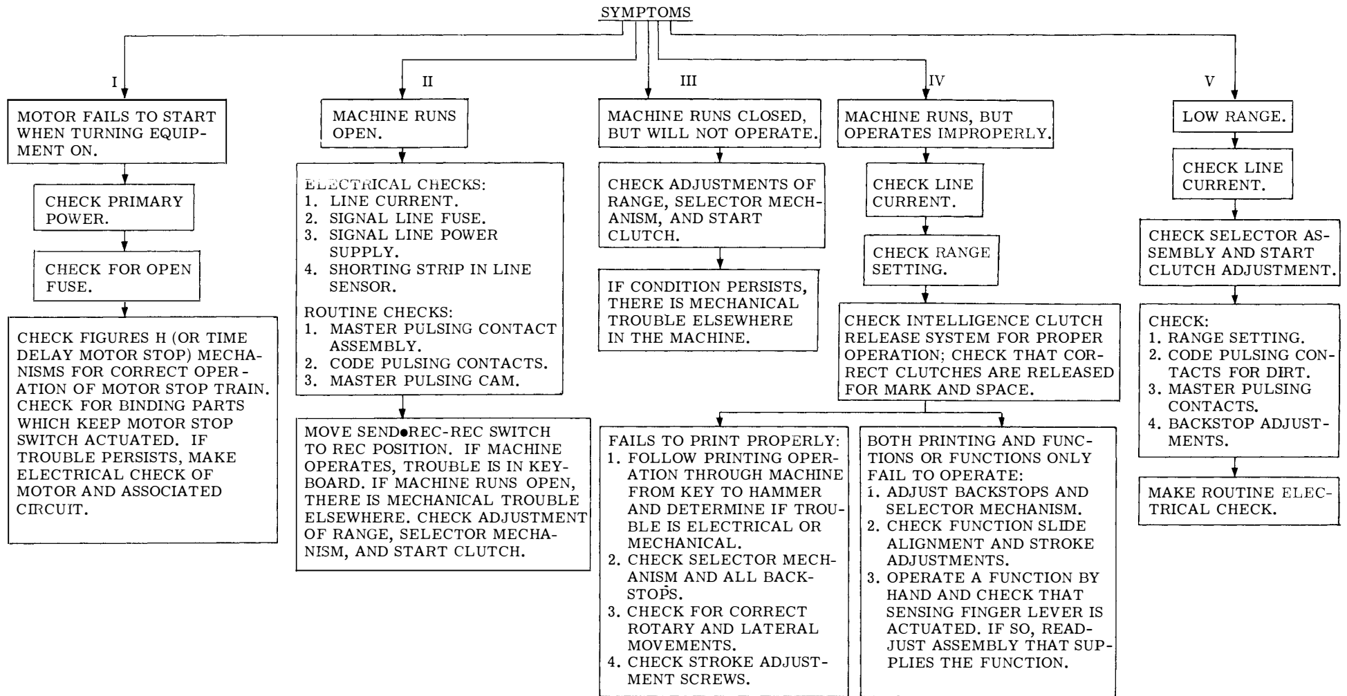
Figure 4-5. Trouble-Shooting Flow Chart
