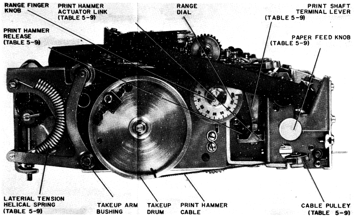
Figure 5-103. Printer Assembly, Left-Side View
