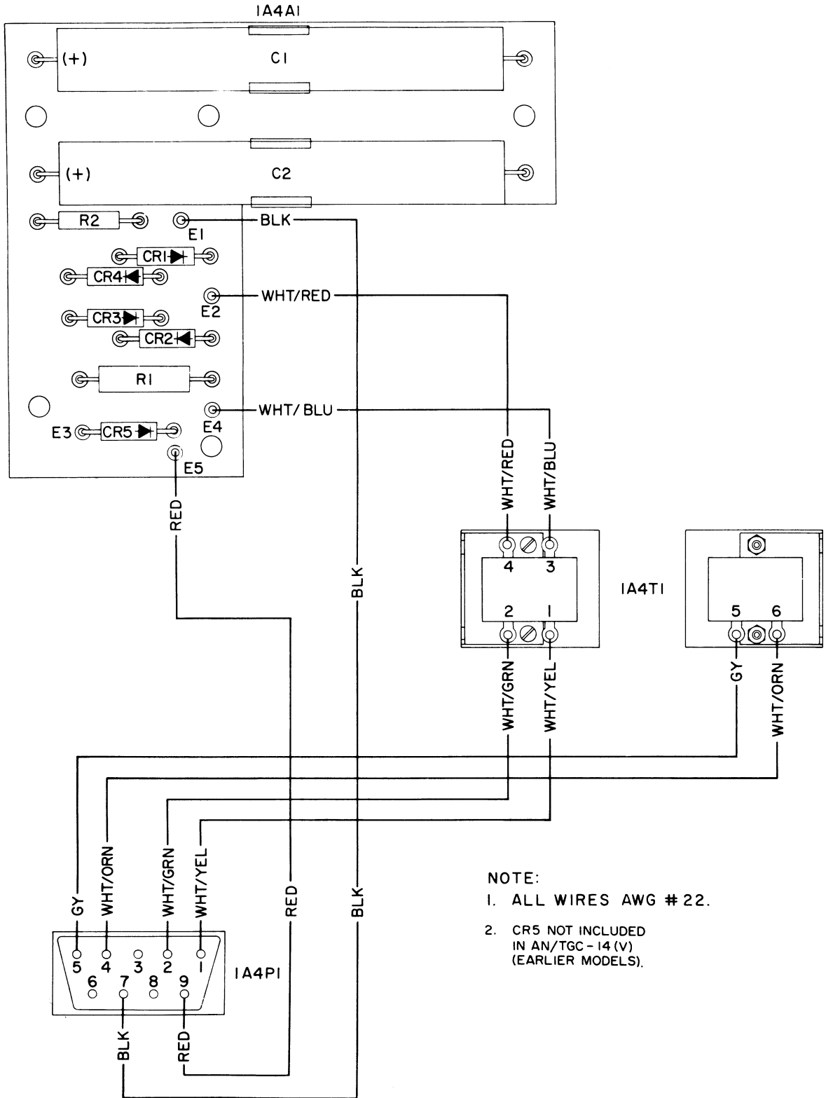
Figure 5-111. Signal Line Power Supply, Wiring Diagram
