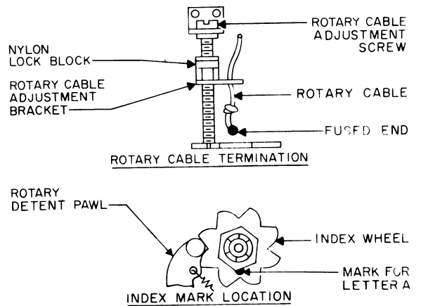
Figure 5-5. Rotary Cable Installation, Detail Views
