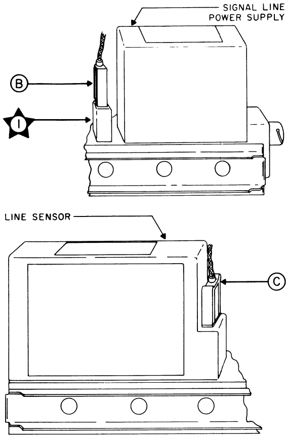
Figure 4-34. Printer 1A2, Location of Test Points
