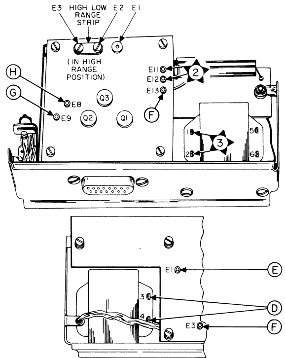
Figure 4-13. Line Sensor 1A3, Location of Test Points
