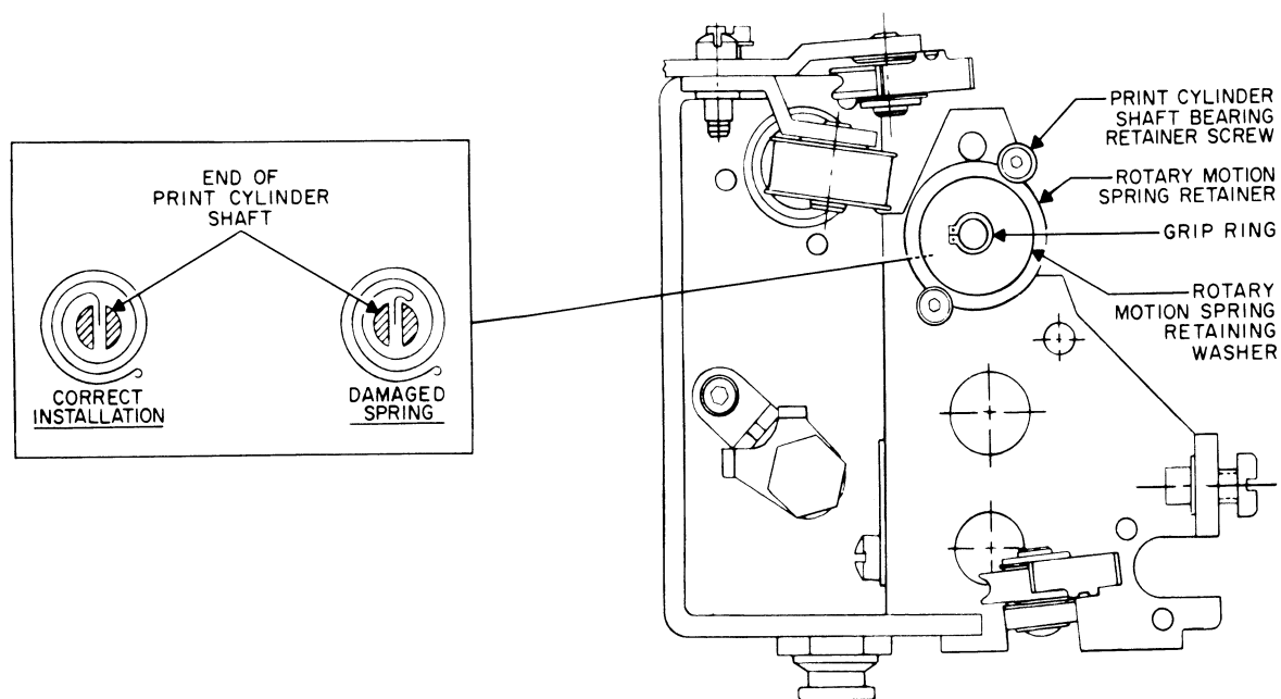
Figure 5-99. Start Clutch Release Mechanism, Exploded View
