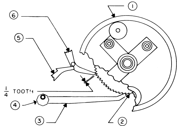
View B
