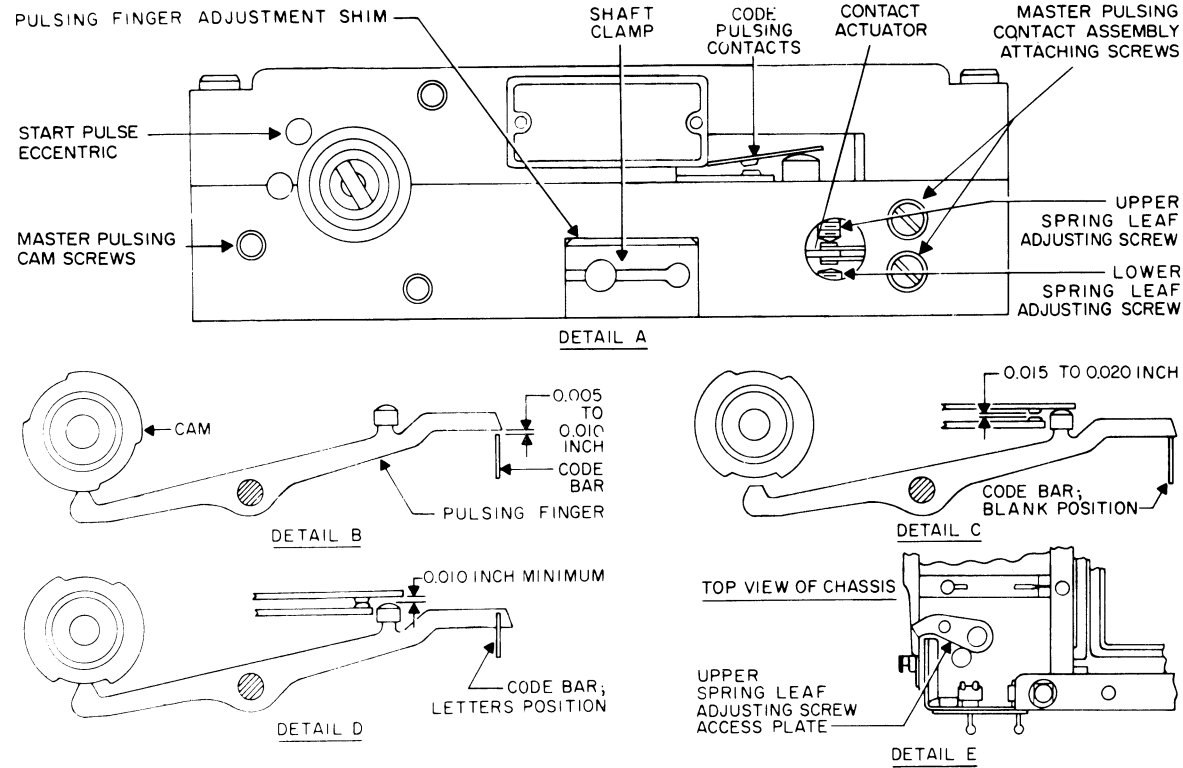
Figure 5-61. Keyboard Adjustment, Parts Location
