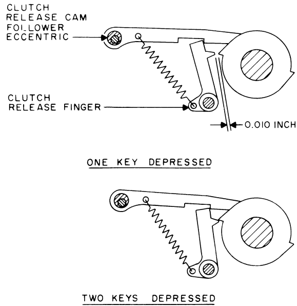
Figure 5-58. Clutch Release Lever Eccentric Adjustment
