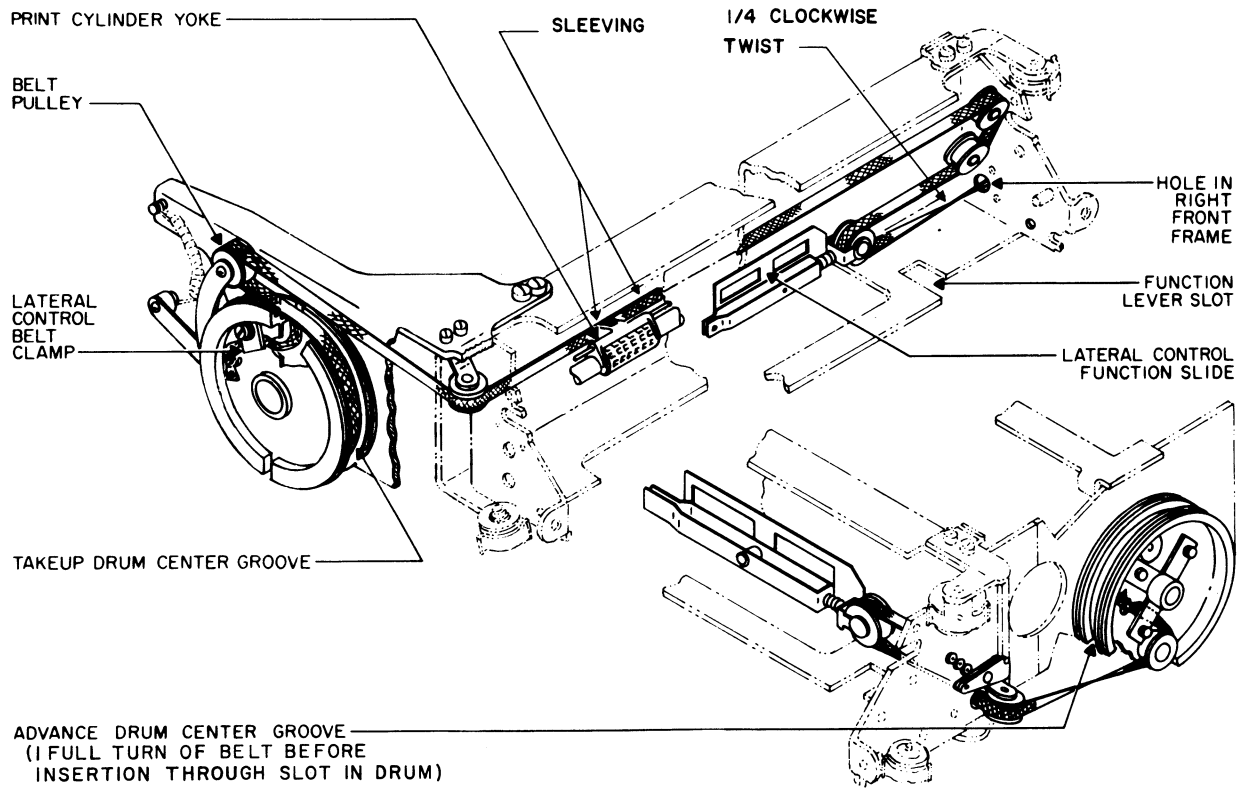
Figure 5-1A. Fiberglass Lateral Control Belt Installation, Belt Threading Diagram
