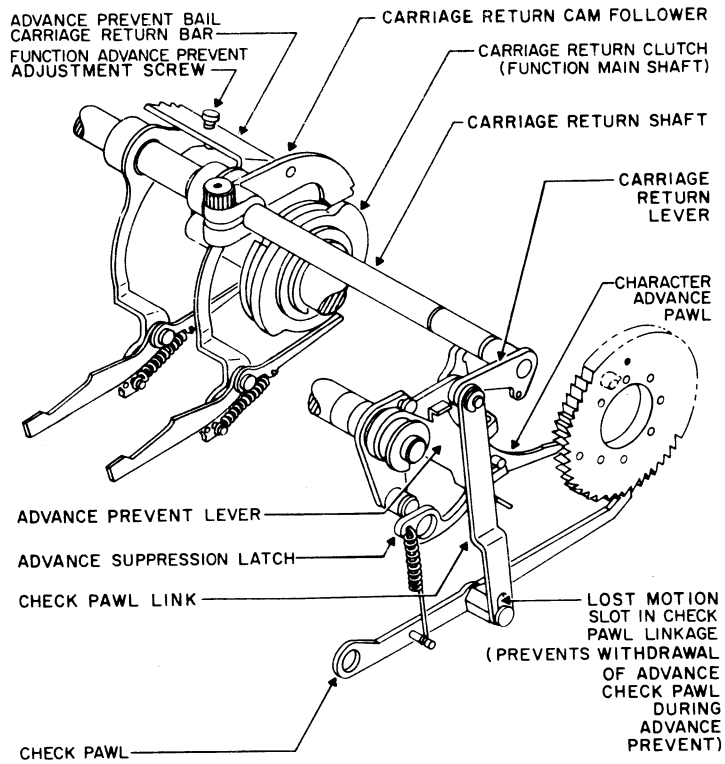
Figure 4-31. Function Selector, Character Advance Prevent Linkage
