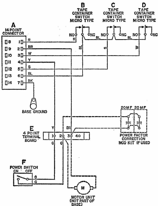
28B Typing Reperforator Base
