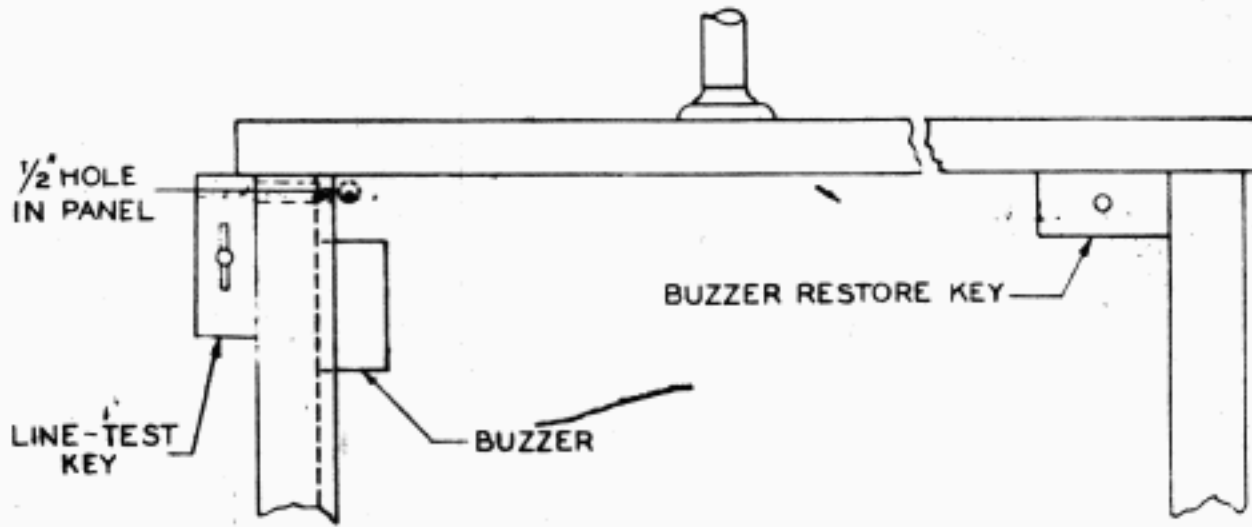
FRONT VIEW RECEIVING STATION
