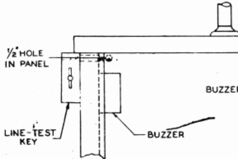
FRONT VIEW RECEIVING STATION
