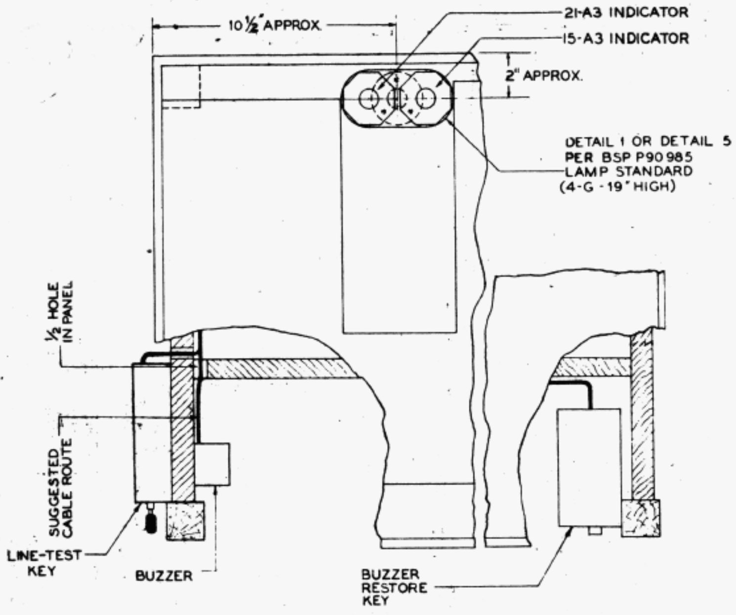
TOP VIEW RECEIVING STATION
