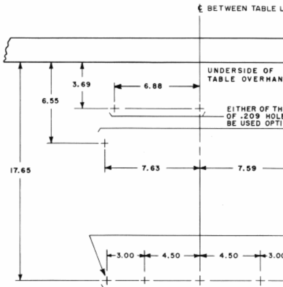
HOLE LOCATIONS FOR MOUNTING DATA SET
