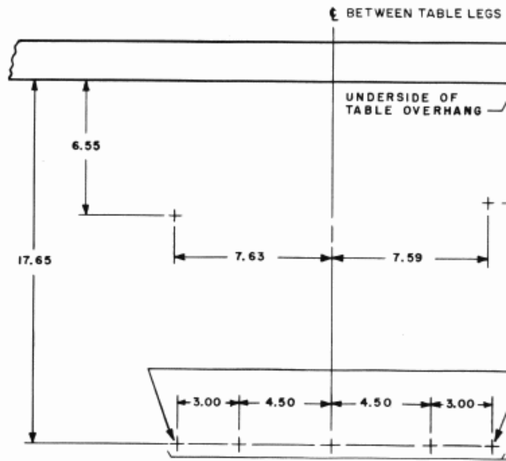
HOLE LOCATIONS FOR MOUNTING DATA SET
