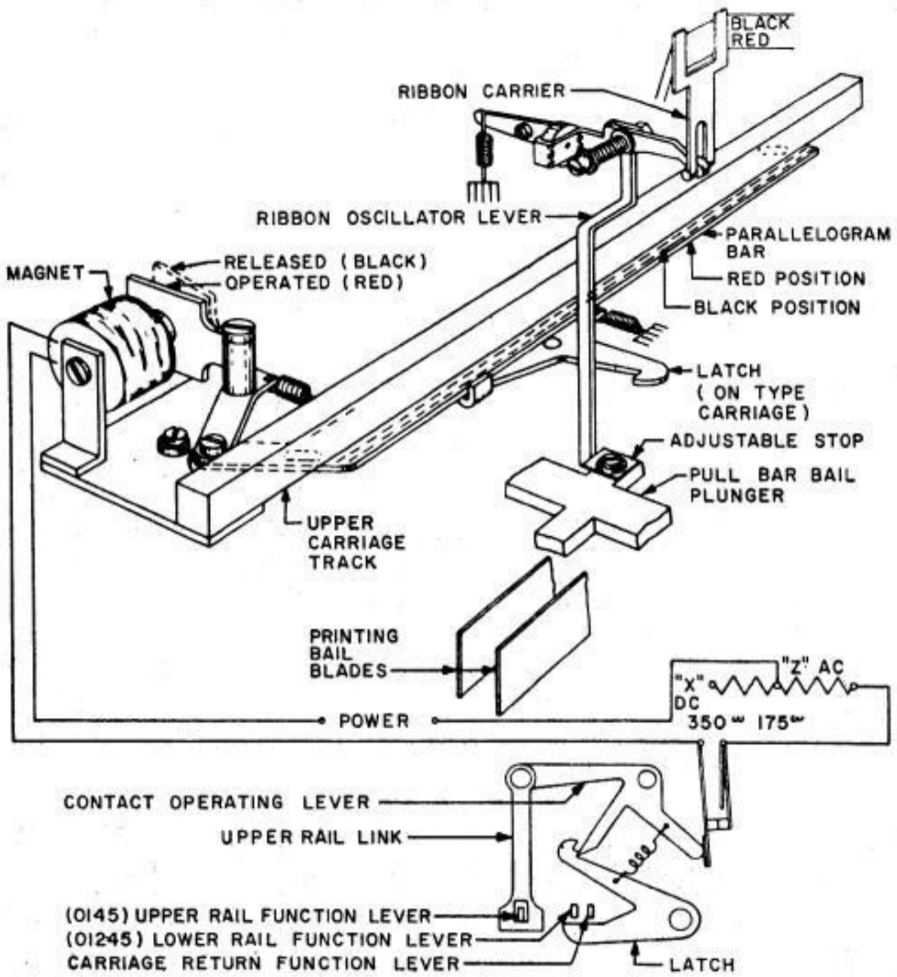
Fig. 1—20 TELETYPEWRITER TWO-COLOR PRINTING MECHANISM THEORY SKETCH
