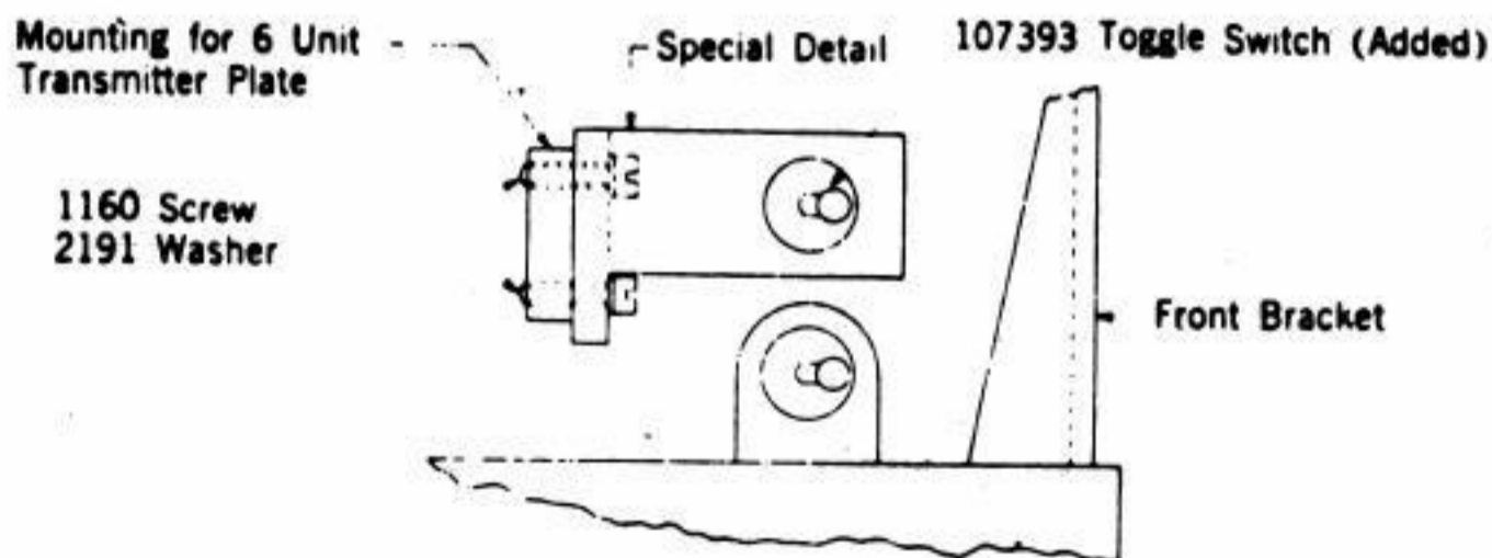
MOUNTING ARRANGEMENT OF MOTOR SWITCH DETAIL FIG. 2 (A & M)
