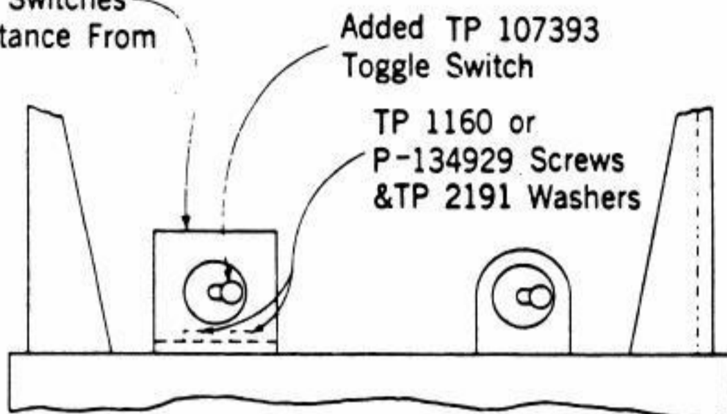
MOUNTING ARRANGEMENT OF MOTOR SWITCH DETAIL
