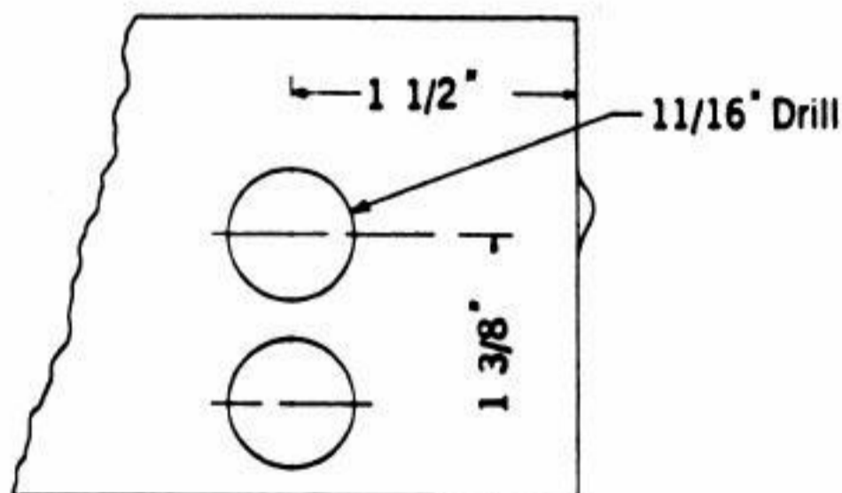
MODIFICATION OF TRANSMITTER SNAP PANEL FIG. 1 (A & M)
