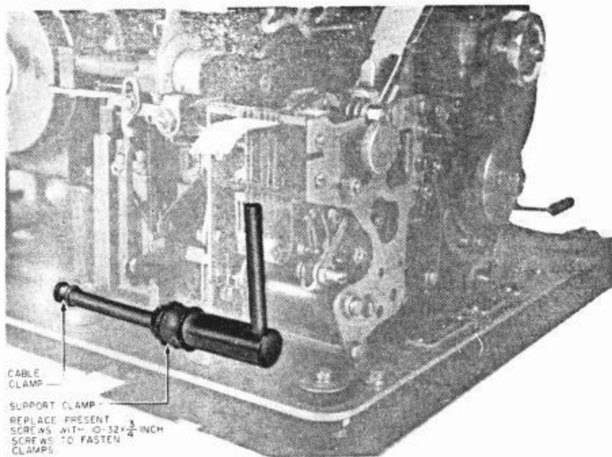
Fig. 8—Inductor Point Mounted on 28 Typing Reperforator
