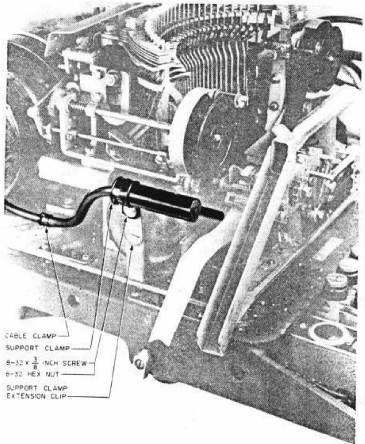
Fig. 6—Inductor Point Mounted on 14 Typing Reperforator
