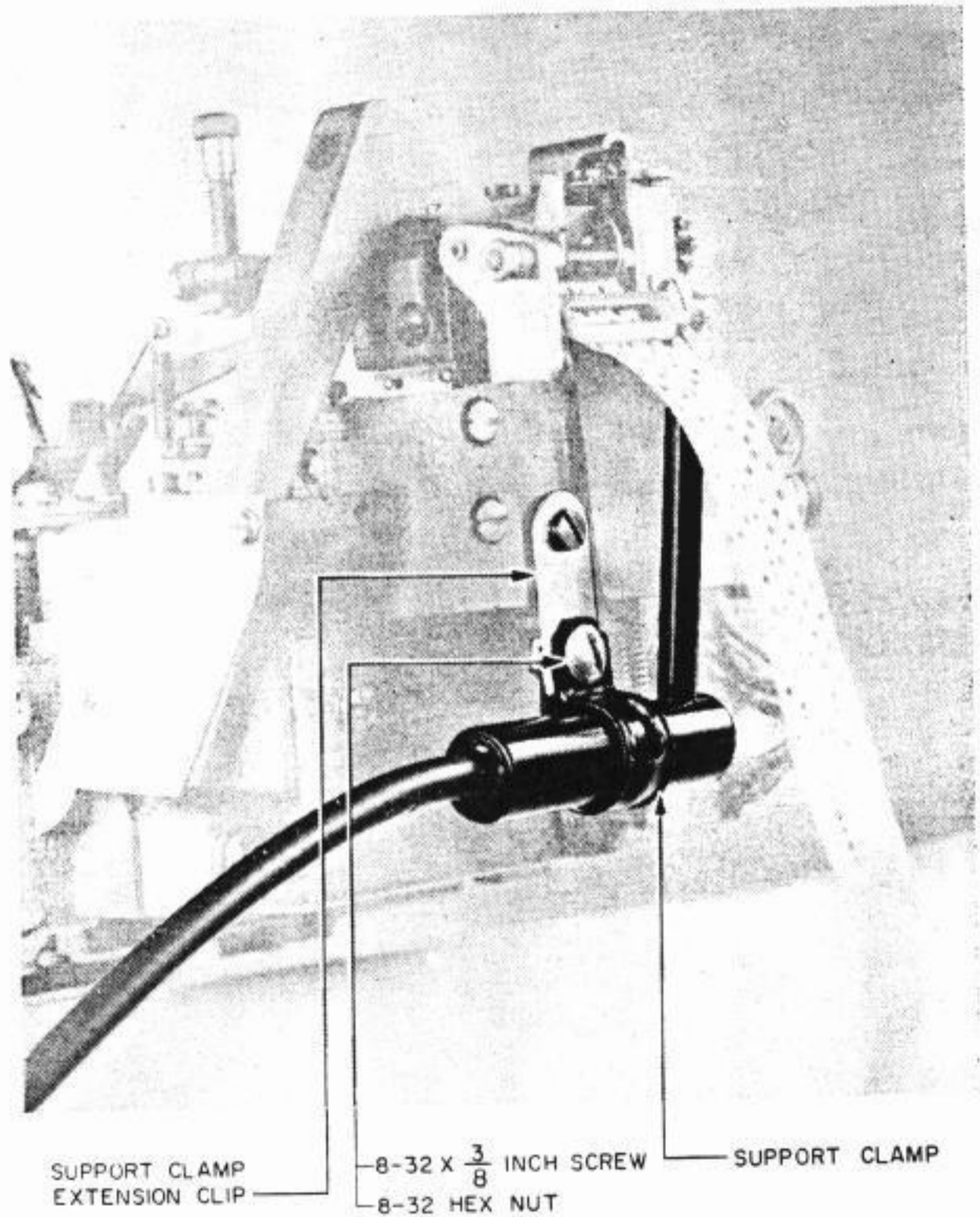
Fig. 10—Inductor Point Mounted on Perforator of 19 Teletypewriter Set
