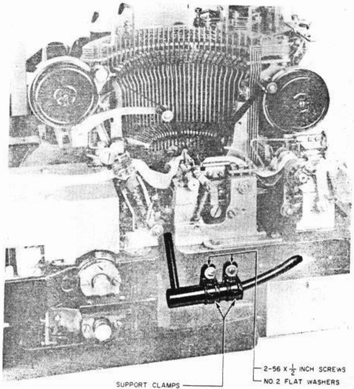
Fig. 7—Inductor Point Mounted on 14 Reperforator-Transmitter
