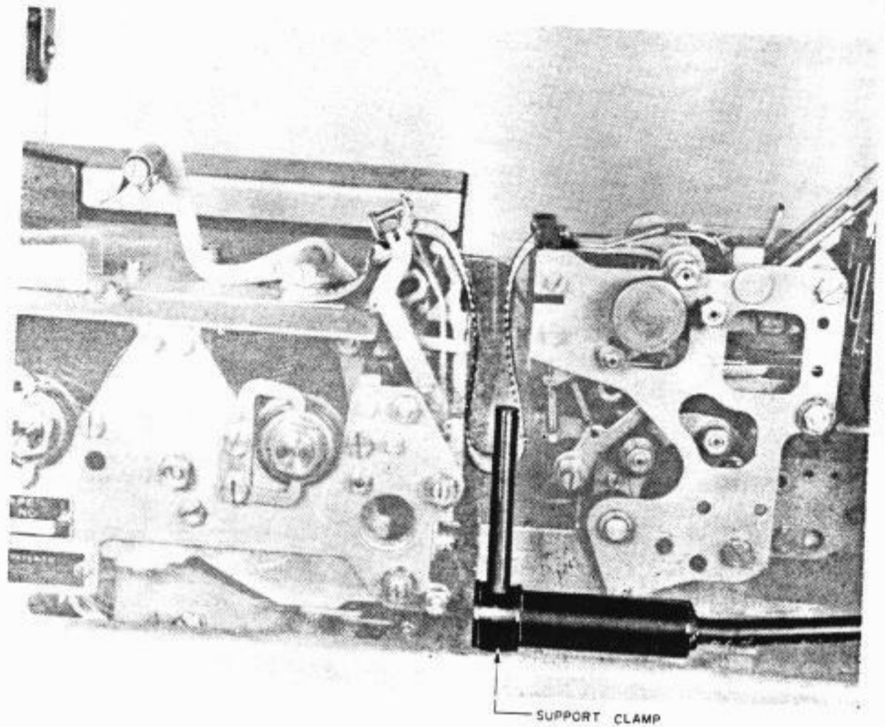
Fig. 9—Inductor Point Mounted on 28 Reperforator-Transmitter
