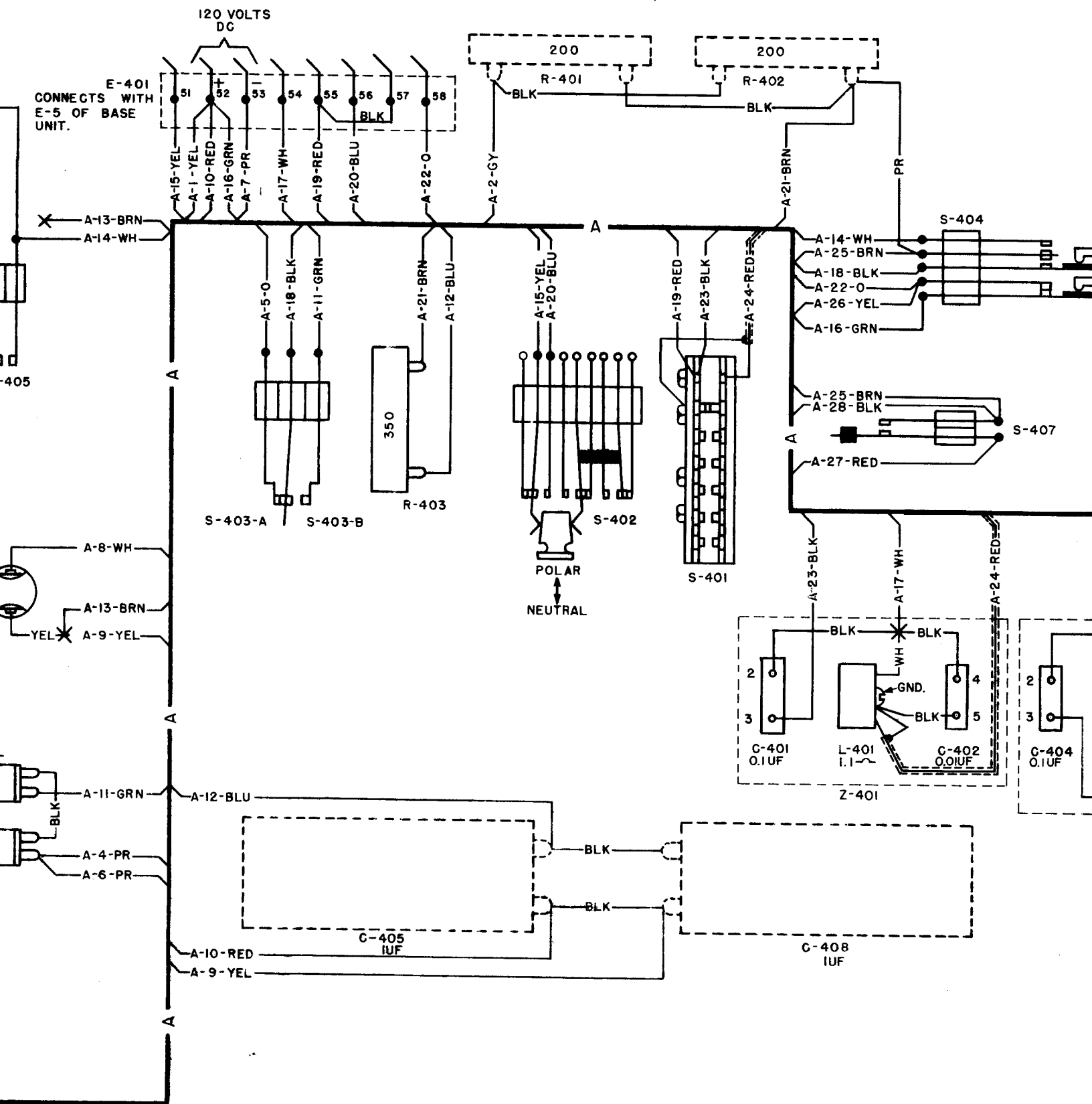
Figure 271. Perforator transmitter, actual wiring diagram.
