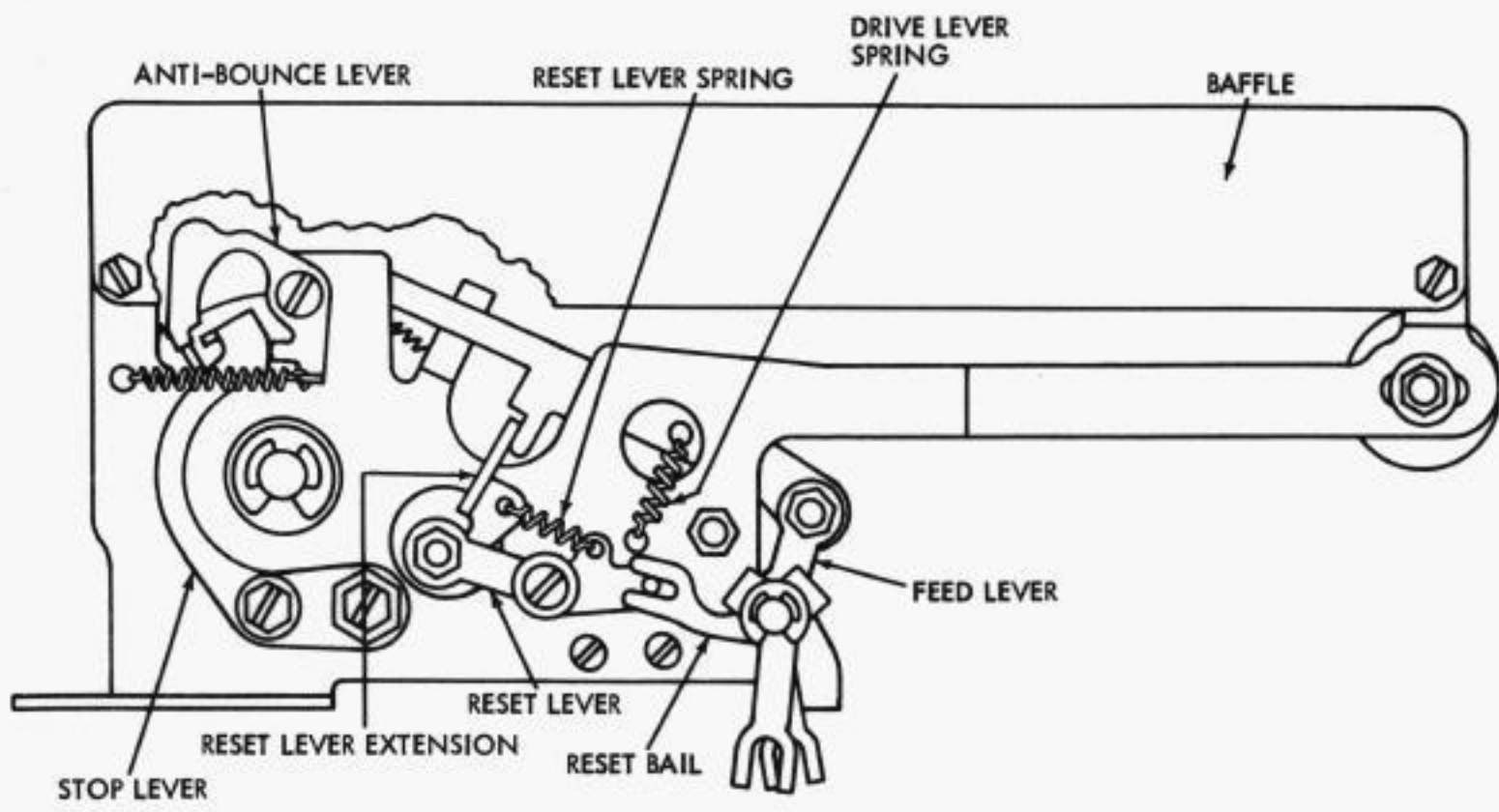
FIGURE 2-15 CHARACTER COUNTER MECHANISM, REAR VIEW
