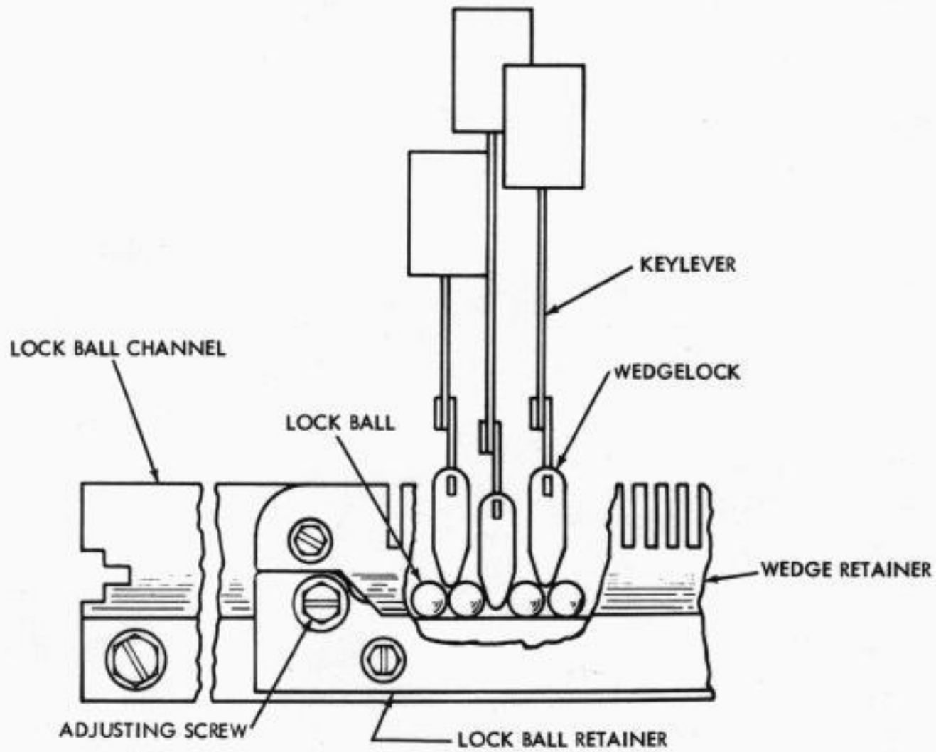
FIGURE 2-2 WEDGELOCK MECHANISM
