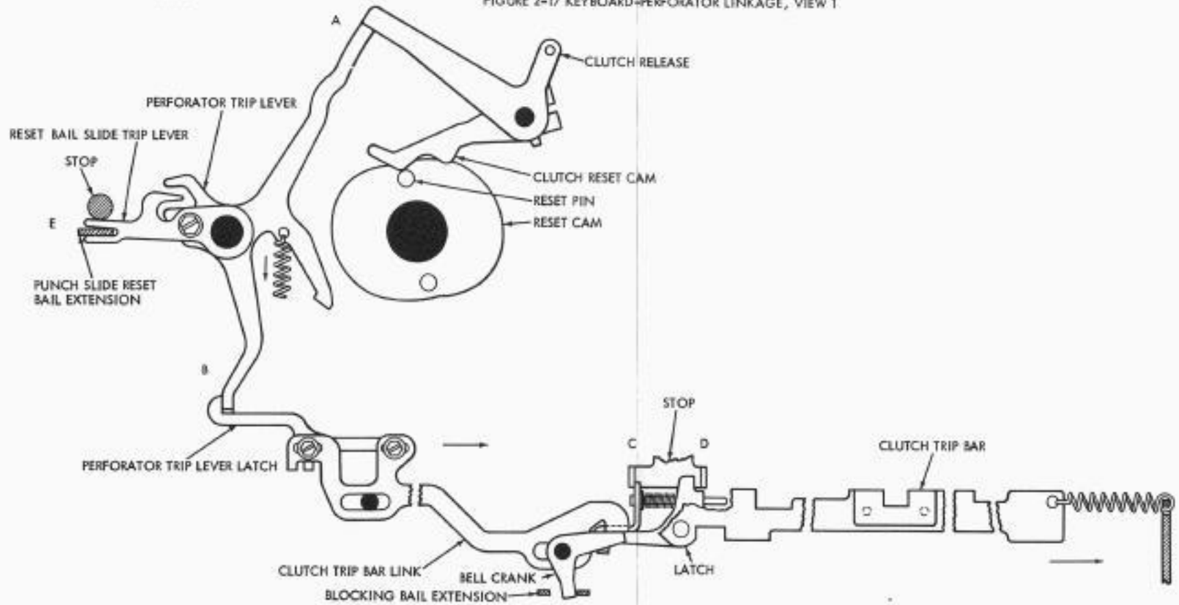
FIGURE 2-18 KEYBOARD - PERFORATOR LINKAGE, VIEW 2
