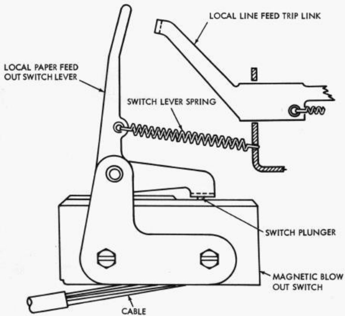
FIGURE 2-9 LOCAL PAPER FEED OUT MECHANISM
