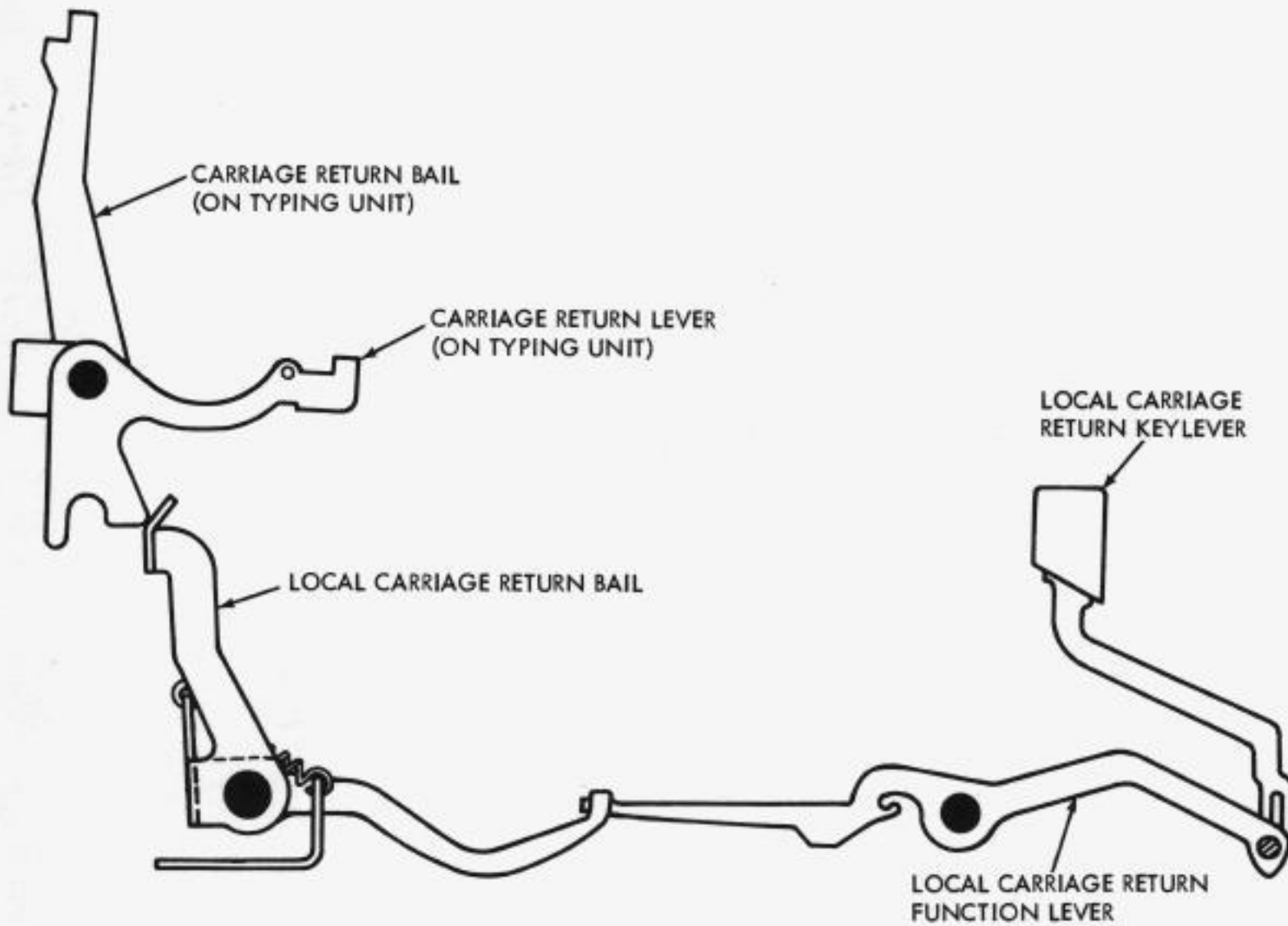
FIGURE 2-12 LOCAL CARRIAGE RETURN MECHANISM
