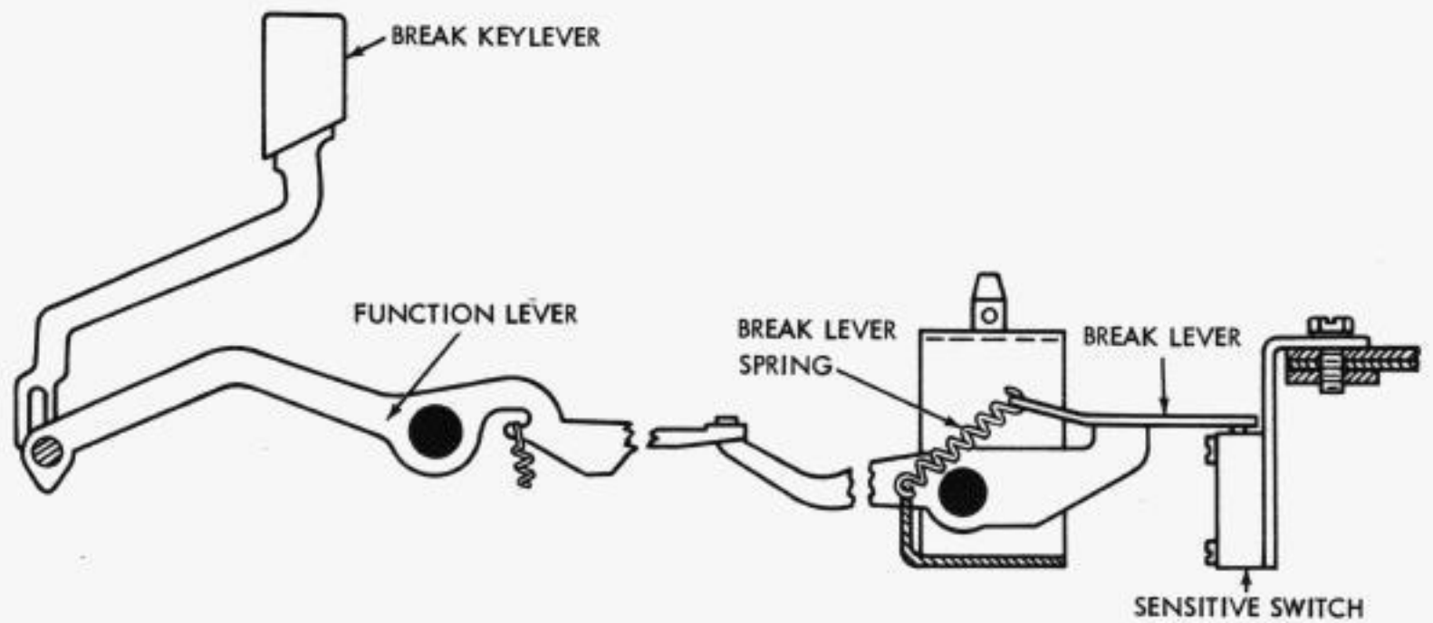
FIGURE 2-7 ELECTRICAL LINE BREAK MECHANISM
