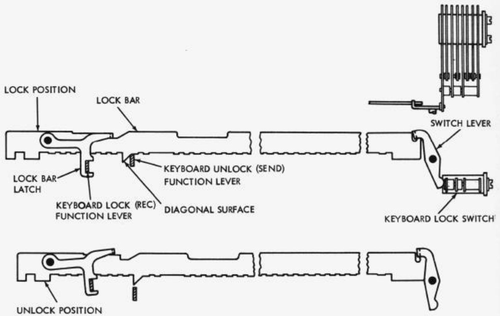
FIGURE 2-10 ELECTRICAL KEYBOARD LOCK MECHANISM
