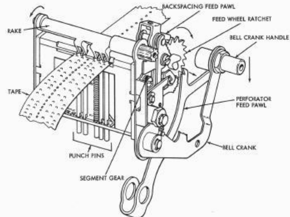
FIGURE 2-21 POWER DRIVE BACKSPACE MECHANISM, VIEW 1
