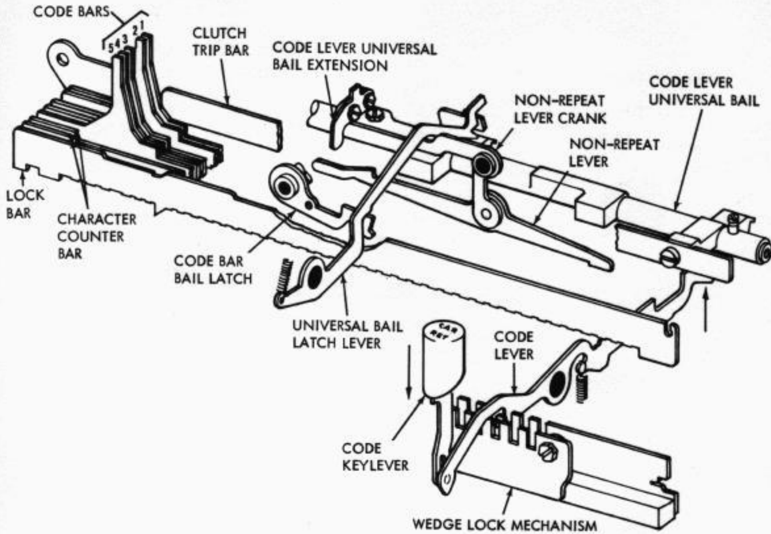
FIGURE 2-1 CODE BAR & CODE LEVER UNIVERSAL BAIL MECHANISM
