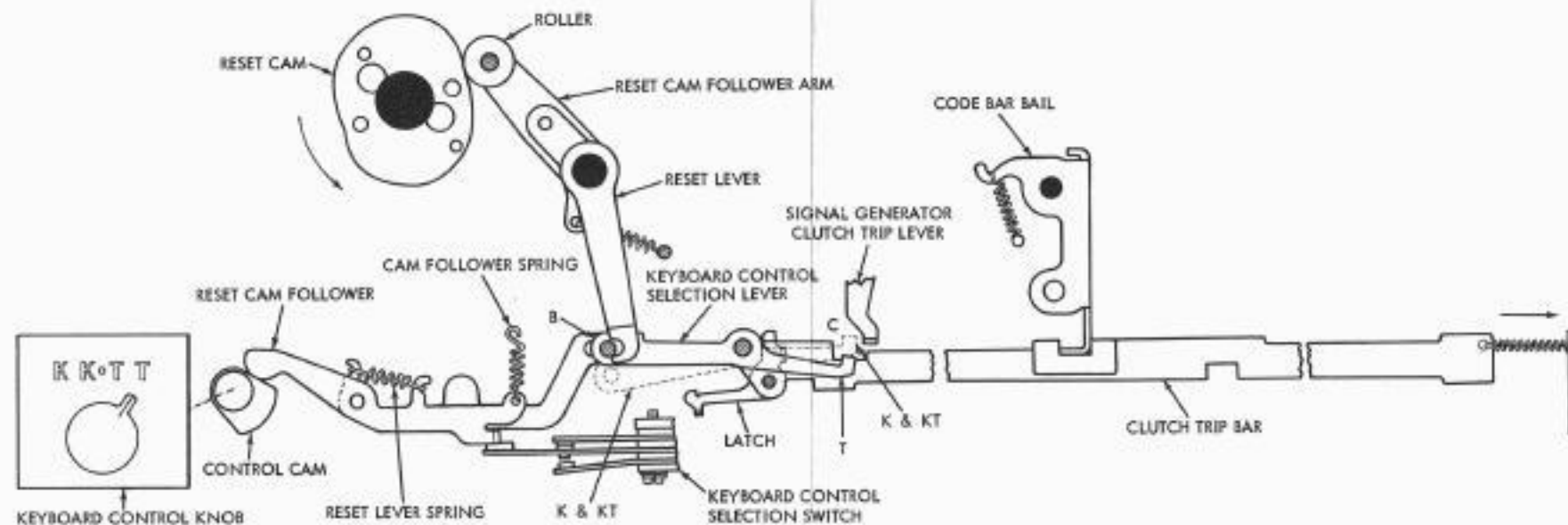
FIGURE 2-19 KEYBOARD - PERFORATOR LINKAGE, VIEW 3
