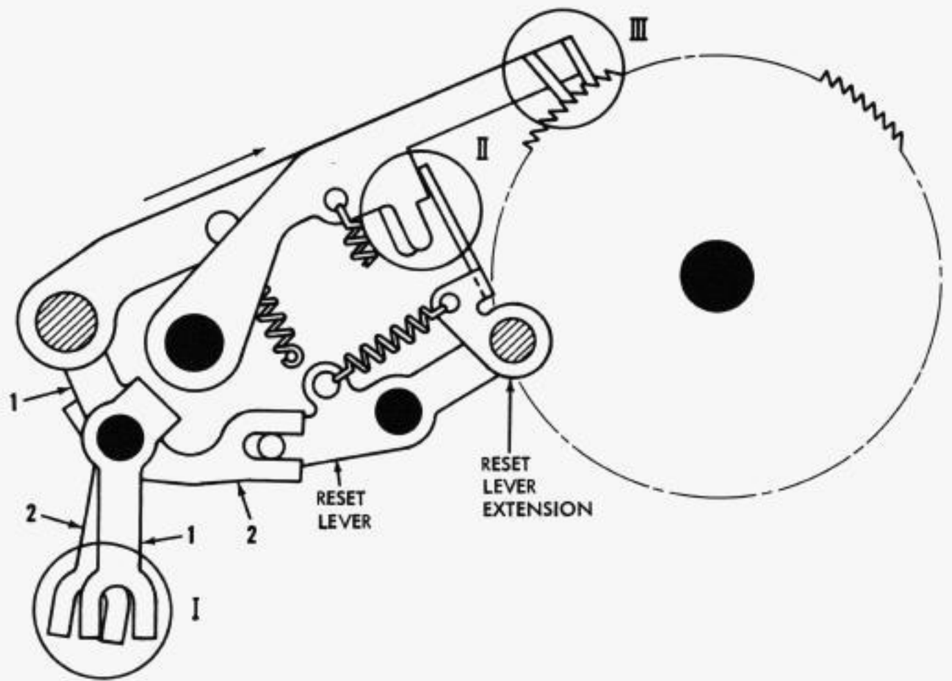
FIGURE 2-16 OPERATION OF CHARACTER COUNTER MECHANISM
