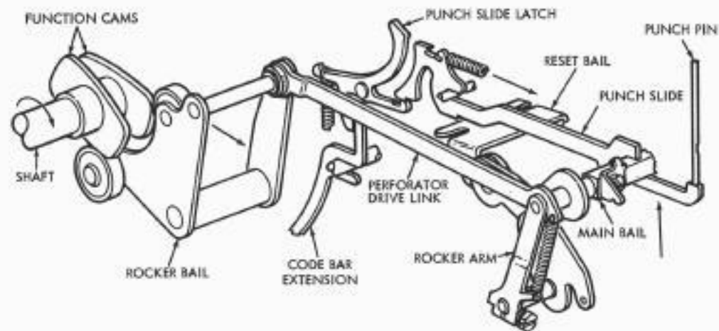
FIGURE 2-20 PERFORATOR PUNCH MECHANISM
