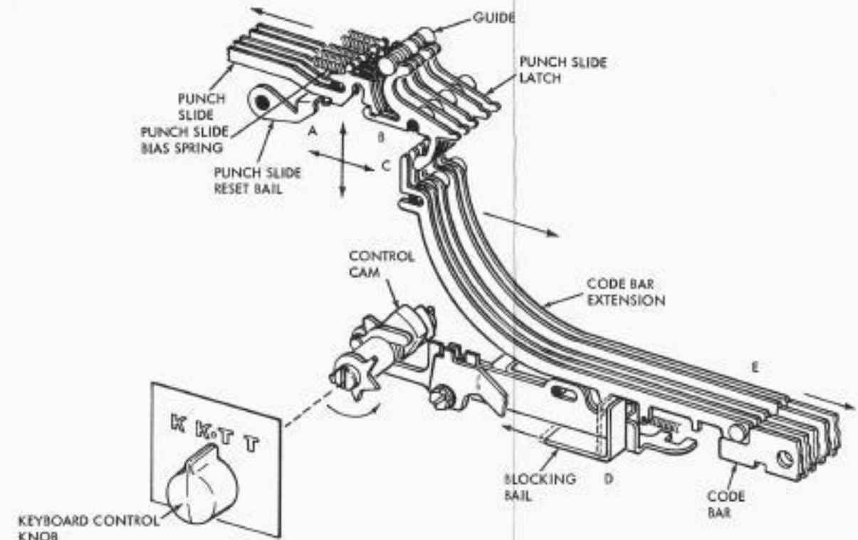
FIGURE 2-17 KEYBOARD-PERFORATOR LINKAGE, VIEW 1
