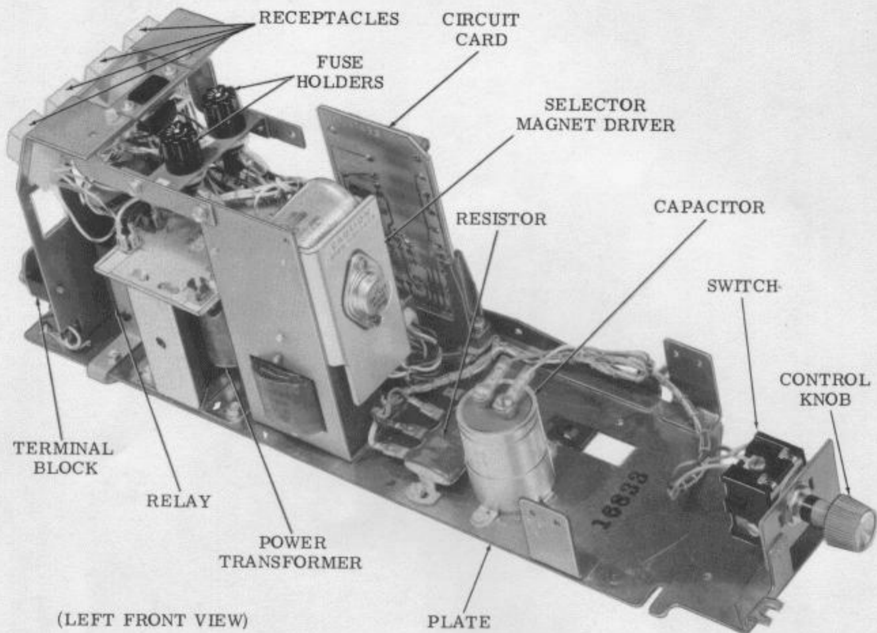
Figure 12 — Typical Call Control Unit
