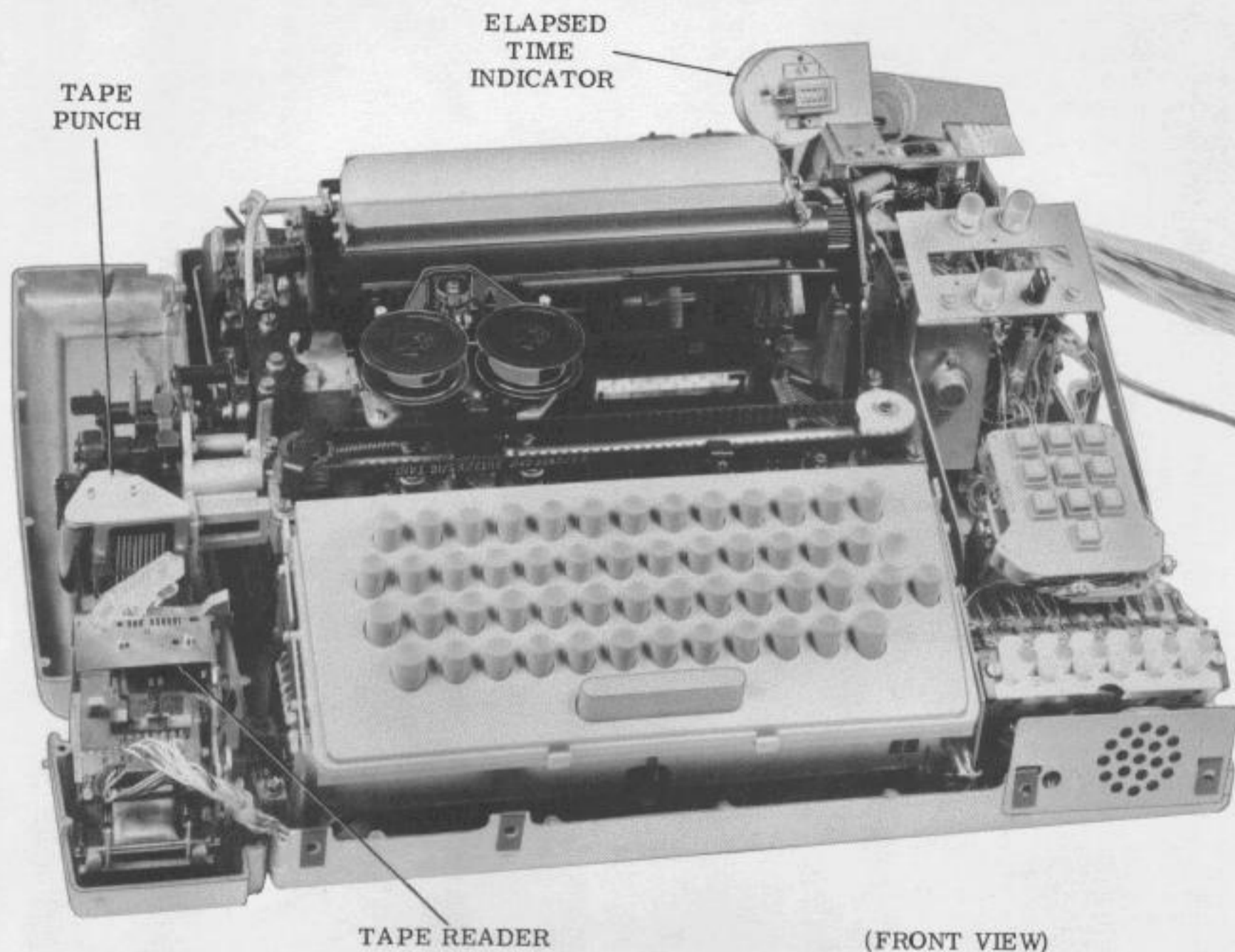
Figure 4 — Automatic Send-Receive (ASR) Teletypewriter Set (Without Cover)
