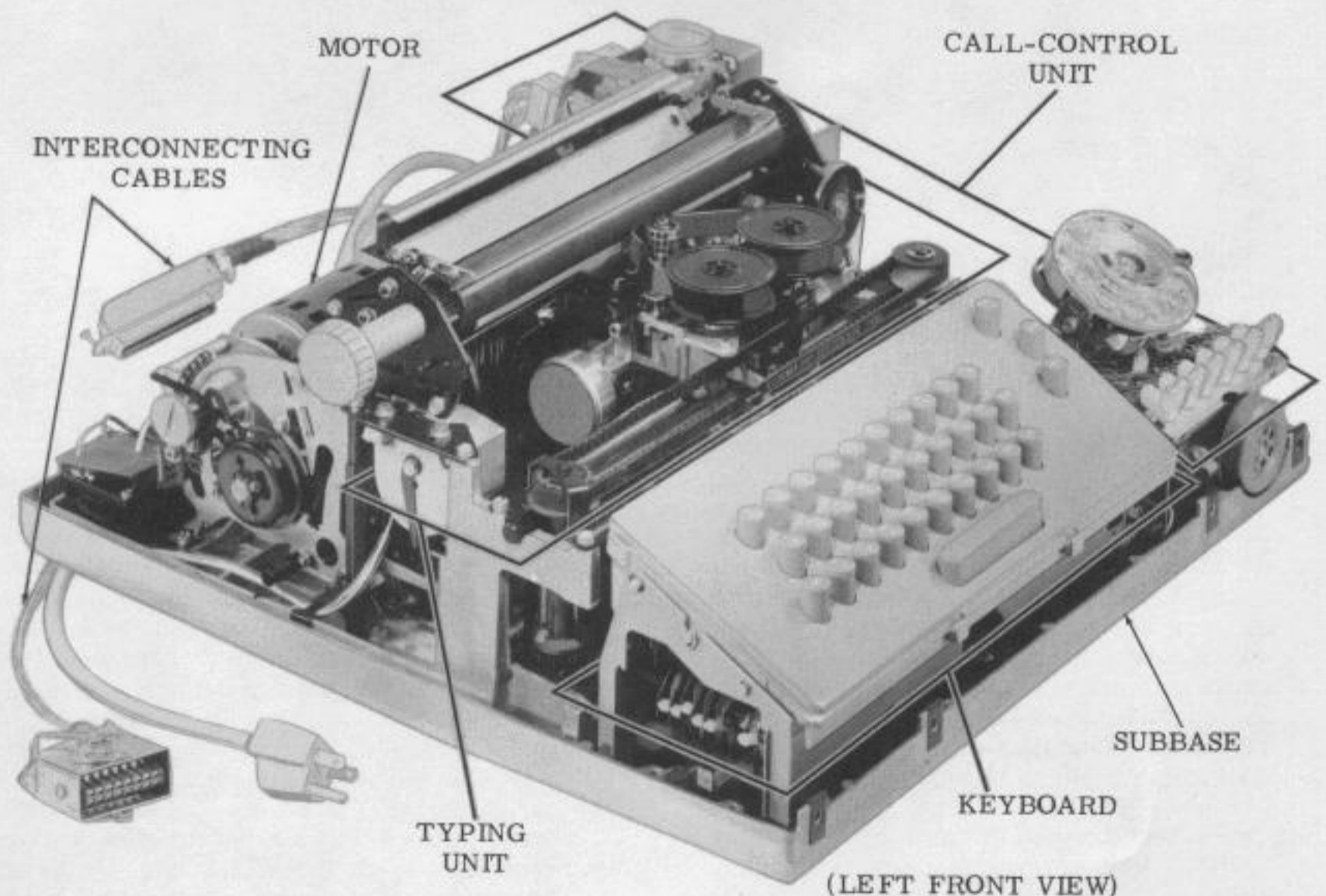
Figure 5 — Keyboard Send-Receive (KSR) Teletypewriter Set (Without Cover)
