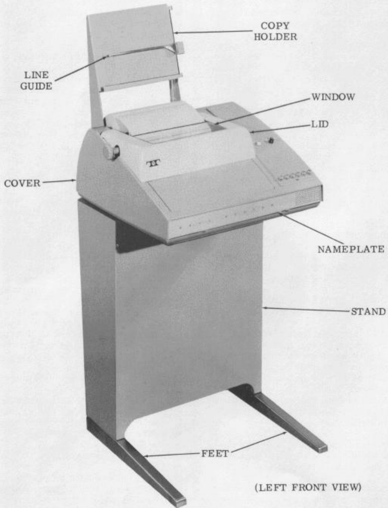
Figure 2 — Receive-Only (RO) Teletypewriter Set
