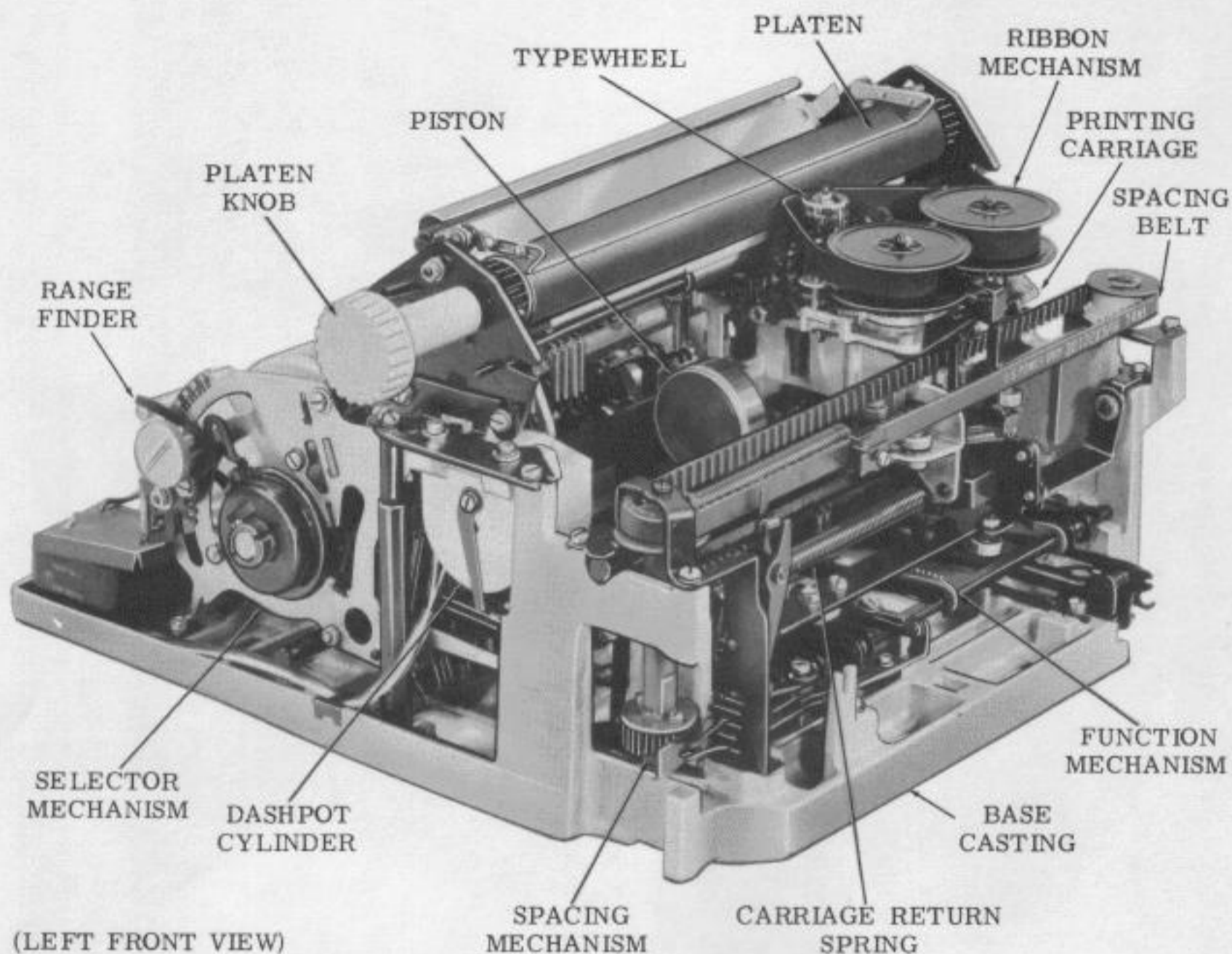
Figure 8 — Typing Unit (Friction Feed)
