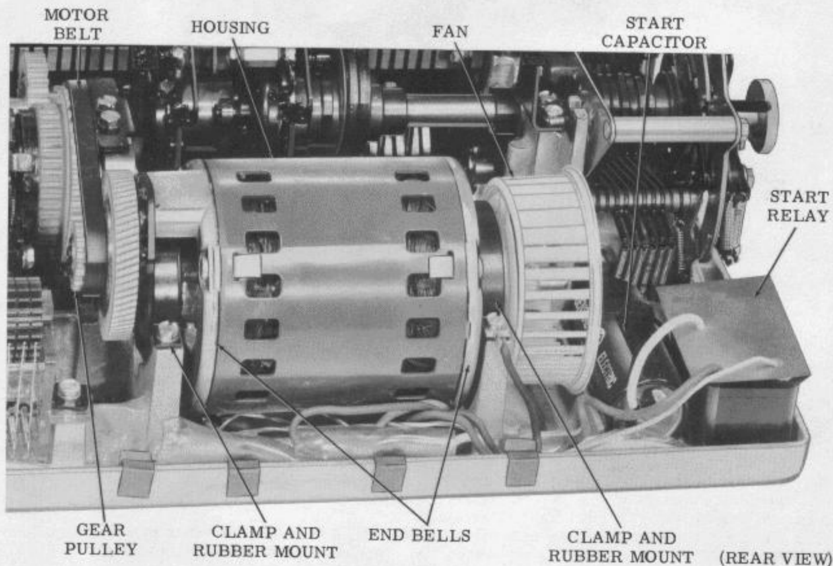
Figure 10 - Motor and Drive Parts
