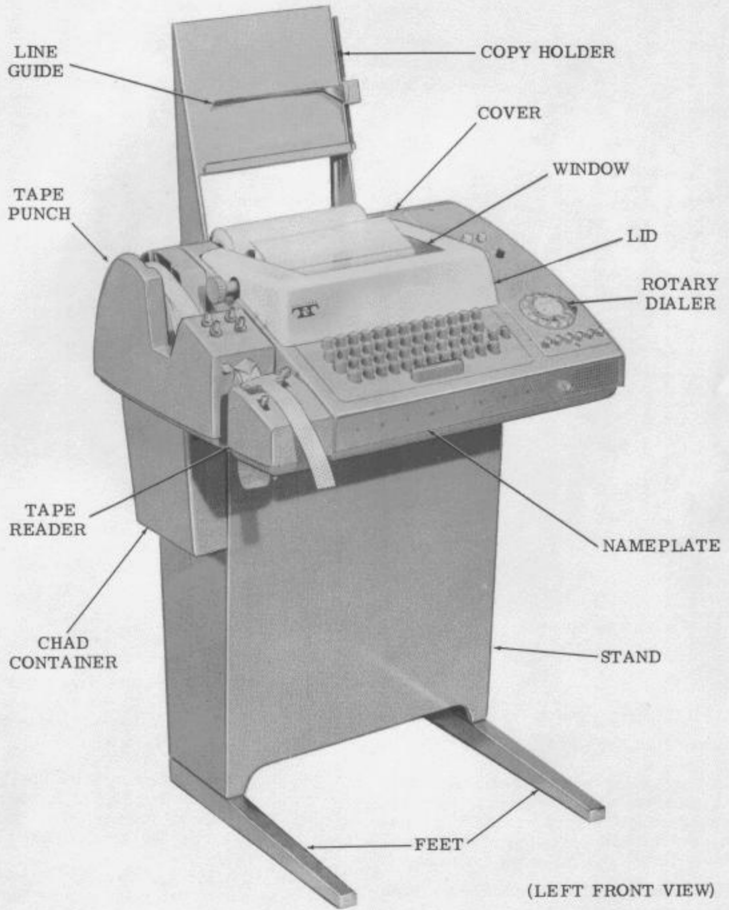
Figure 3 - Automatic Send-Receive (ASR) Teletypewriter Set
