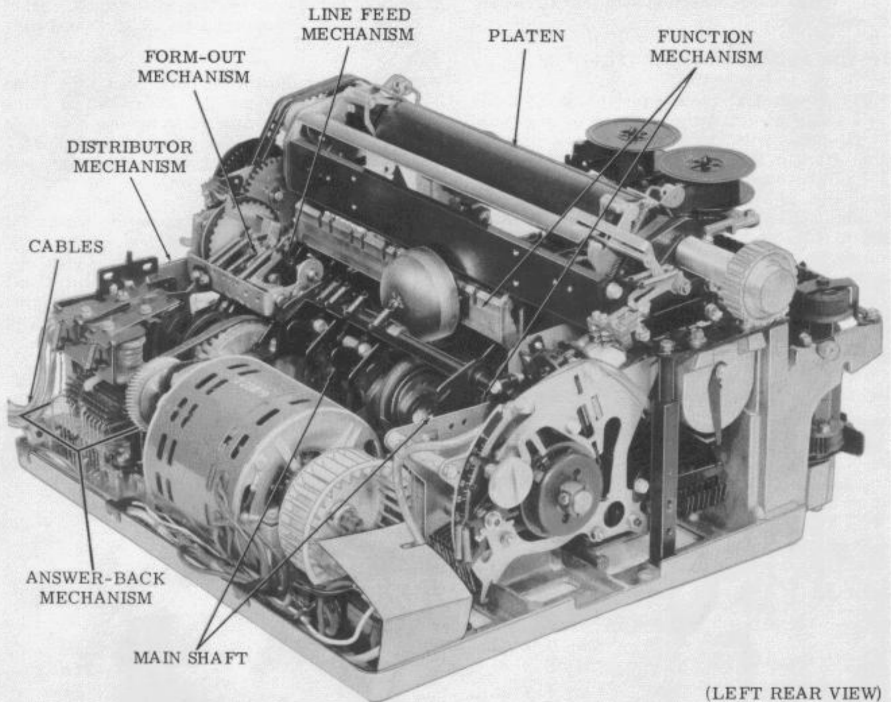
Figure 9 — Typing Unit (Sprocket Feed)
