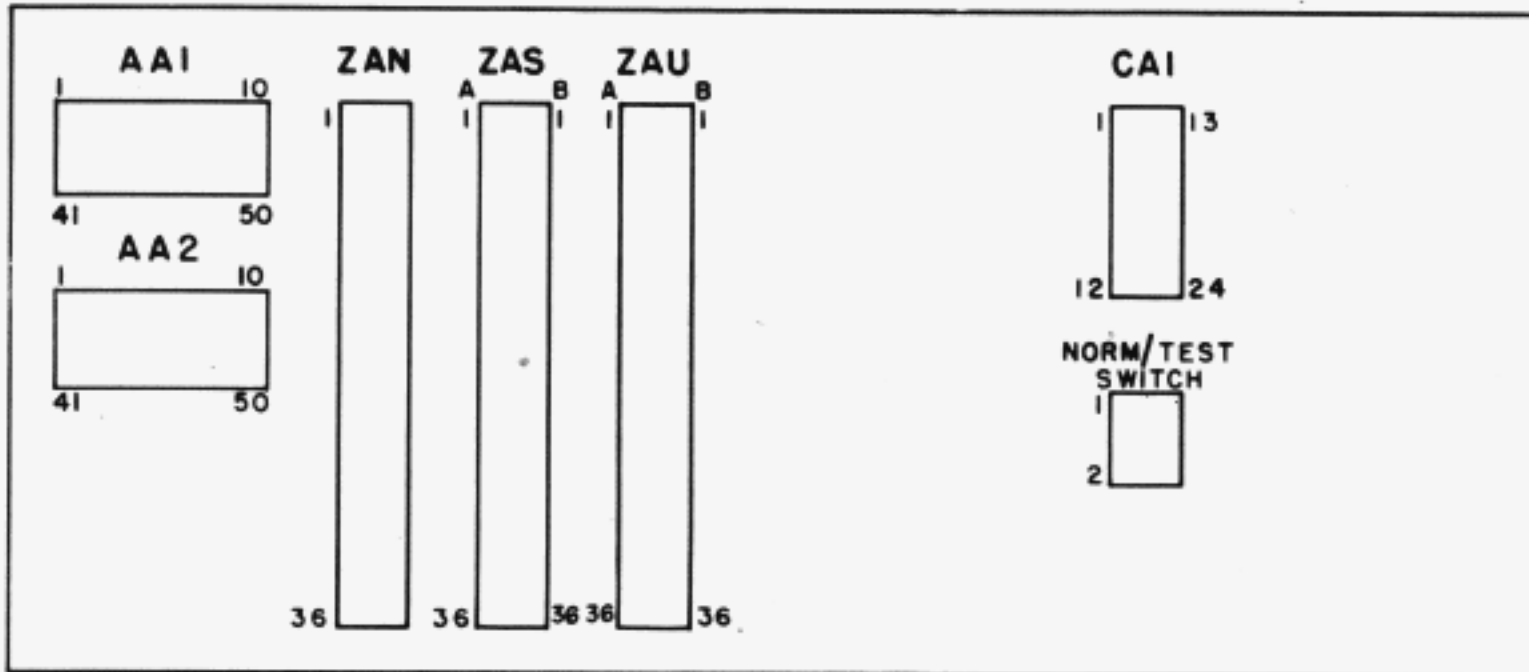
DAIF1 Serial Interface Terminal Location (Wiring Side View)
