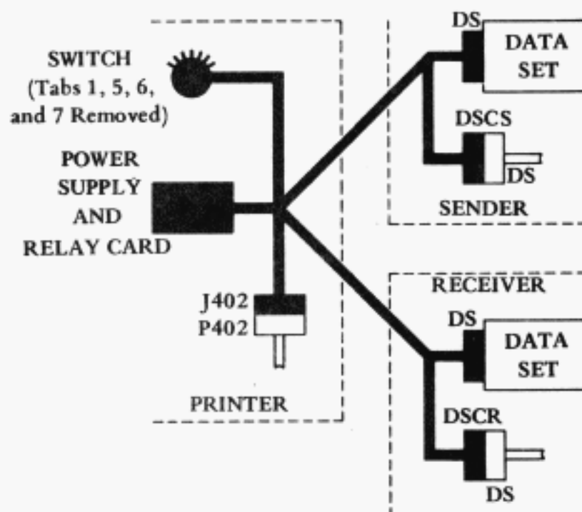
Figure 11 - Connection of INKTRONIC Printer to Type 5 TELESPEED Sender and Receiver
