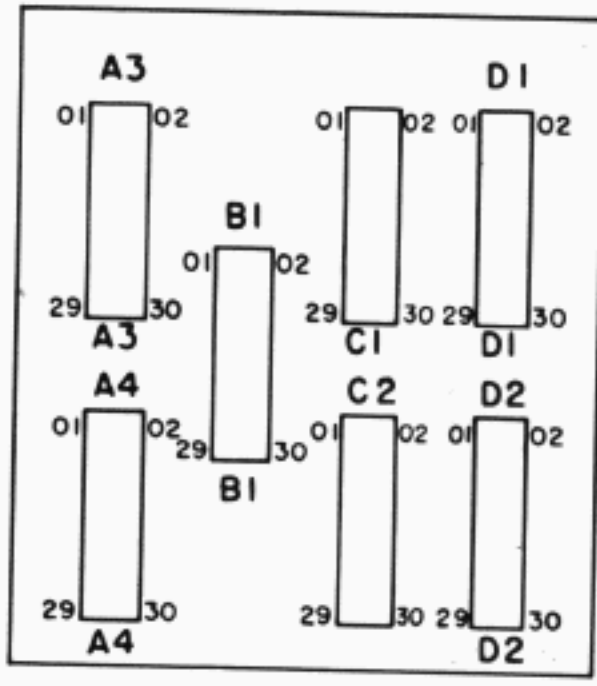
Rear of DAG Cable Connector (Coverplate Removed)
