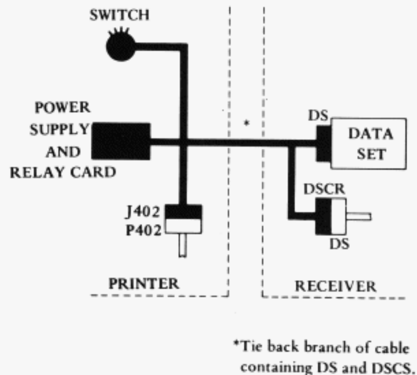
Figure 10 - Connection of INKTRONIC Printer to Type 5 TELESPEED Receiver
