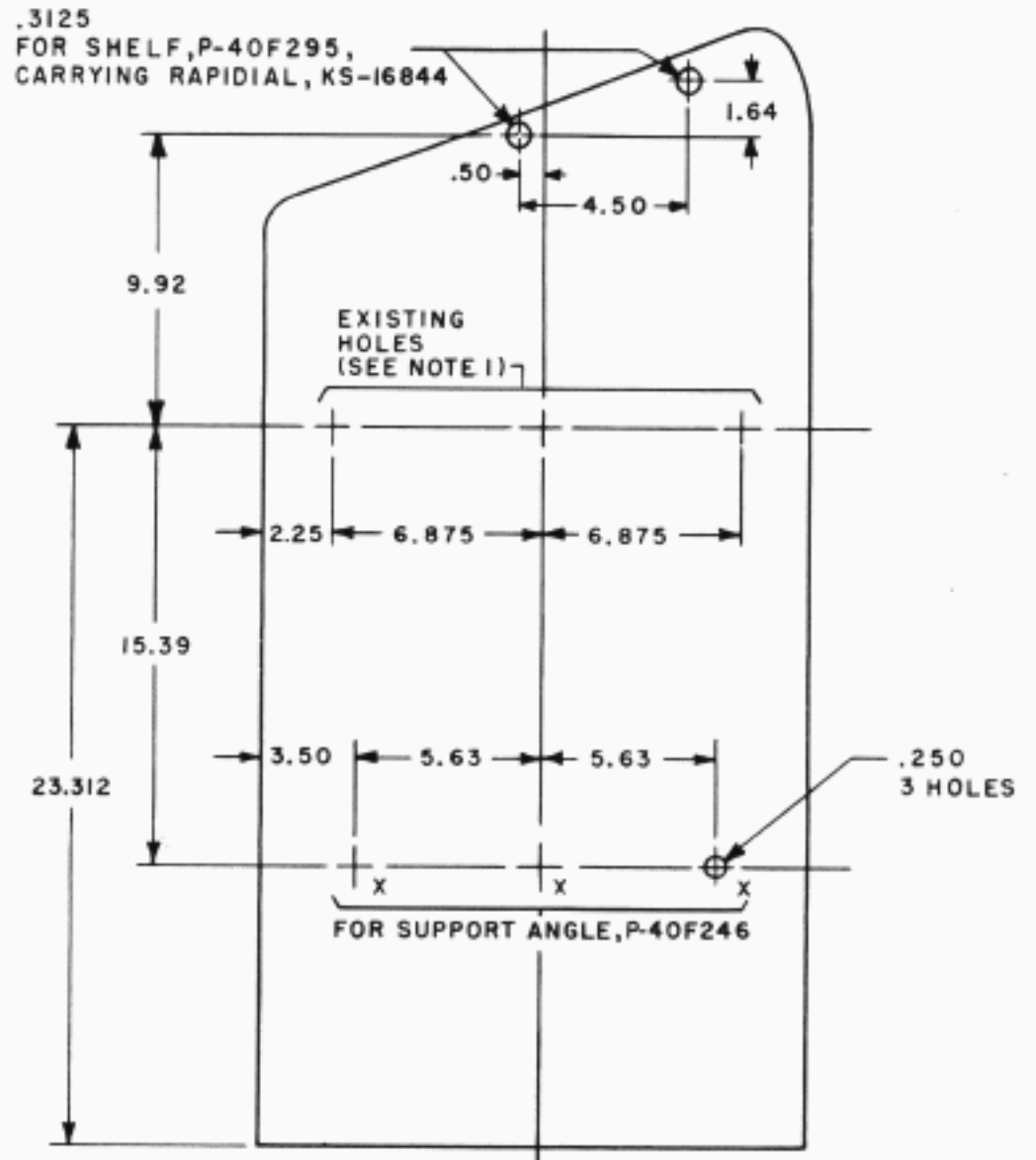
MODIFICATION OF 28 TYPE TTY CABINET TO PROVIDE X HOLES FOR MOUNTING DATA SET IOIA, JIDIOIA, AND RAPIDIAL, KS-16844
