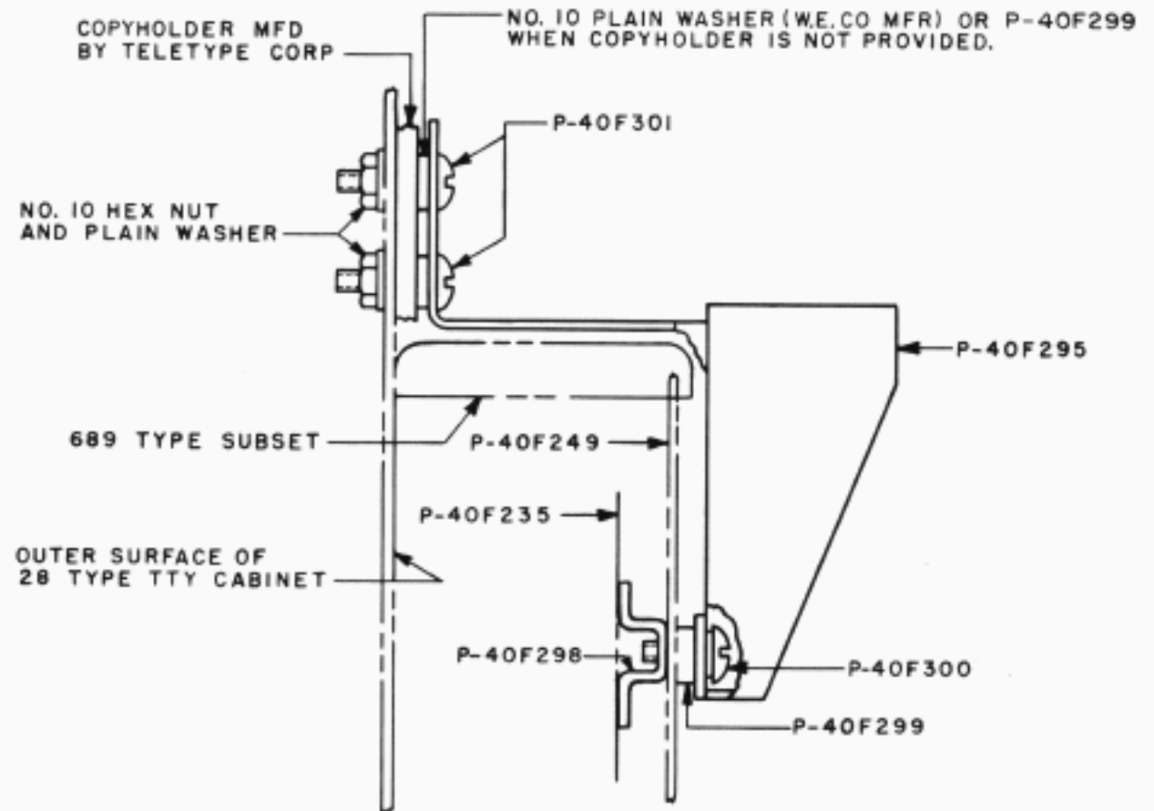
ASSEMBLY OF SHELF, JIDIOIA, L8, TO TELETYPEWRITER CABINET FIG. A
