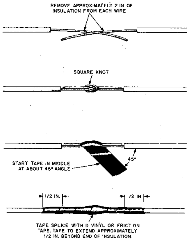
Fig. 5—Repairing Broken Cord
