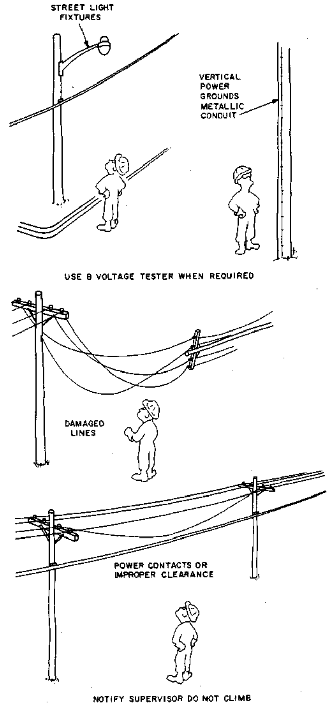
Fig. 6—Visual Inspection for Potential Electrical Hazards
