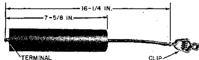
Fig. 3—B-Shunting Capacitor
