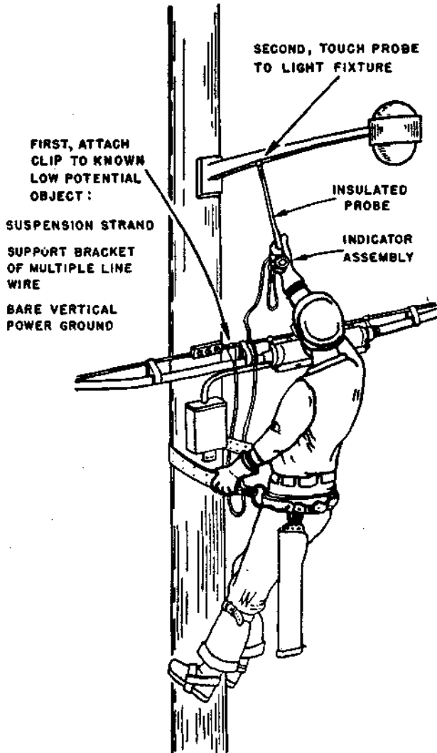
Fig. 11—Testing Street Light Fixture
