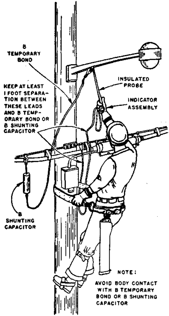
Fig. 12—Use of B-Shunting Capacitor
