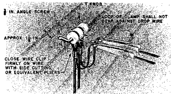
Fig. 1 — Angle Screw
