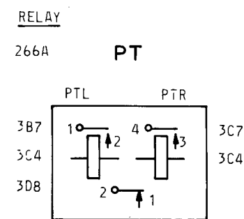
Fig 5L—Method of Showing Individual Relays
