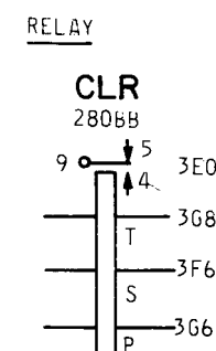
Fig 5L—Method of Showing Individual Relays
