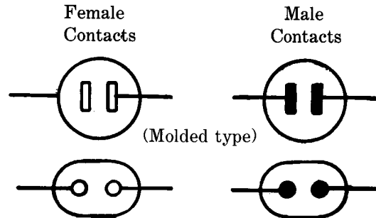
(2) 2-conductor polarized (see preceding note)
