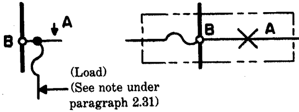
(c) Alarm-type fuse on bus bar
