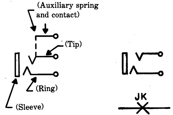
(4) 3-conductor plug
