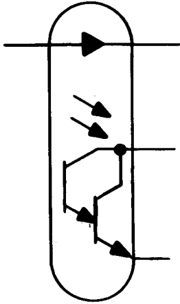
(15) Photo-darlington-detector
