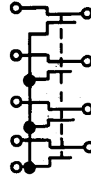
(h) Connectors commonly used for power supply (convenience outlets and mating connectors)
