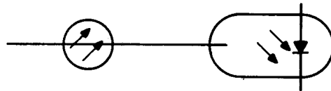
(c) Combined Transmitter-Monitor (Laser - PIN type shown)
