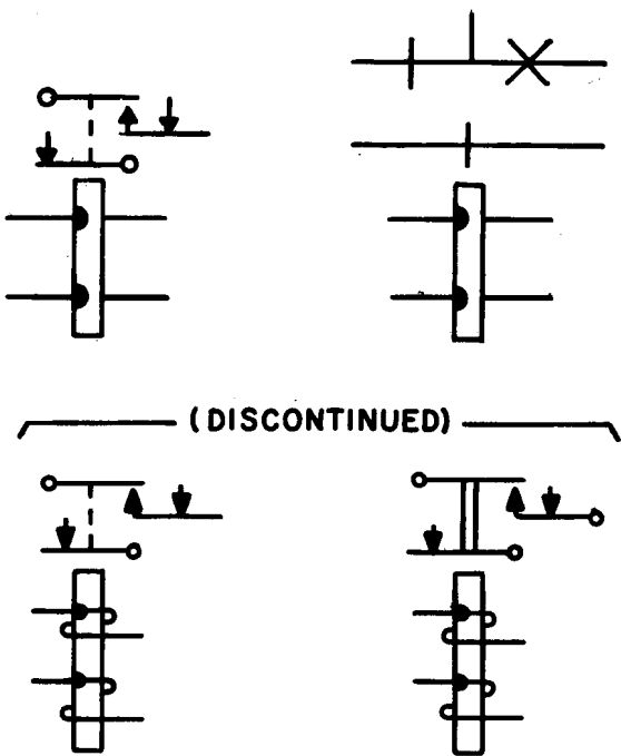
(b) Double-wound relay with break- and make-before-break contacts
