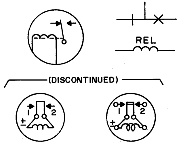
(l) Ammeter-type relay
