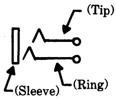
(3) 3-conductor jacks
