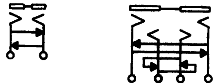
(7) Twin-type jacks
