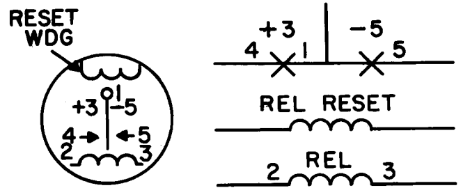
(m) Sensitrol-type relay
