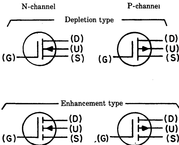
(10) Insulated gate field effect transistors, IGFETs
