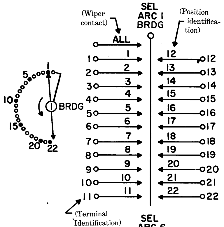
(b) 22-terminal rotary-type selector
