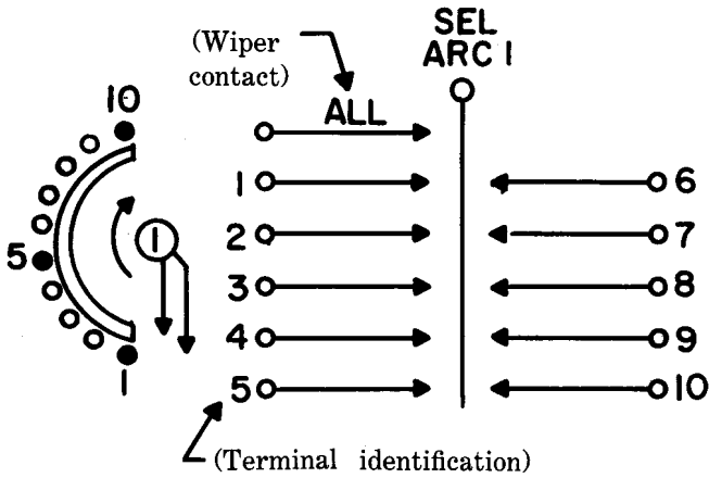
(a) 10-terminal rotary-type selector
