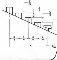
Key dimensions
