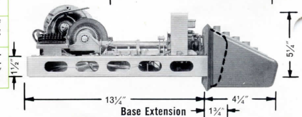
Send-Receive Keyboard — Side view
