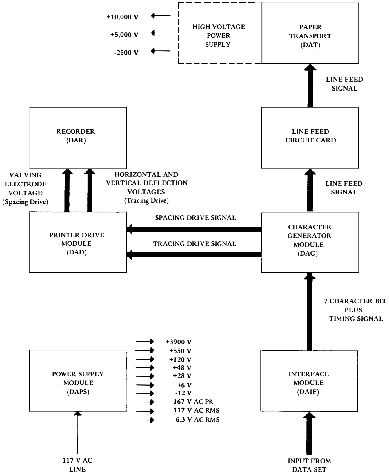
Figure 15 - General Data Flow in DATASPEED Printer
