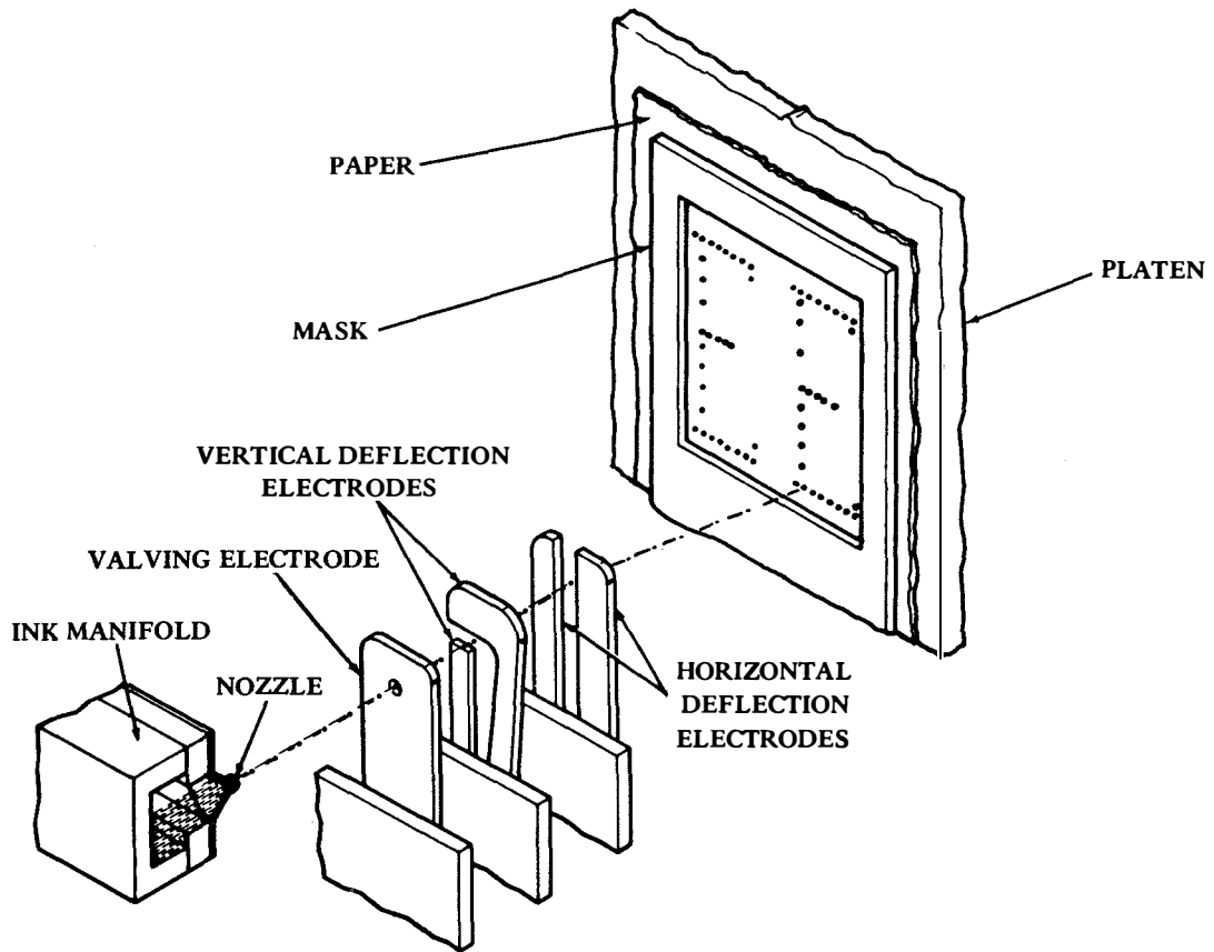
Figure 3 - Ink Manifold, Modulating Electrodes, and Mask Assembly
