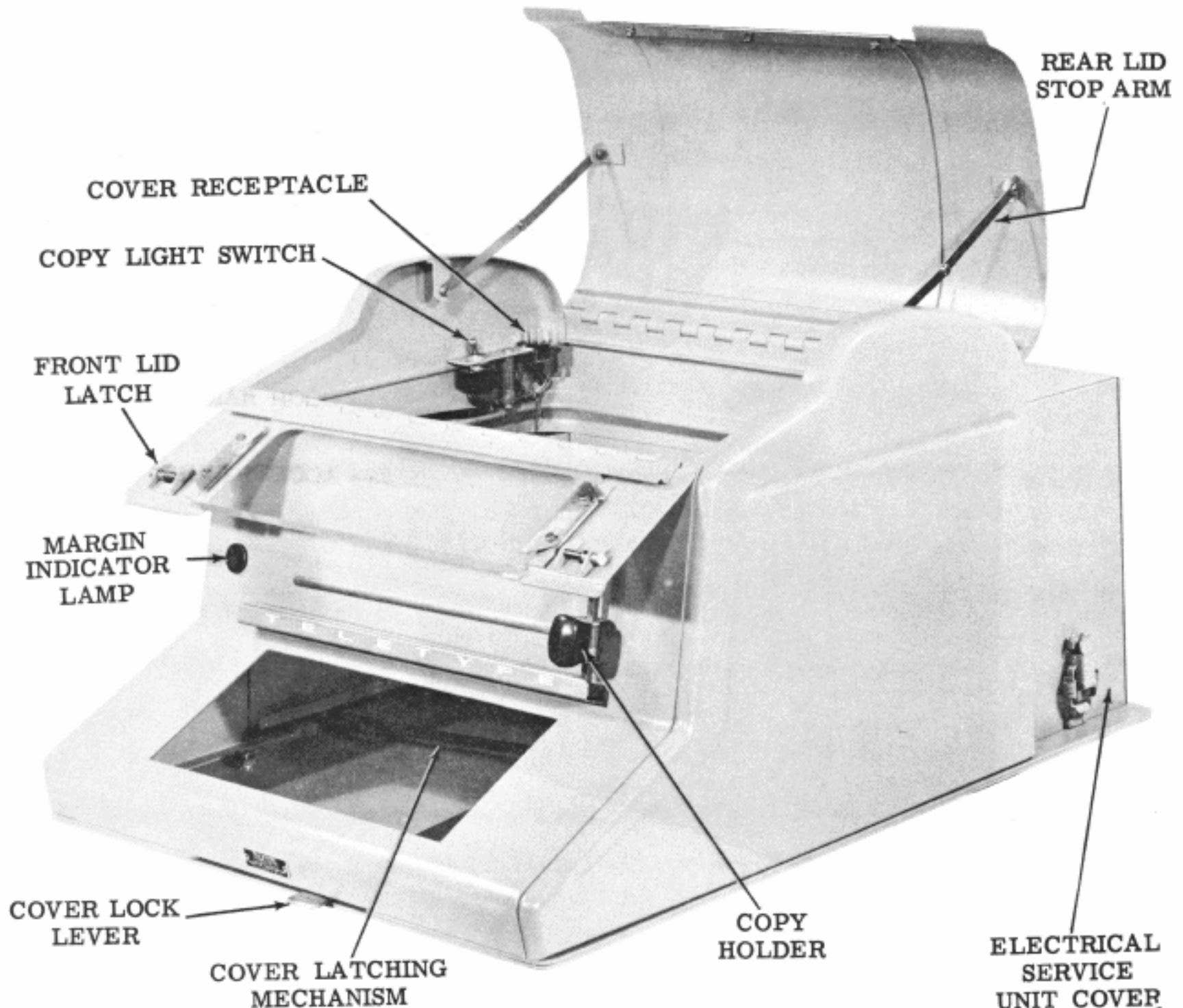
Figure 4 - Rack Mounted Cover
