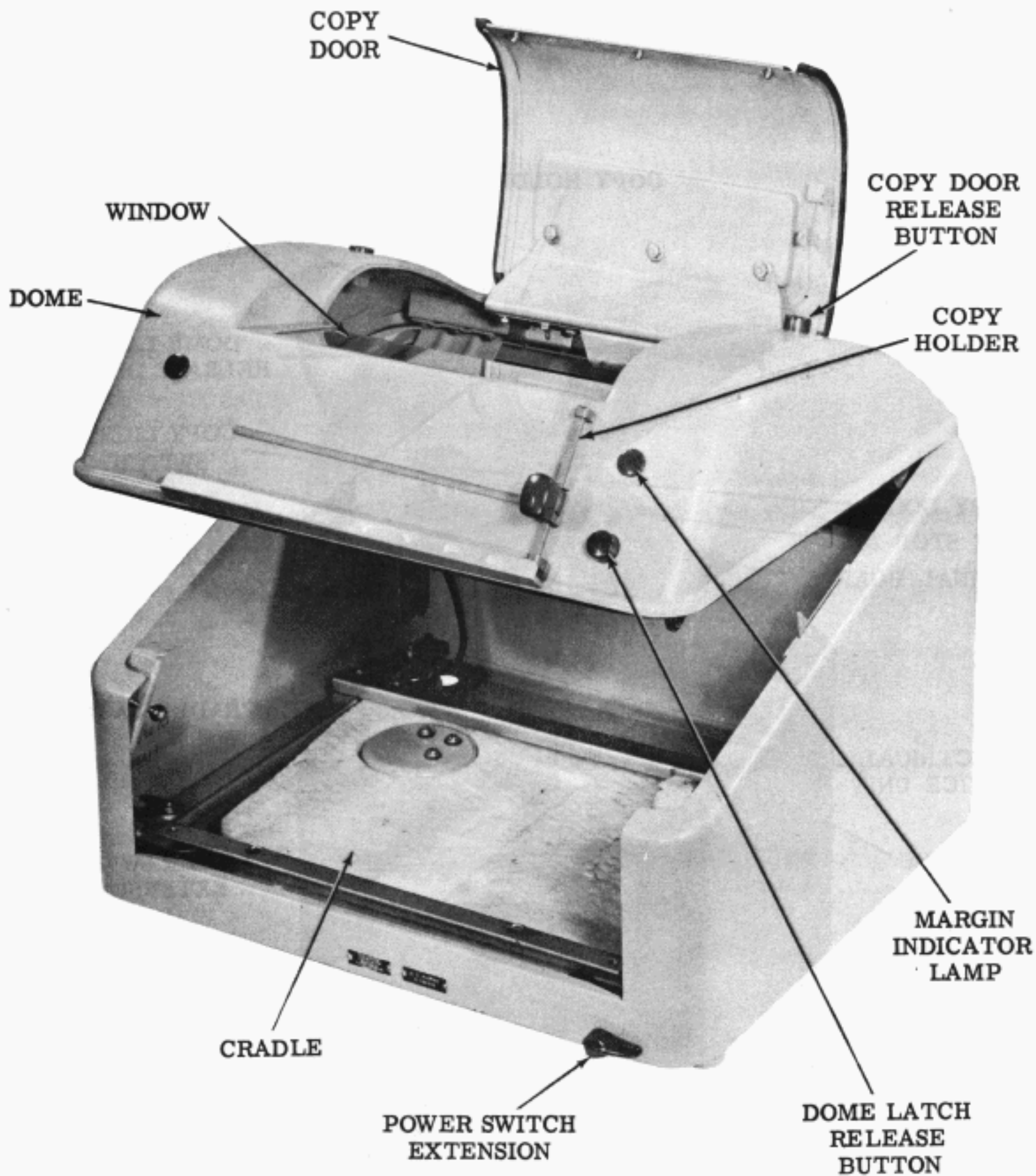
Figure 3 - Table Model Enclosure
