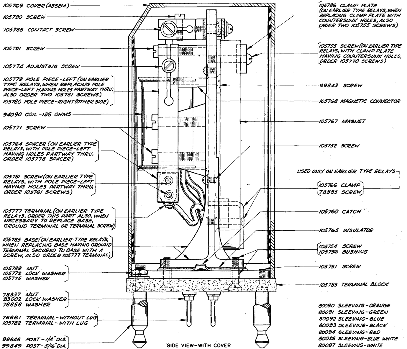
SIDE VIEW - WITH COVER
