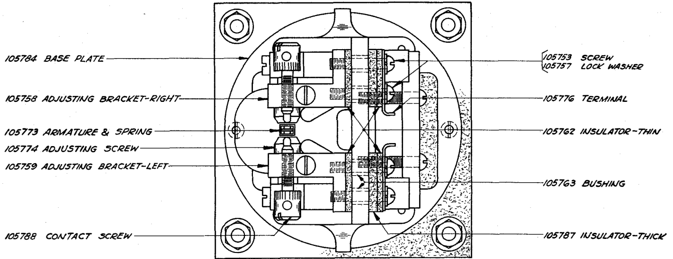
TOP VIEW - COVER REMOVED
