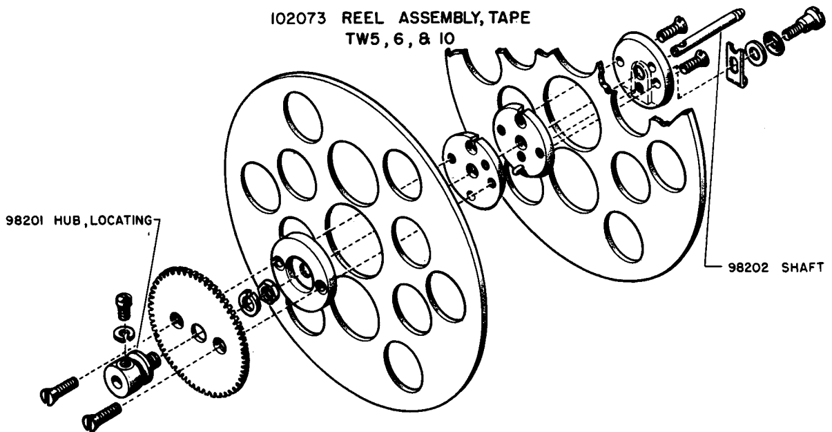
98200 REEL ASSEMBLY, TAPE TW3 & 4
