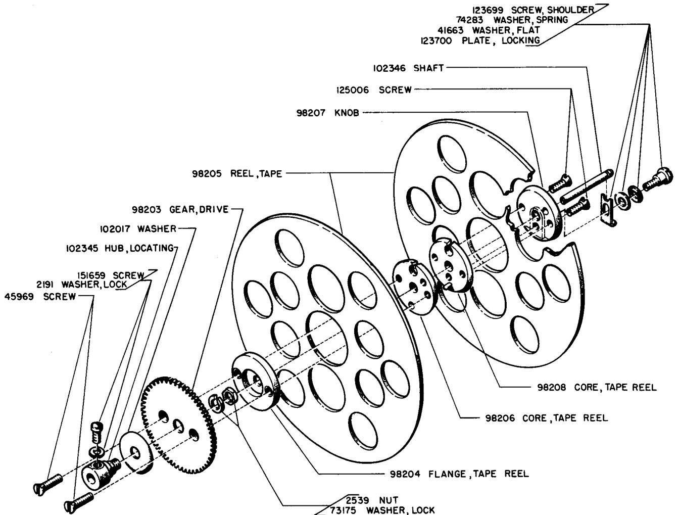
102073 REEL ASSEMBLY, TAPE TW5, 6, & 10
