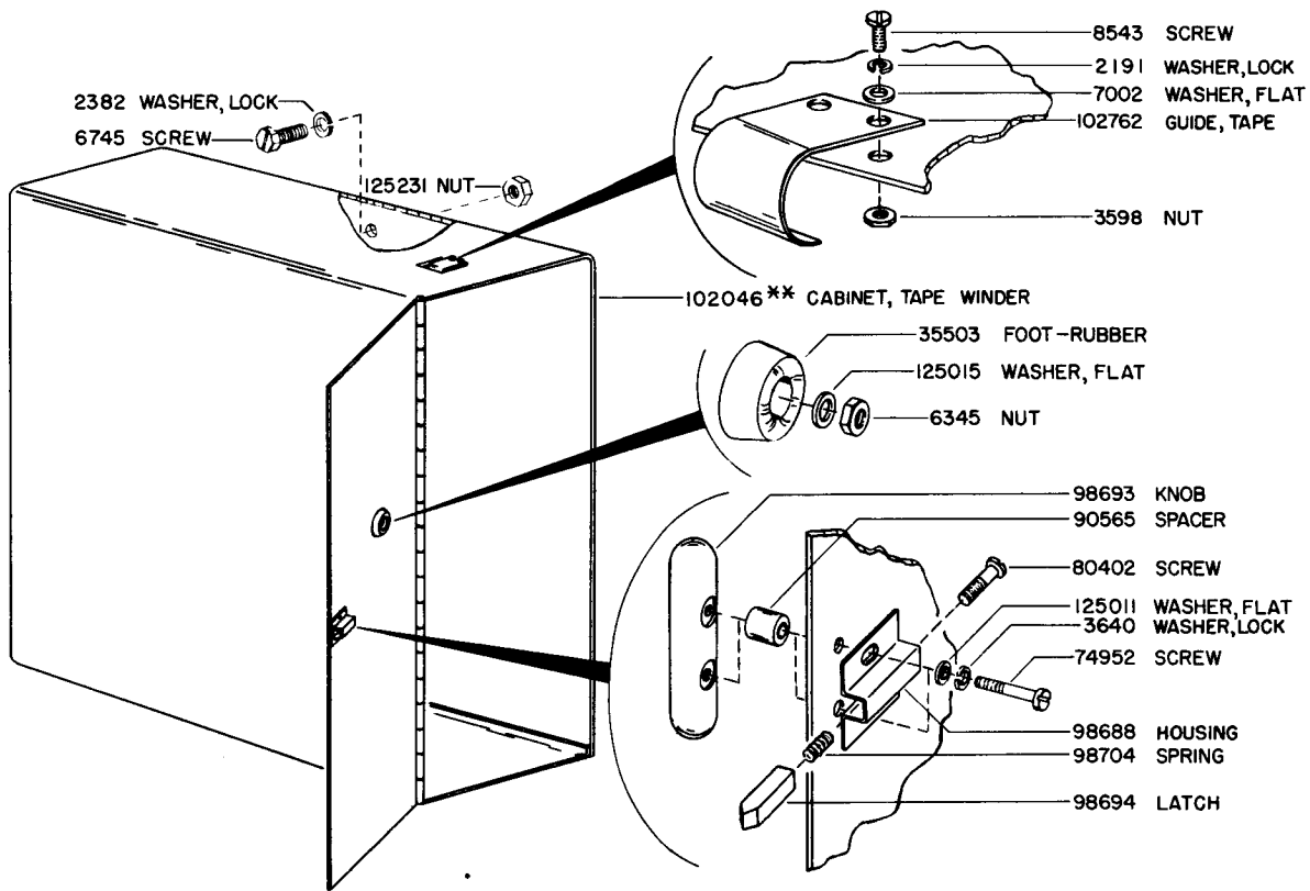
118634** TAPE WINDER CABINET ASSEMBLY
