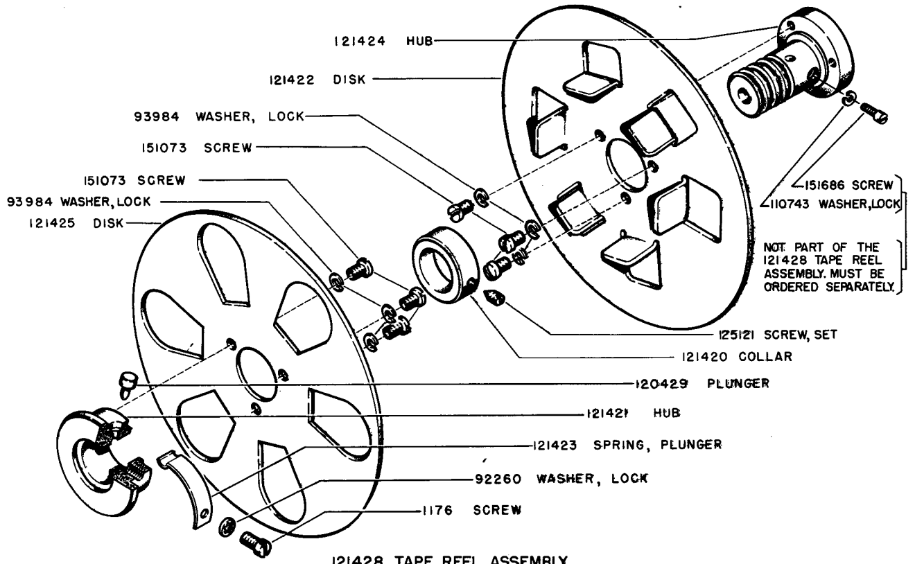
121428 TAPE REEL ASSEMBLY TW200**
