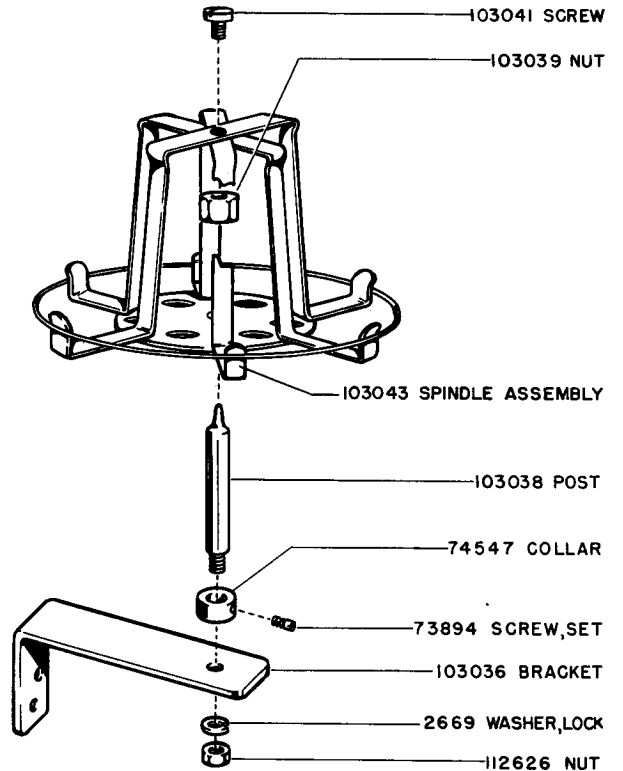
103035 SET OF PARTS FOR APPLYING CENTER UNWIND REEL (USED WITH SPRING DRIVEN TAPE WINDERS)
