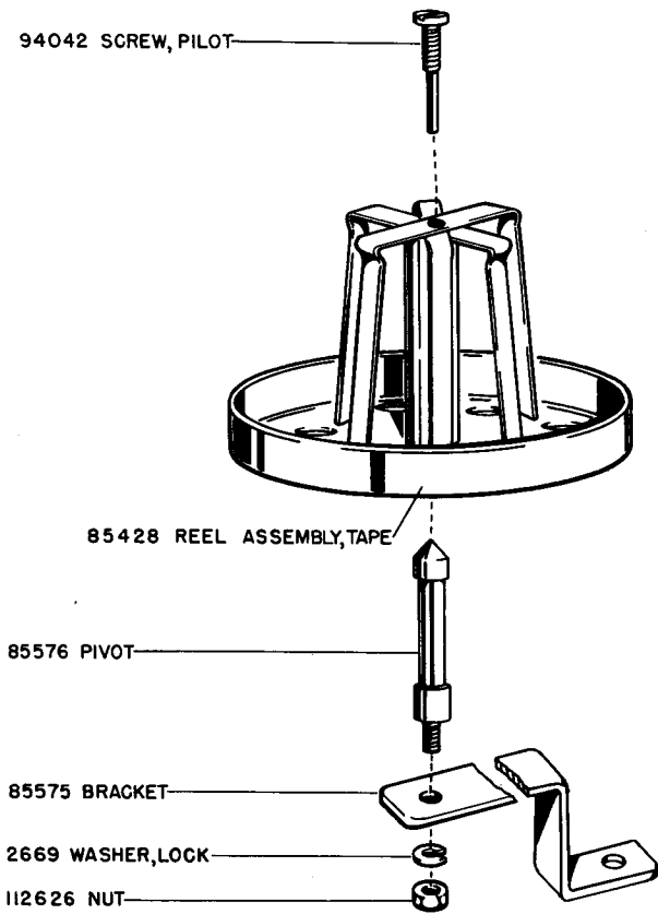
9189 SET OF PARTS FOR APPLYING CENTER UNWIND REEL (USED WITH SPRING DRIVEN TAPE WINDERS)
