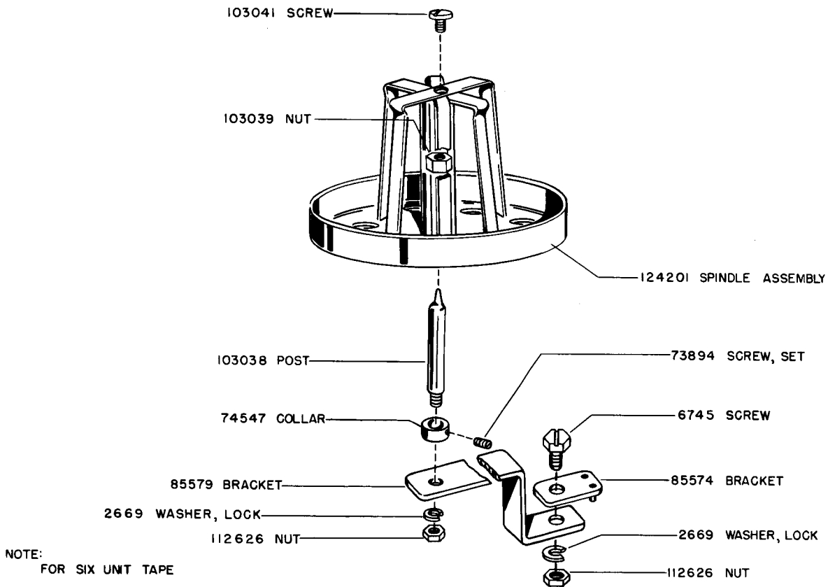
116836 SET OF PARTS FOR APPLYING CENTER UNWIND REEL (USED WITH SPRING DRIVEN TAPE WINDERS) (EXCLUDES PARTS IN FIGURE 5)
