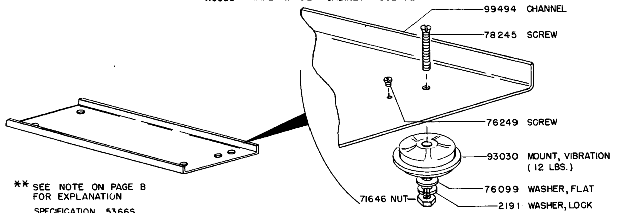
102492 TAPE WINDER MOUNTING CHANNEL ASSEMBLY
