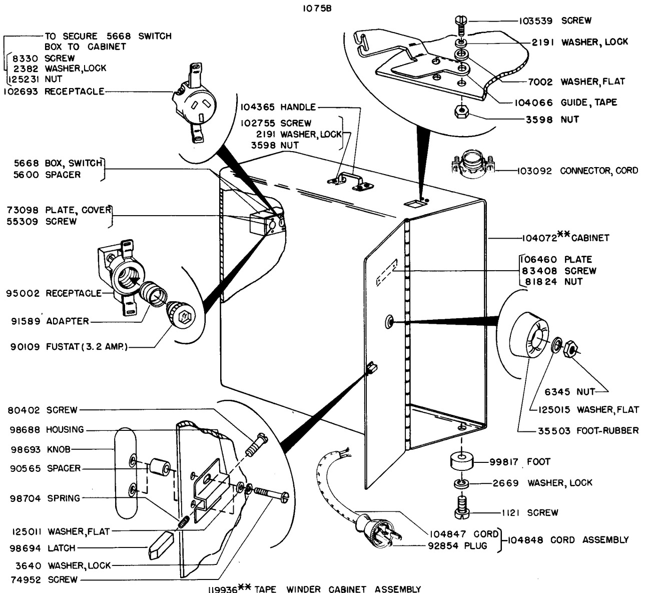
1075B 119936** TAPE WINDER CABINET ASSEMBLY
