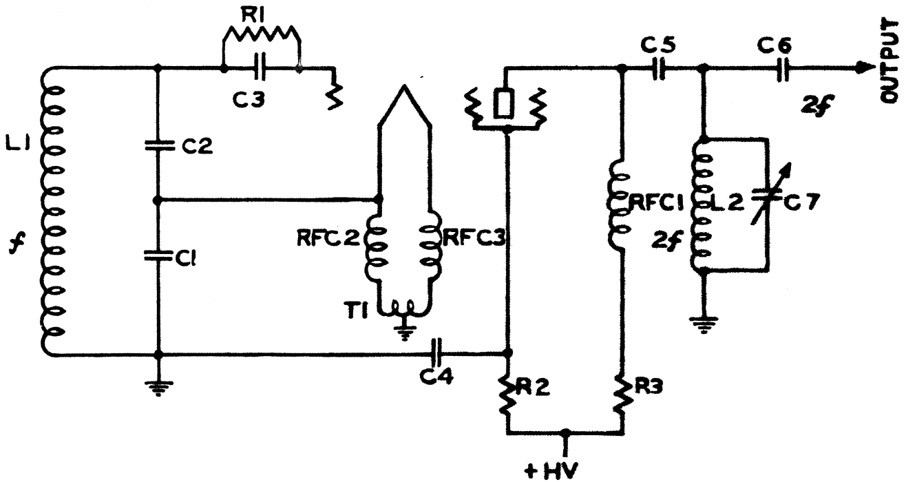
ELECTRON COUPLED OSCILLATOR CIRCUIT
