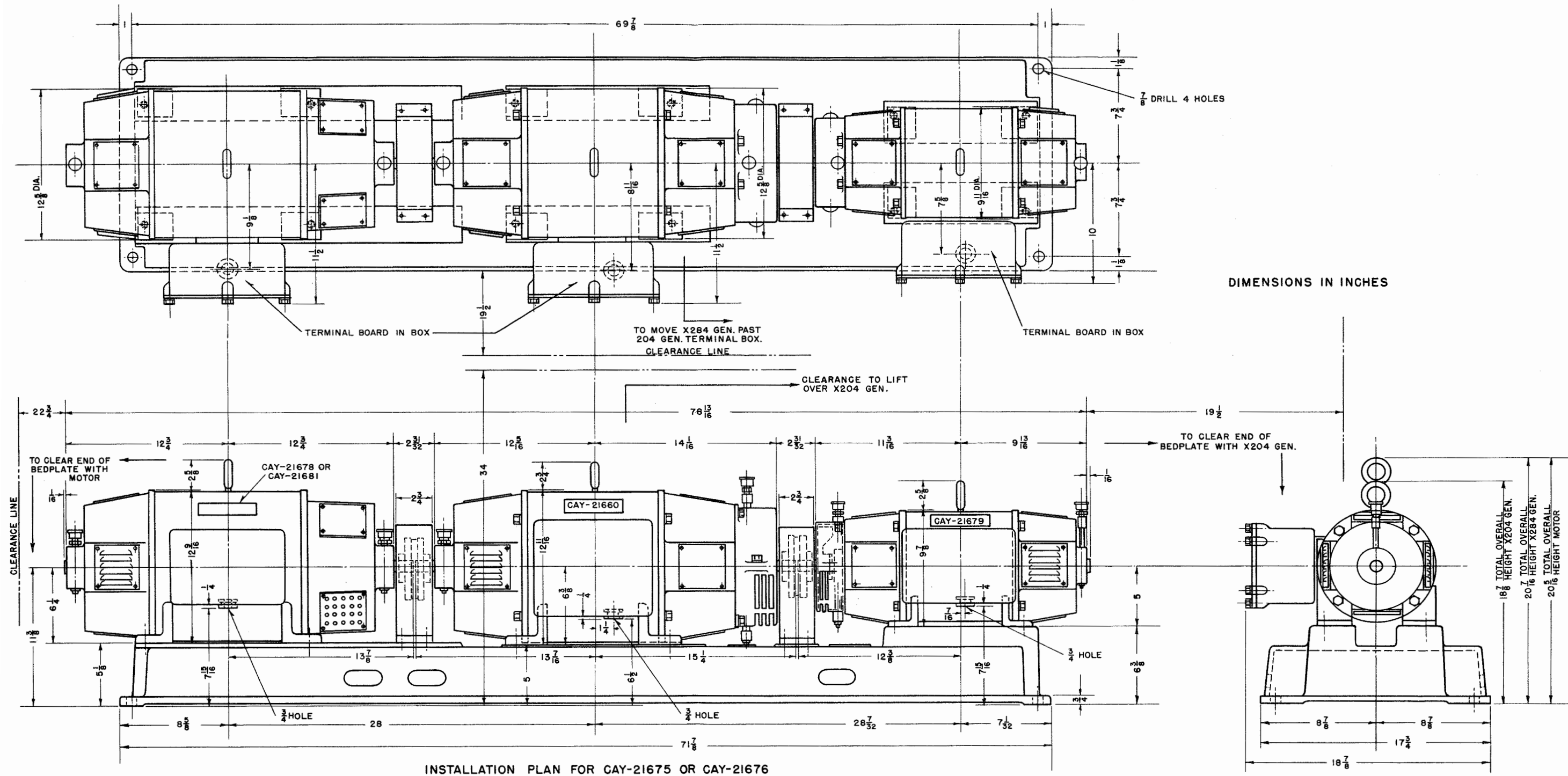
INSTALLATION PLAN FOR CAY-21675 OR CAY-21676
