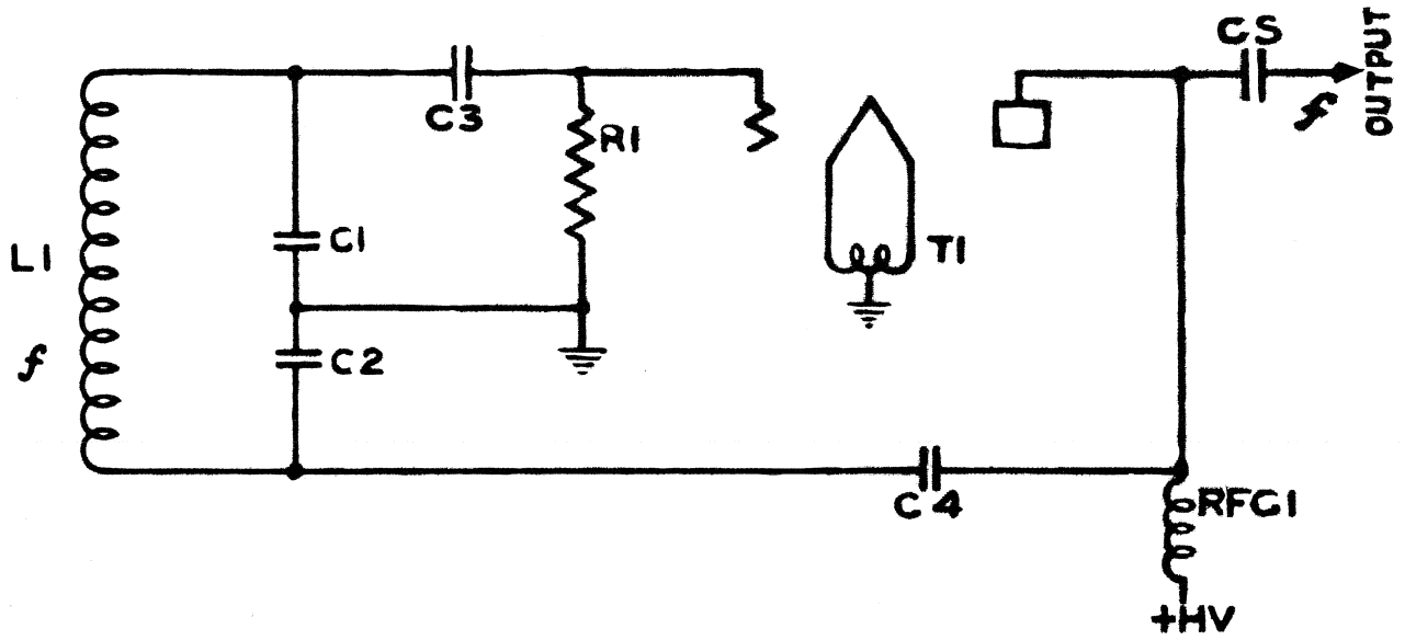
STANDARD COLPITTS OSCILLATOR CIRCUIT
