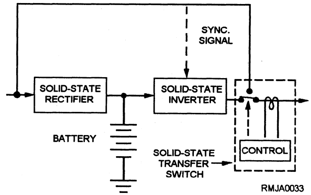
Figure 4-9.—UPS with transfer switch.
