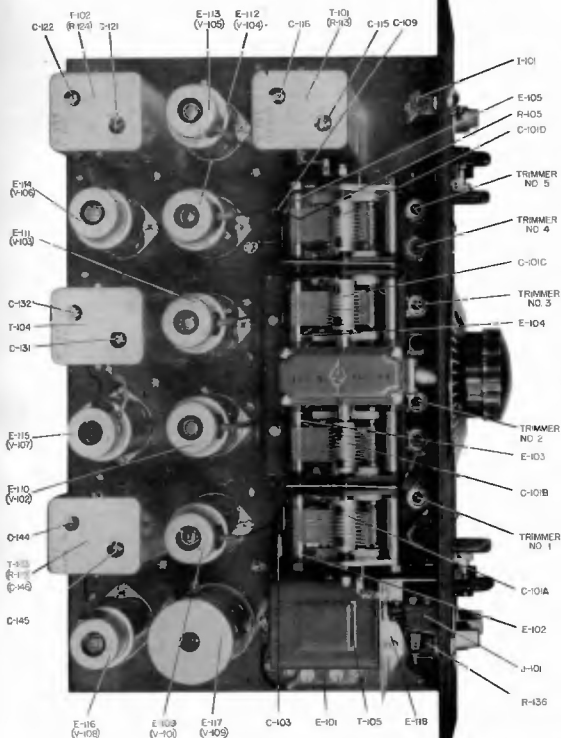
PHOTO NO. 17.18 TOP VIEW OF RADIO RECEIVER
