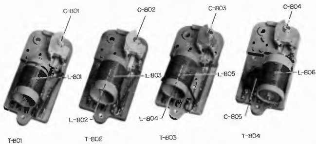
PHOTO NO. 17.10 R.F. TRANSFORMER SET NO. 5
