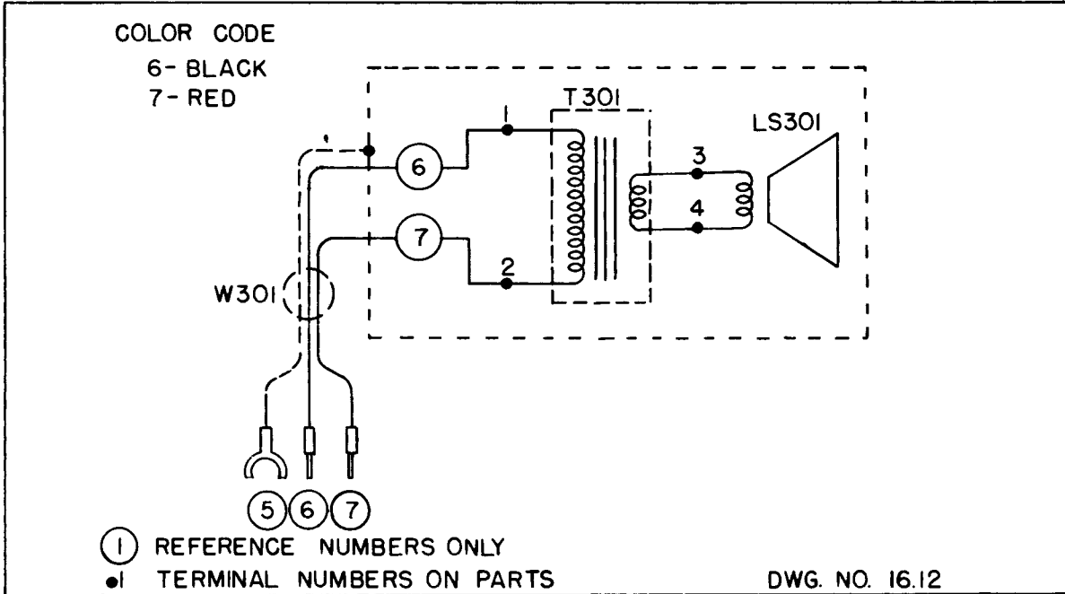
ACTUAL WIRING DIAGRAM TYPES CNA-49105 AND CNA-49106 LOUD SPEAKER UNITS
