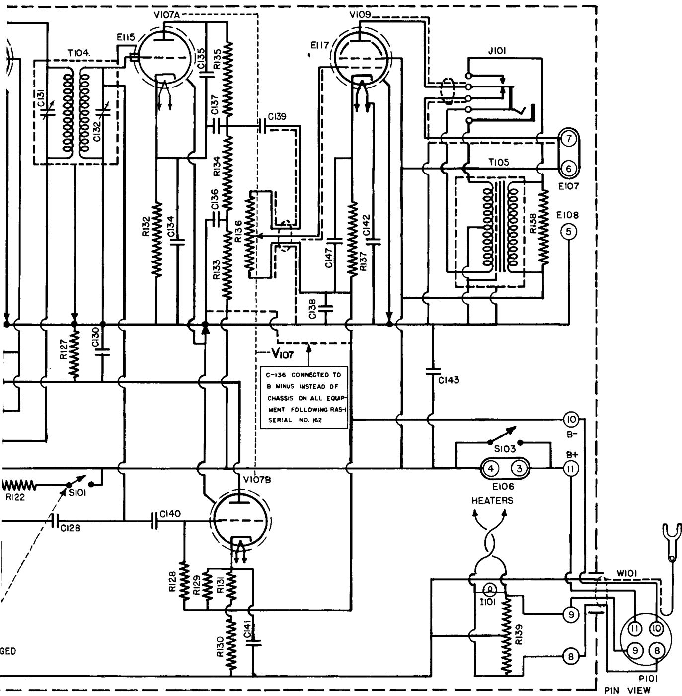
TYPE CNA-46080 RADIO RECEIVER DWG. NO. 16.10
