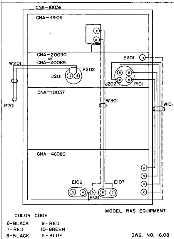
EXTERNAL WIRING CONNECTIONS
