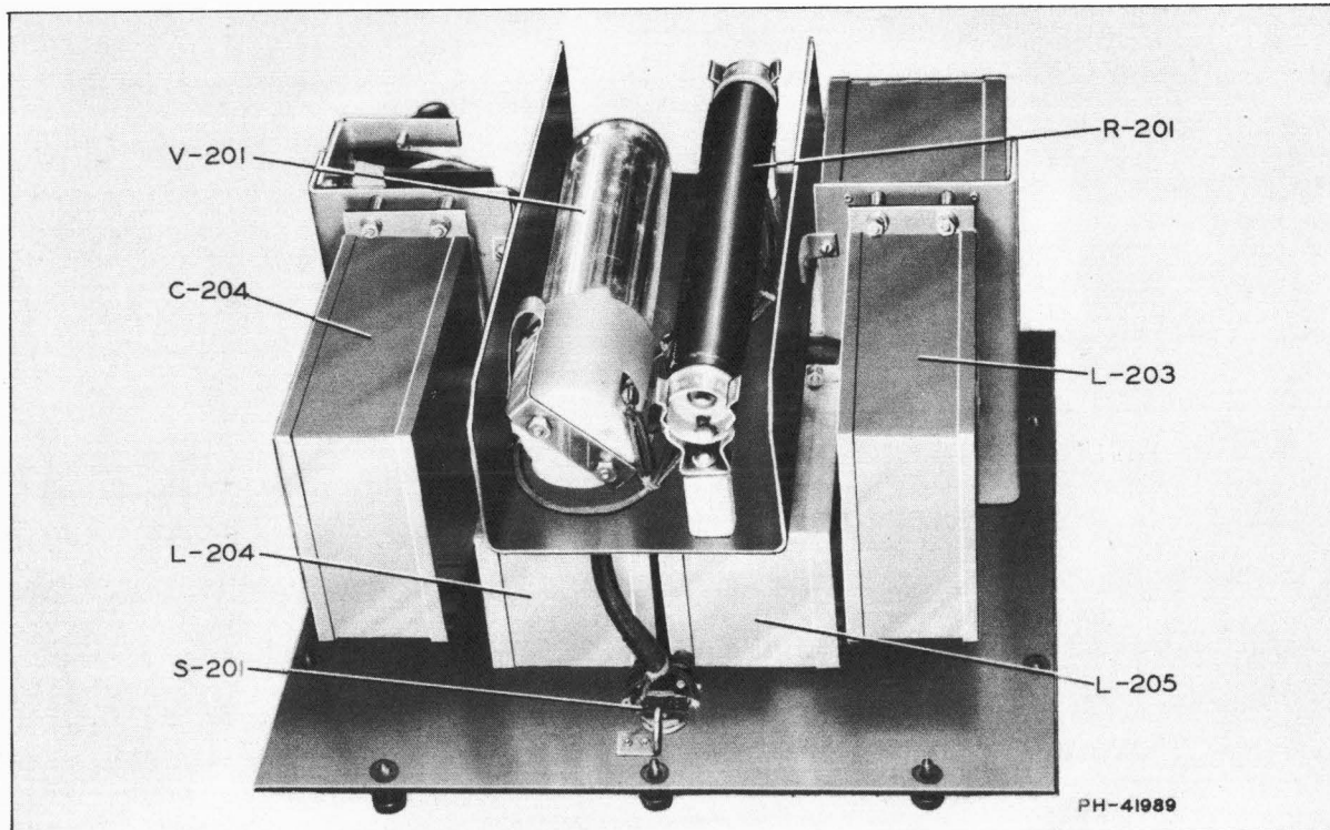
Figure 7—Power Unit CRV-20131 (Bottom View of Chassis)
