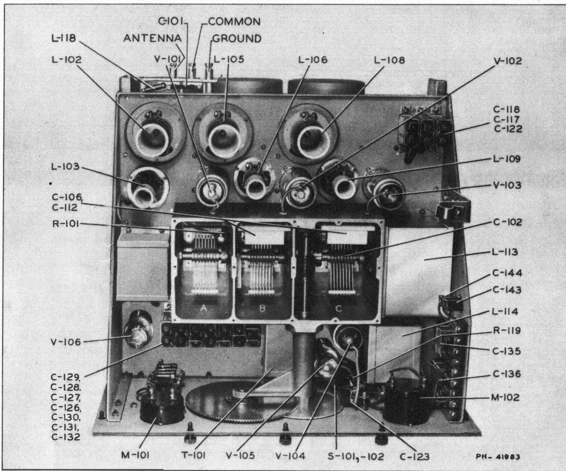
Figure 3—Receiver Unit CRV-46156 (Top View of Chassis—Covers Removed)
