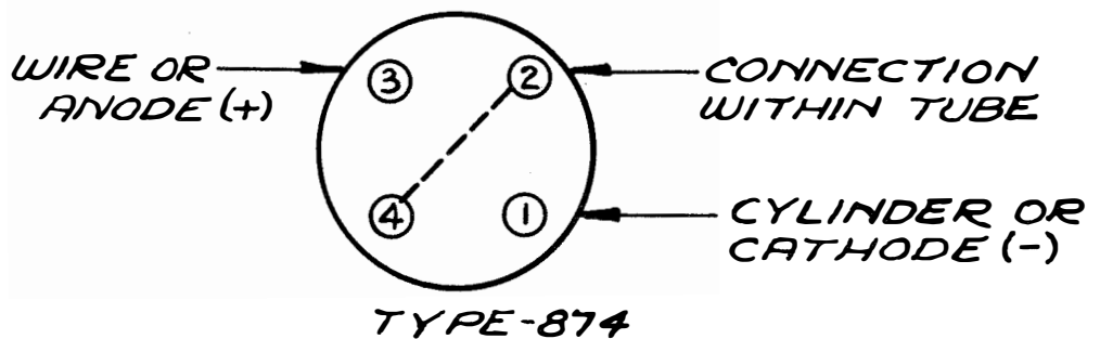
Figure 23—Tube Socket Connections (K-850992)
