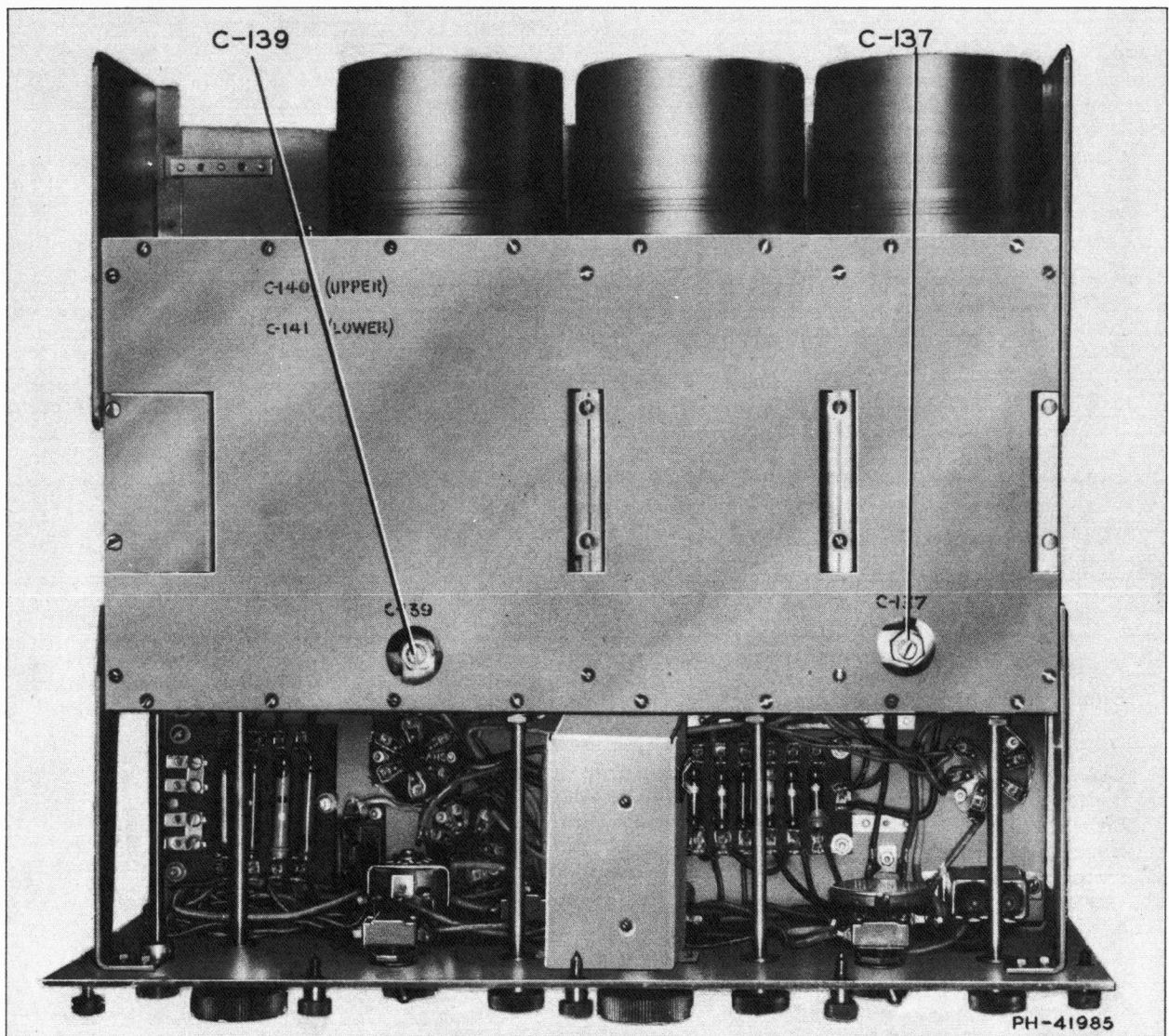
Figure 14—Receiver Unit CRV-46156 (Bottom View of Chassis)
