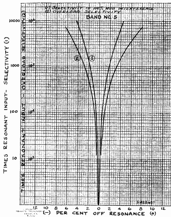
Figure 11—Average Selectivity and Overload Selectivity—Bands 4, 5 and 6 (1) Selectivity to 100% Mod. Interference; (2) Overload Selectivity
