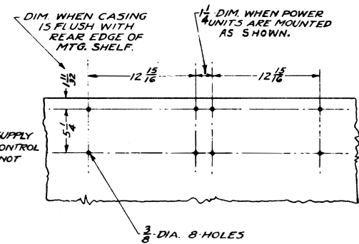
DRILLING PLAN FOR POWER UNITS
