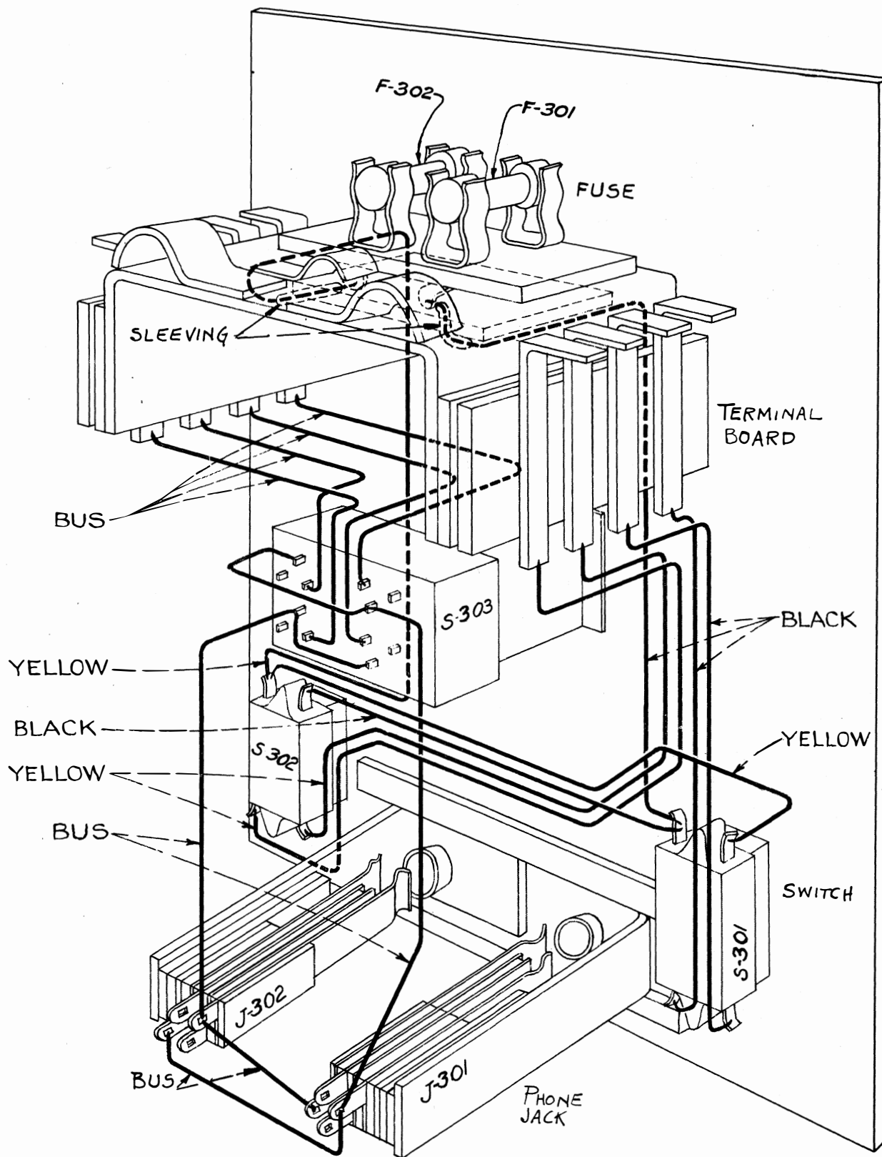
Figure 22—Connection Diagram, Control Unit CRV-23073 (P-714101)
