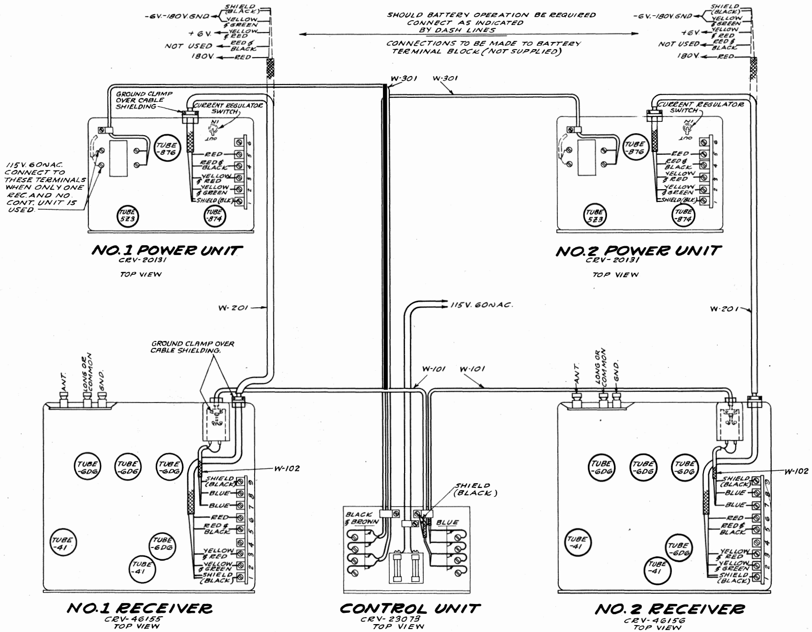
Figure 16—External Cable Connection Diagram (P-721267)
