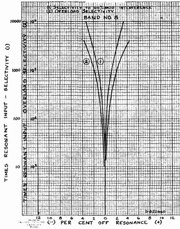
Figure 12—Average Selectivity and Overload Selectivity—Bands 7, 8 and 9 (1) Selectivity to 100% Mod. Interference; (2) Overload Selectivity
