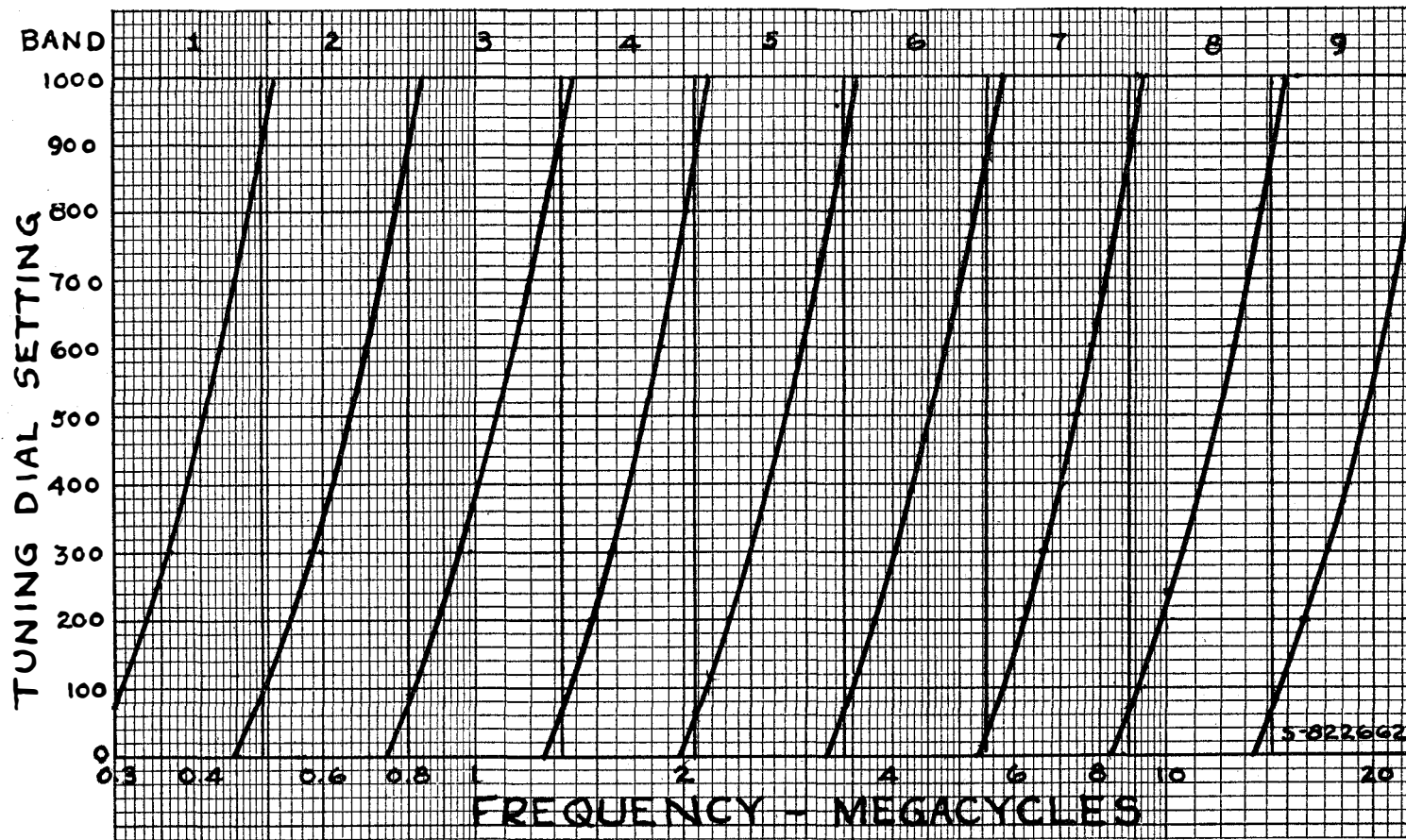
Figure 13—Average Frequency Calibration Curves
