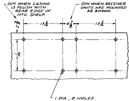
DRILLING PLAN FOR RECEIVER UNITS
