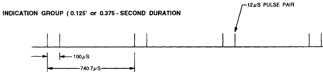
Figure 2-4.—Transponder output pulse train.
