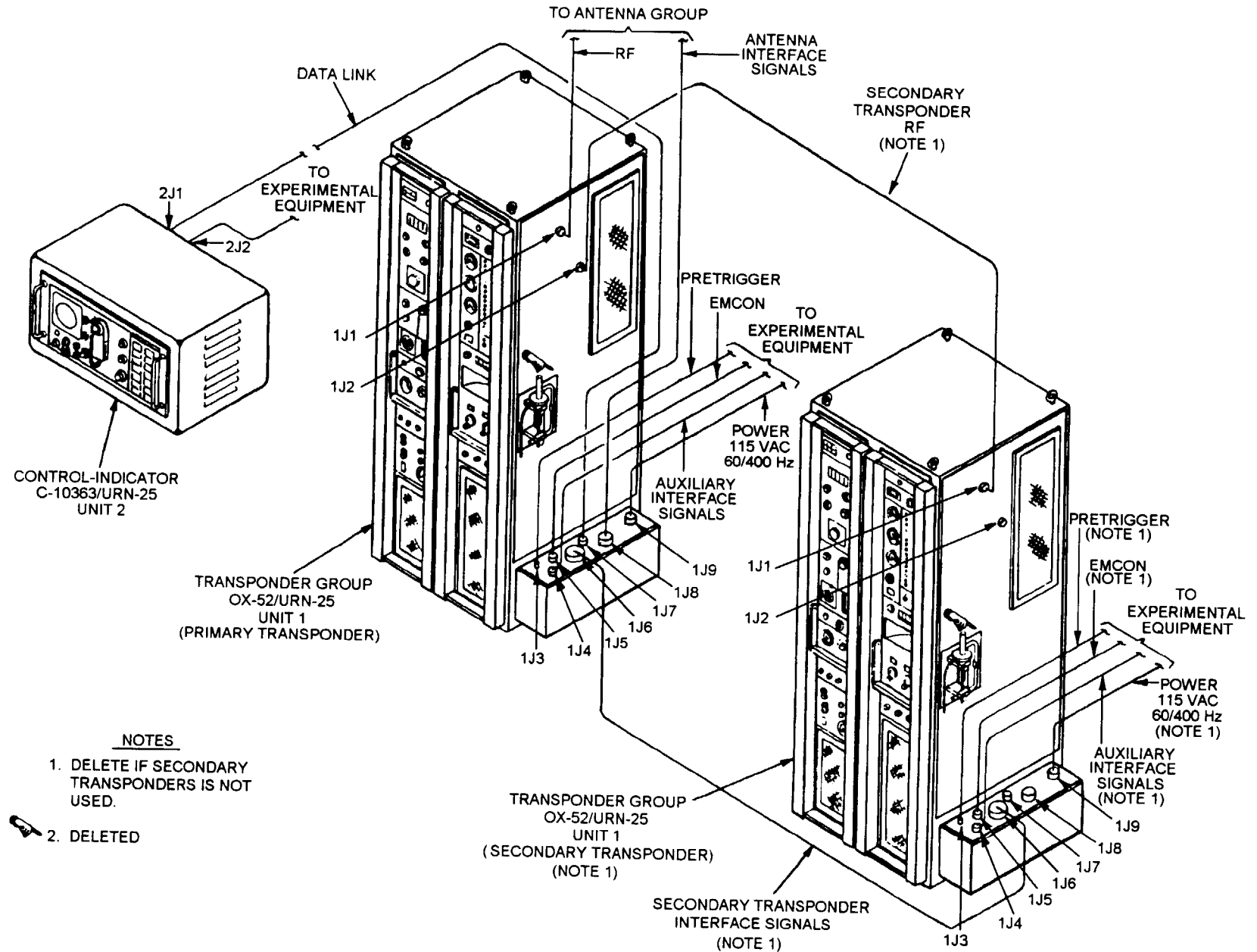
Figure 2-7.-TACAN Set AN/URN-25.
