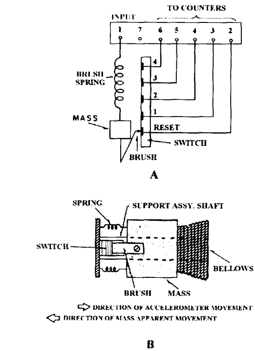
Figure 1-3.—Pulse counting accelerometer.
