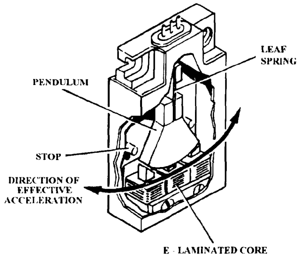
Figure 1-2.—E-transformer accelerometer.
