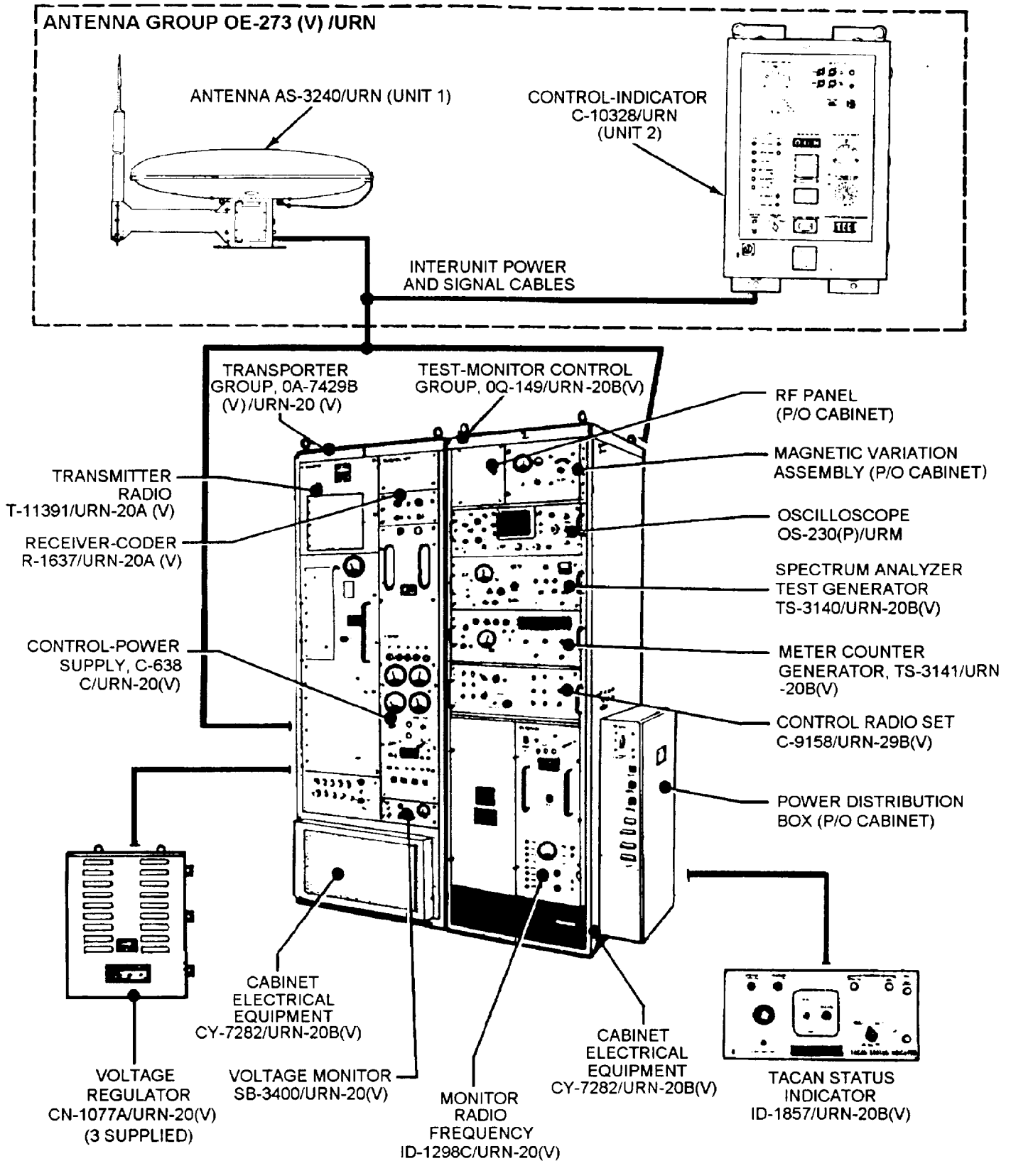
Figure 2-9.—TACAN Set AN/URN-20(V)1.
