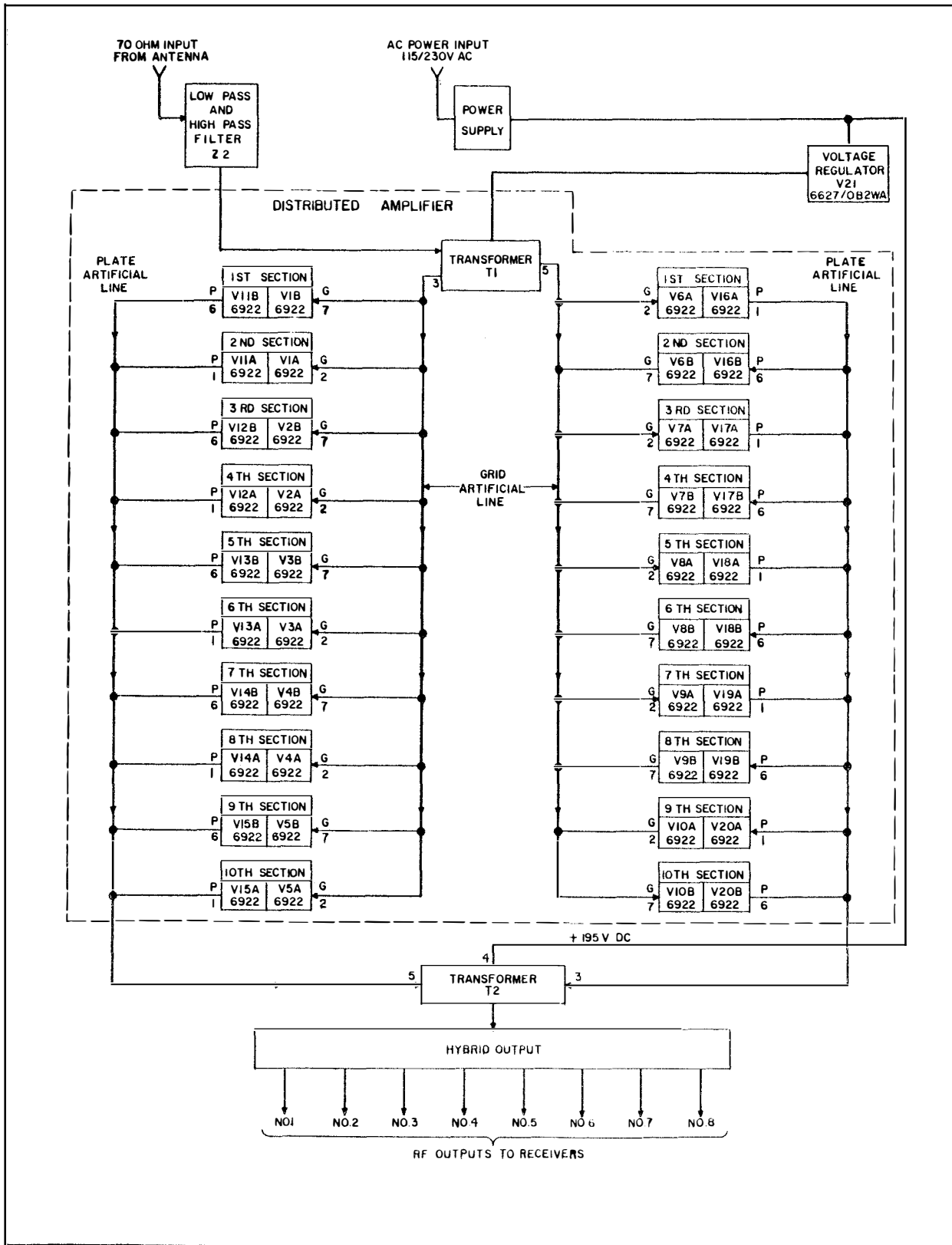
Figure 4-1. Antenna Coupler CU-872/U, Functional Block Diagram
