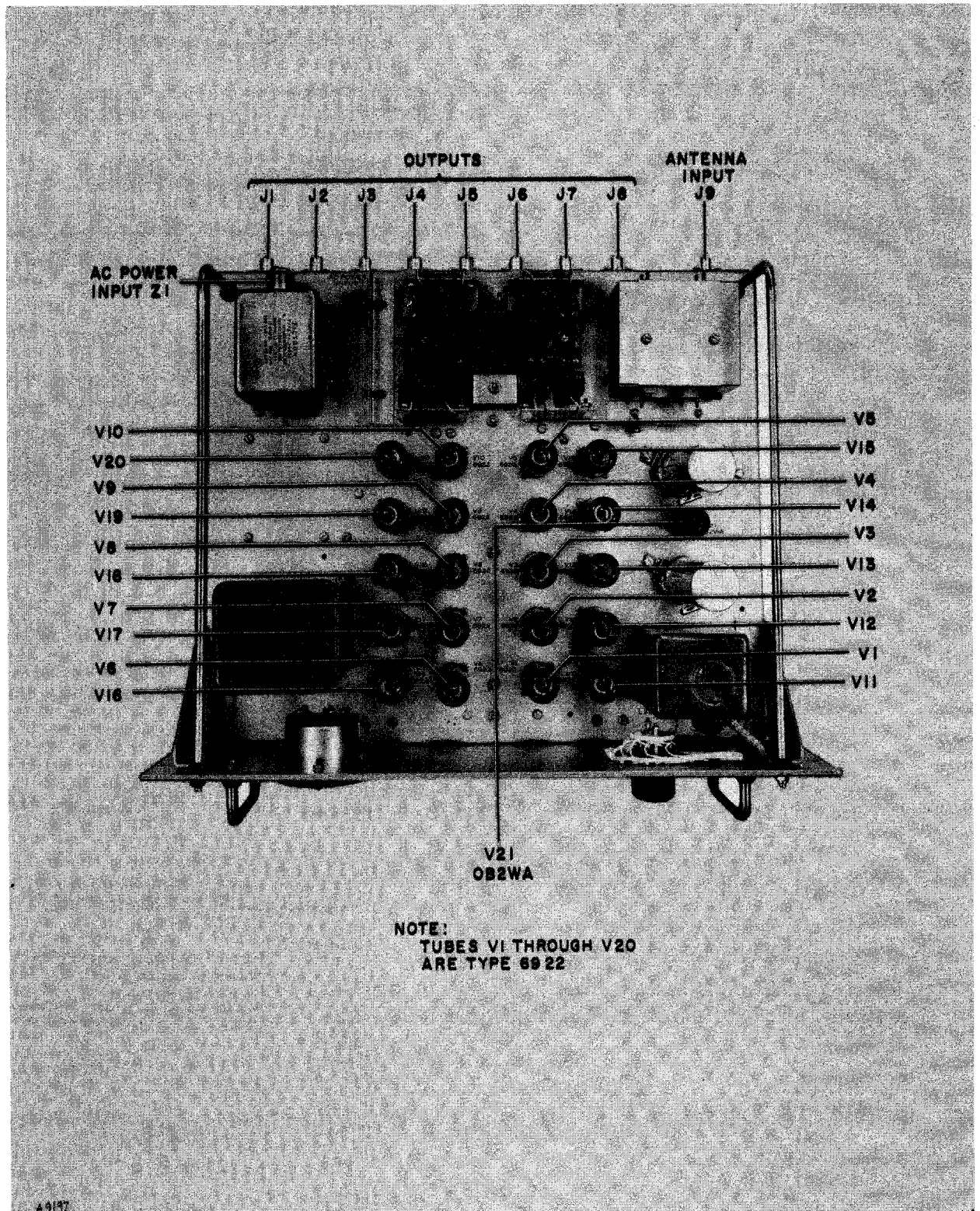
Figure 3-2. Antenna Coupler CU-872/U, Location of Tubes and Connectors
