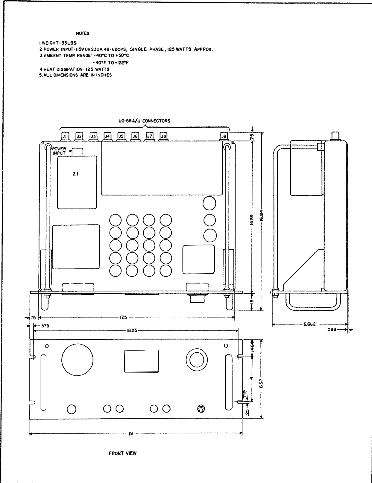
Figure 2-1. Antenna Coupler CU-872/U, Outline Drawing
