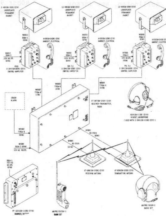
FLIGHT DECK COMMUNICATION SYSTEM AN/SRC-22(V)(XN-1)
