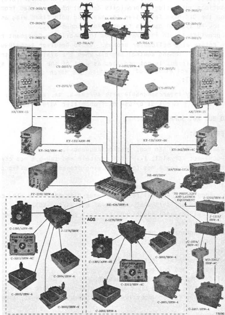
TARGET CONTROL SYSTEM AN/SRW-4G
