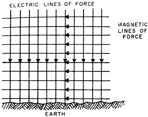
20. 241 Figure 6-1. —Cross section of a radio wave.
