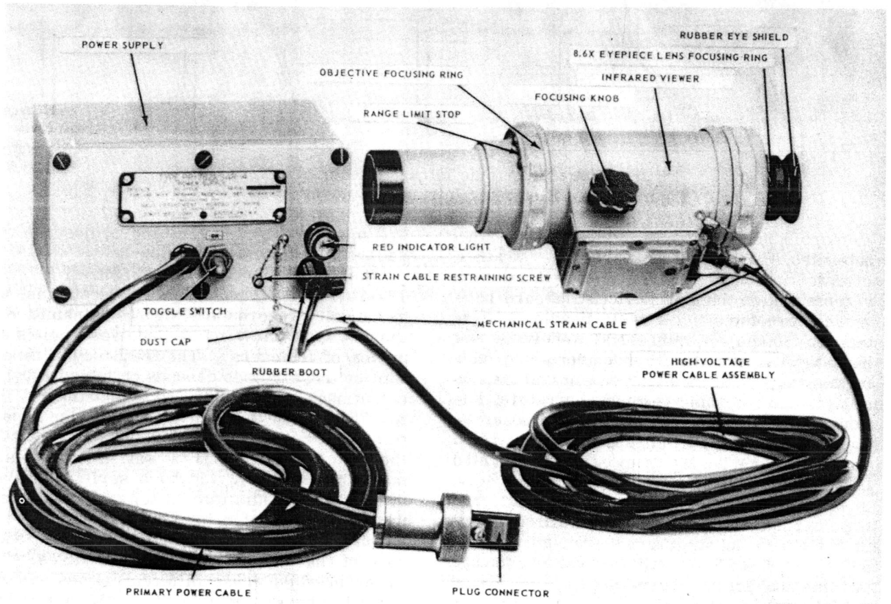
Figure 12-8.—Electronic Infrared Receiver AN/SAR-4( ).
