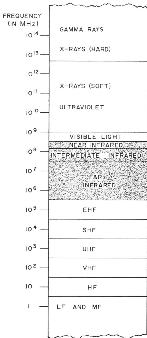
120.49 Figure 12-5.—Electromagnetic spectrum showing infrared bands.
