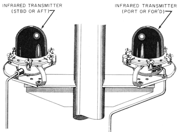
101.6 Figure 12-7.—Infrared Yardarm Beacons AN/SAT-( ).
