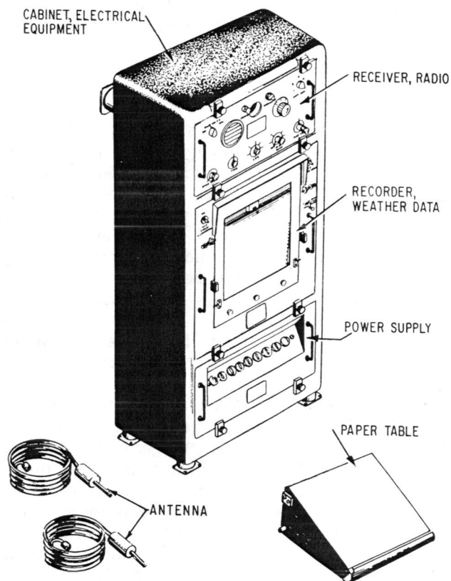
120.52 Figure 12-11.—Radiosonde Receptor AN/SMQ-1( ).
