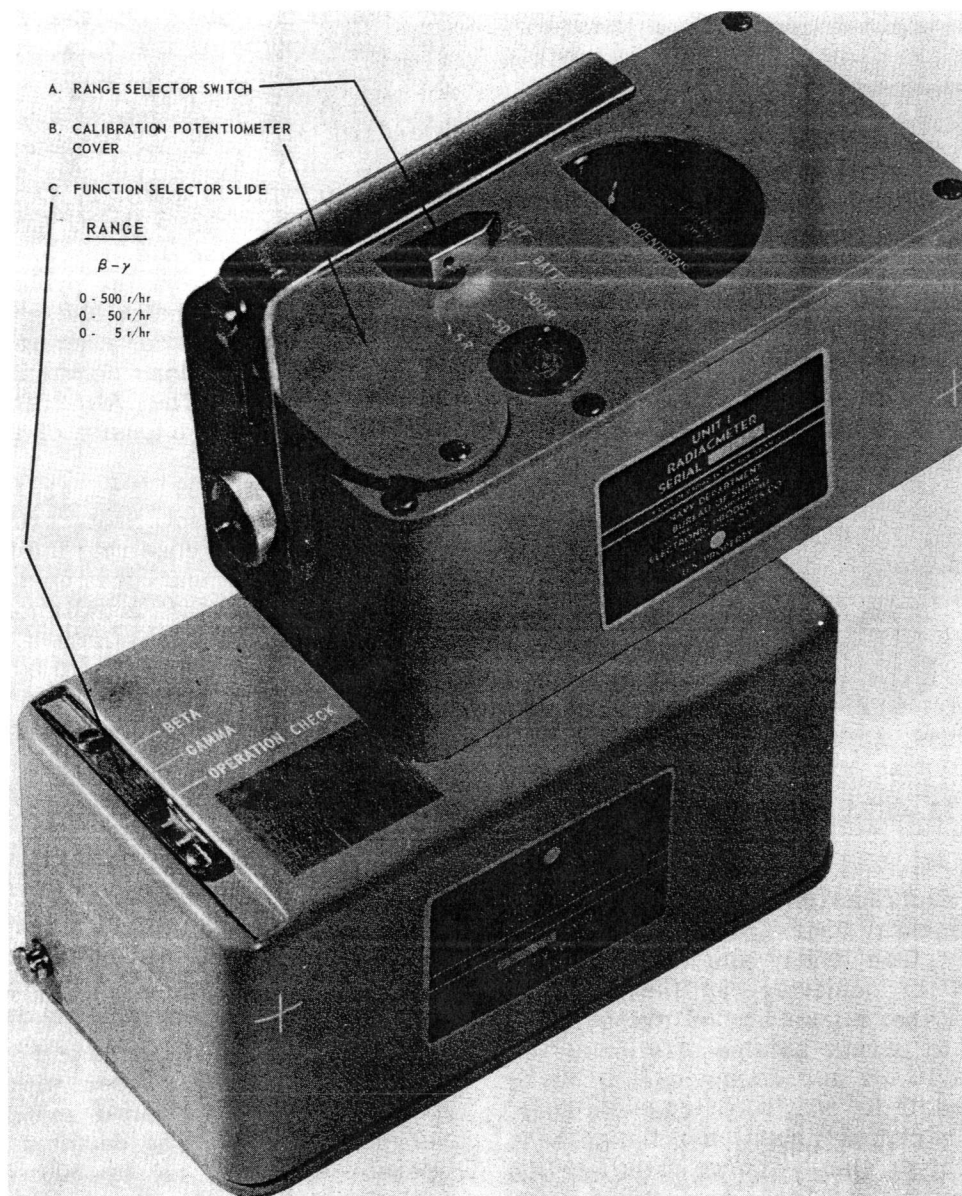
Figure 12-14.—Radiacmeter AN/PDR-43( ).
