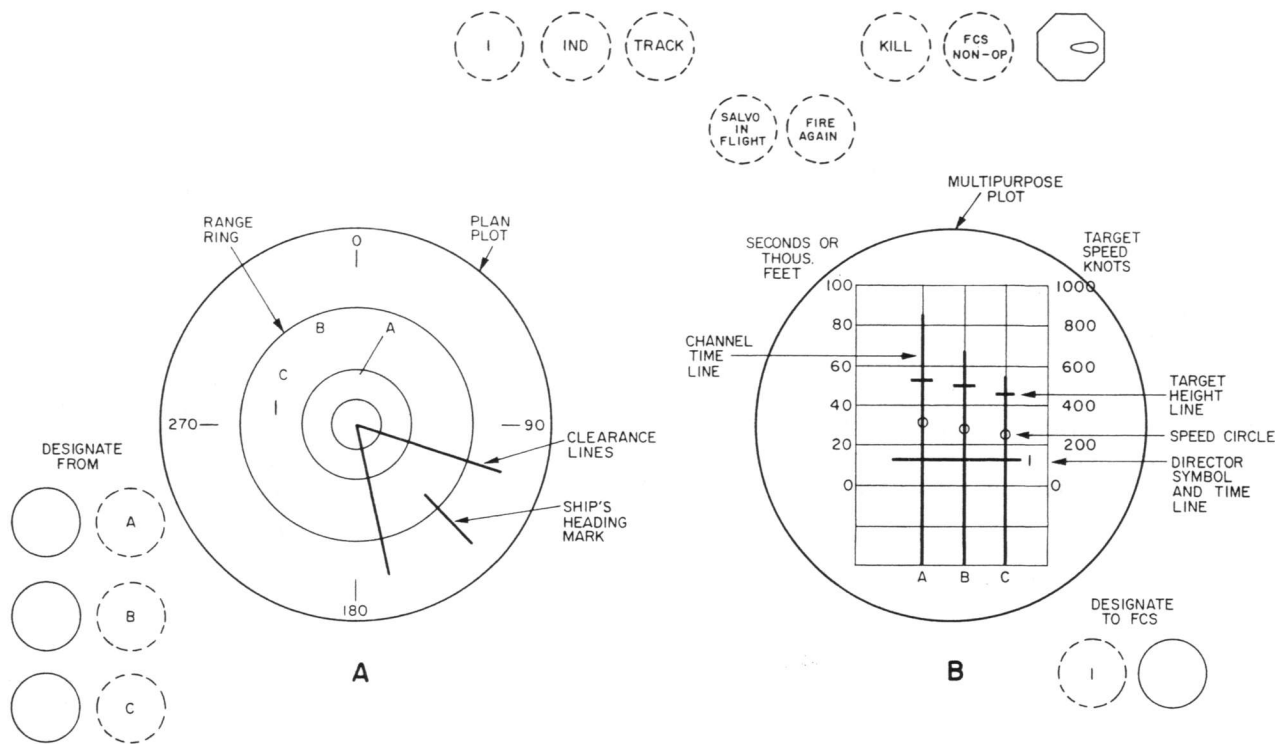
Figure 11-3.—Director assignment console display.
