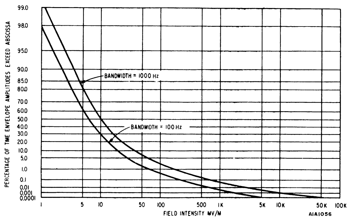
Figure 2-45. Field Intensity MV/Meter, Temperate Zone (Autumn)
