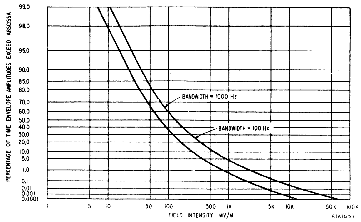
Figure 2-46. Field Intensity MV/Meter, Torrid Zone (Autumn)
