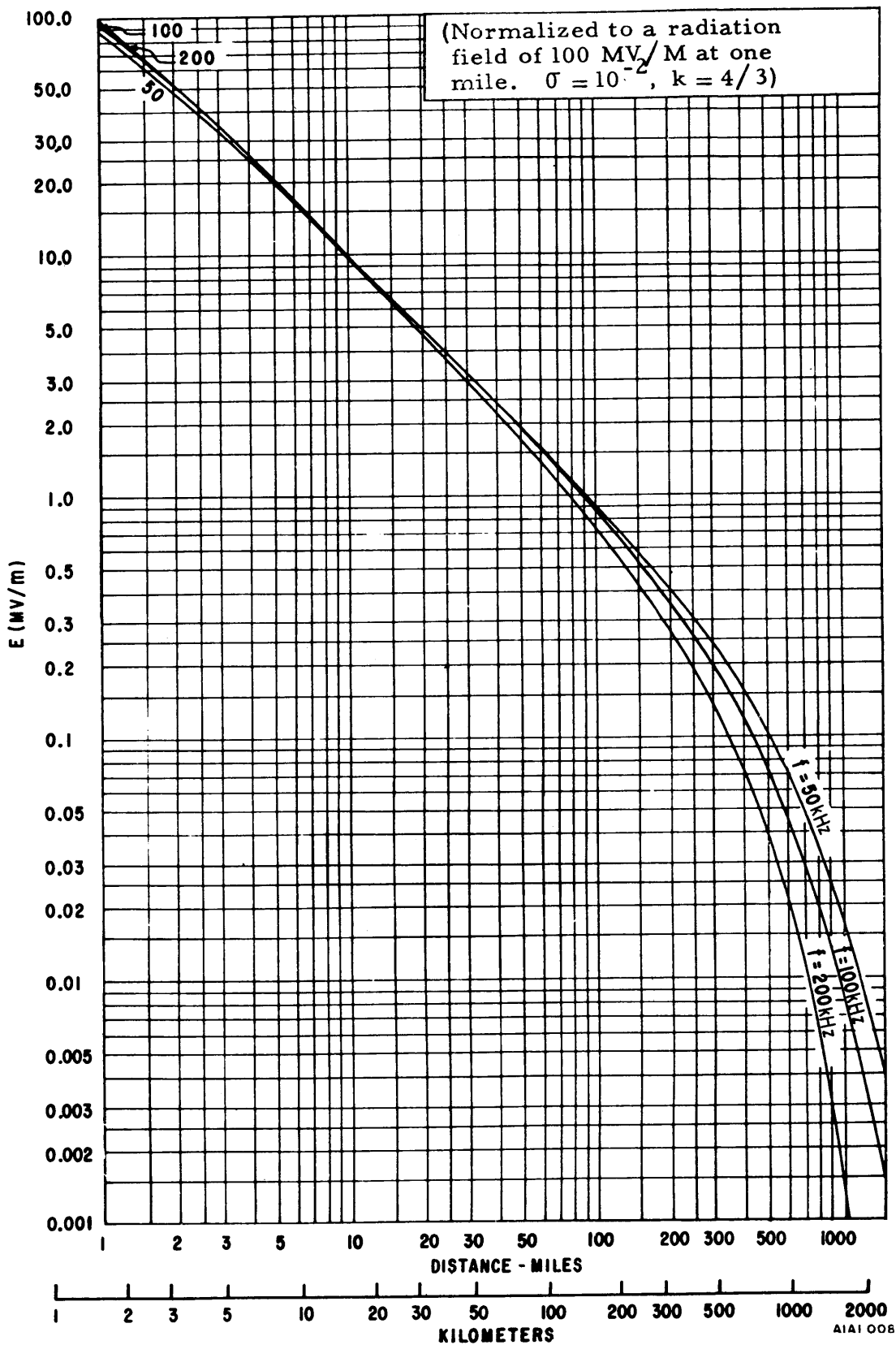
Figure 2-5. Amplitude of Ground Wave Electric Field for f = 50, 100, 200 kHz at \sigma = 10^{-2}
