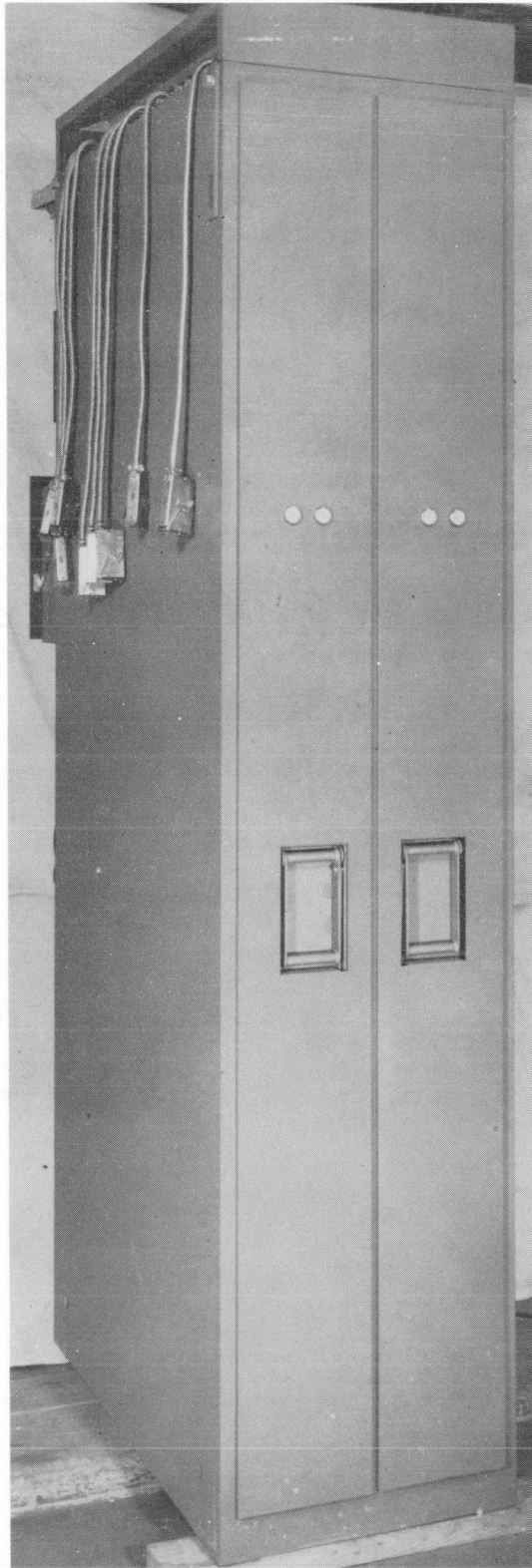
56-3587 - Teletypewriter Switching Unit 82B1 - J70121A Incoming Cabinet - Rear View - Weight 1200 Lbs. - 7-1-56
