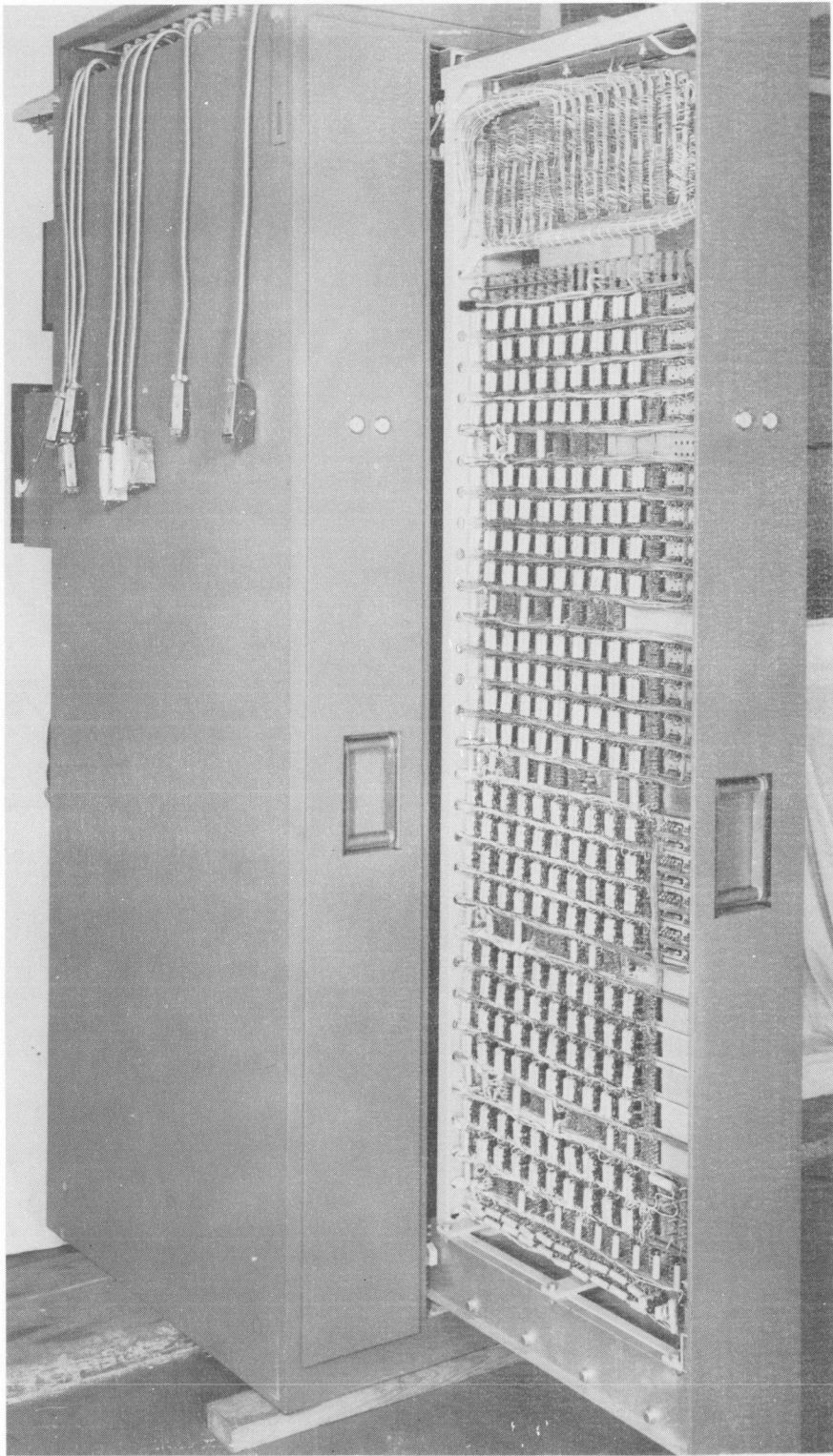
56-3589 - Teletypewriter Switching Unit 82B1 - J70121A Incoming Cabinet - Wiring Side of Relay Rack A2 - Weight 1200 Lbs. - 7-1-56
