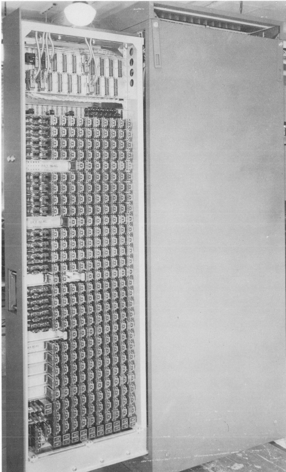
56-3585 - Teletypewriter Switching Unit 82B1 - J70121A Incoming Cabinet - Apparatus Side of Relay Rack A2 - Weight 1200 Lbs. - 7-1-56
